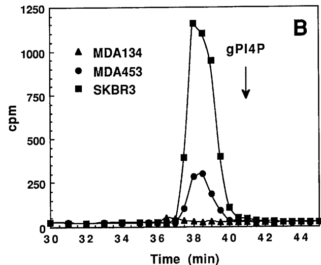
FIG. 5. Association of PI 3-kinase activity with the phosphorylated ErbB3 protein in breast cancer cells. A, 1 mg of lysate from MDA-MB-453, MDA-MB-134, or SK-BR-3 cells, or 2 mg from MDA-MB-468 cells was immunoprecipitated with anti-ErbB3 2F12. 2 mg of MDA-MB-453 cell lysate were also immunoprecipitated with normal mouse IgG as a control. The immunoprecipitates were analyzed for PI 3-kinase activity by thin layer chromatography. B, HPLC analysis of PIP products showed 32 P-labeled gPI-3-P eluting ahead of the gPI-4-P standard. Similar results were obtained in two independent experiments.
