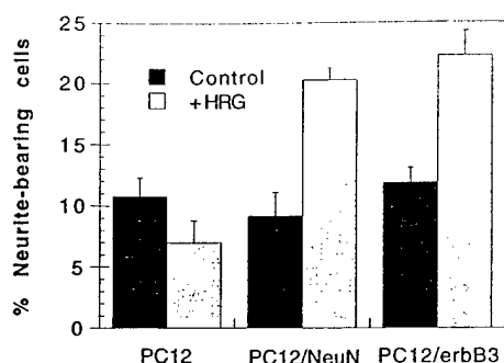
FIG. 2. Heregulin-stimulated neurite outgrowth in PC12/Erbb3 (C59.3) cells. Cells were incubated in 2 nM heregulin (HRG) in 0.5% fetal bovine serum for 3 days. Neurites were scored as described by Gamett and Cerione (9).
