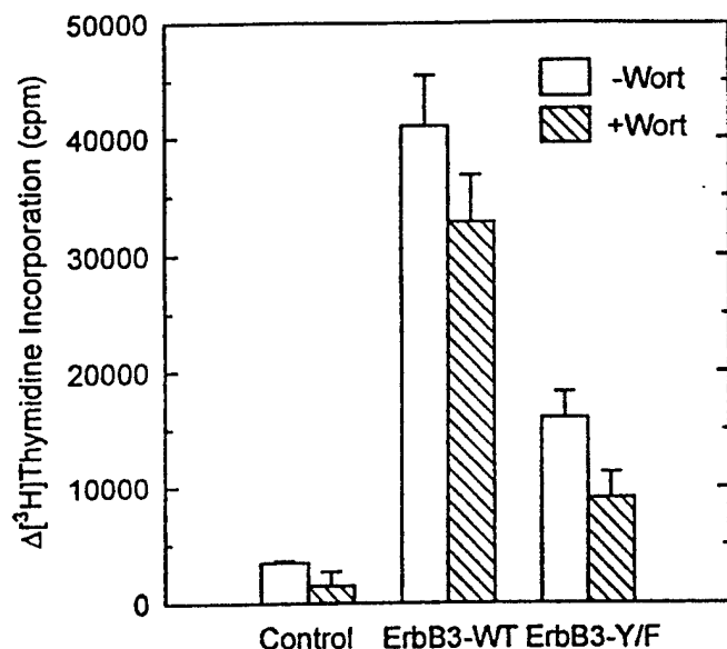
FIG. 6. Effect of inhibition of PI 3-kinase activity on heregulin-stimulated ^3\text{H} thymidine uptake. Serum-starved cells transfected with pcDNA3, pcDNA3-B3-Y/F, or pcDNA3-B3-WT expression vectors were incubated with wortmannin (Wort; 100 nM) or vehicle for 30 min prior to stimulation with either vehicle or heregulin (10 nM) for 18 h. ^3\text{H} thymidine incorporation assays were performed as indicated in Fig. 5. Heregulin-stimulated ^3\text{H} thymidine incorporation ( \Delta[^3\text{H}] thymidine incorporation) was determined in triplicate assays by subtracting basal incorporation from that stimulated by 10 nM heregulin.
