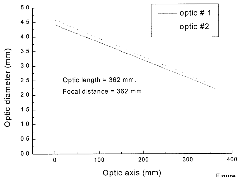
Figure 69. Profiles of two recently manufactured matched linear tapers.
