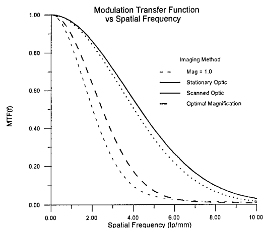
Figure 75. Modulation transfer function.
