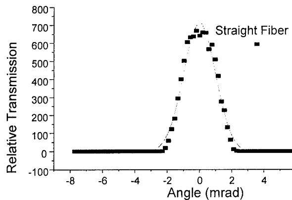
Figure 39. For an ideal fiber (with no surface defects), the divergence simulation yields a FWHM of 2.36 mrad at 8 keV.
