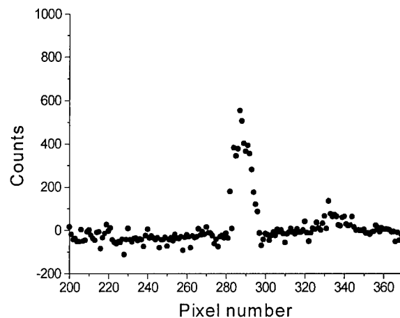
Figure 96. Background subtracted image of slit after moving detector to the left.
