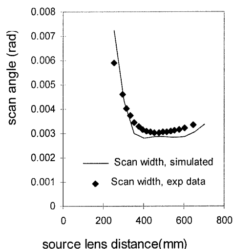
Figure 50. Source scan of tapered lens.
