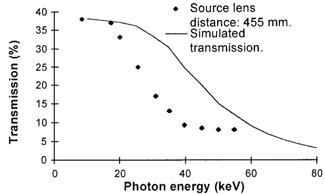
Figure 54. Transmission of whole tapered lens.
