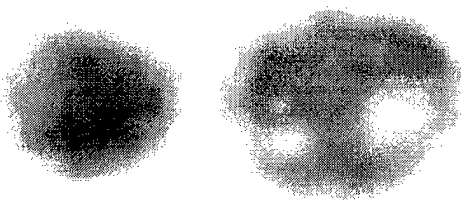
Figure 59 X-ray micrograph of pieces B (left) and A (right). A is larger since it is toward the large end of the taper, and contains the defect.
