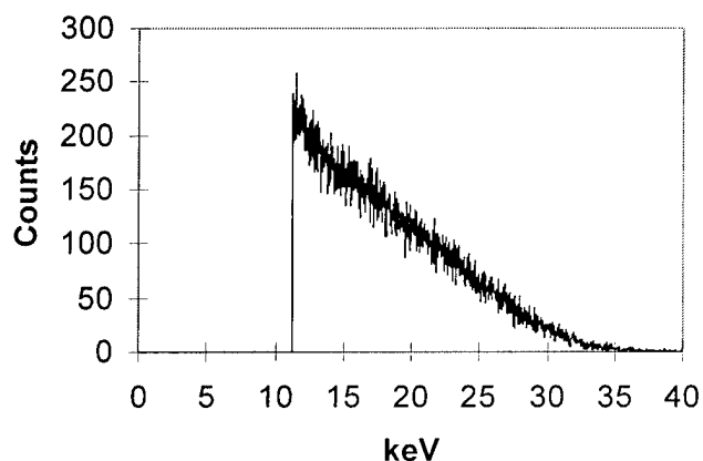
Figure 88. Spectrum of copper x-ray source, taken with single pixel CZT detector. The lower level discriminator was set at the lower end of the region of interest (ROI) marked in figure 5.
