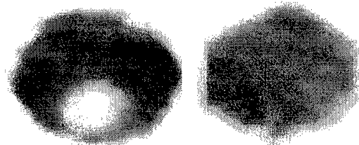
Figure 58. X-ray micrograph of next-to-last and last 5.5 cm of the optic (pieces A21, left and A22, right). A21 has a defect.
