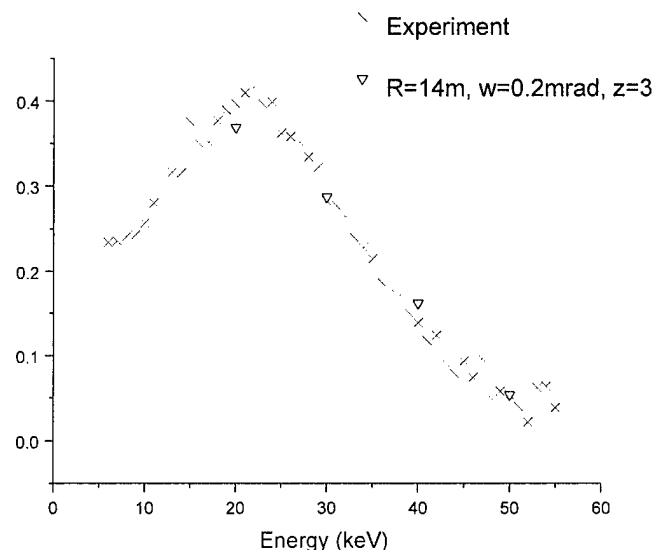
Figure 20. Transmission efficiency of 350 \mu\text{m} OD polycapillary fiber with 6 \mu\text{m} channel diameter. The fiber length is 25 cm. Simulated values are shown for 20, 30, 40, 50 keV x rays. The parameters are curvature, R ; waviness, w ; and roughness, z .
