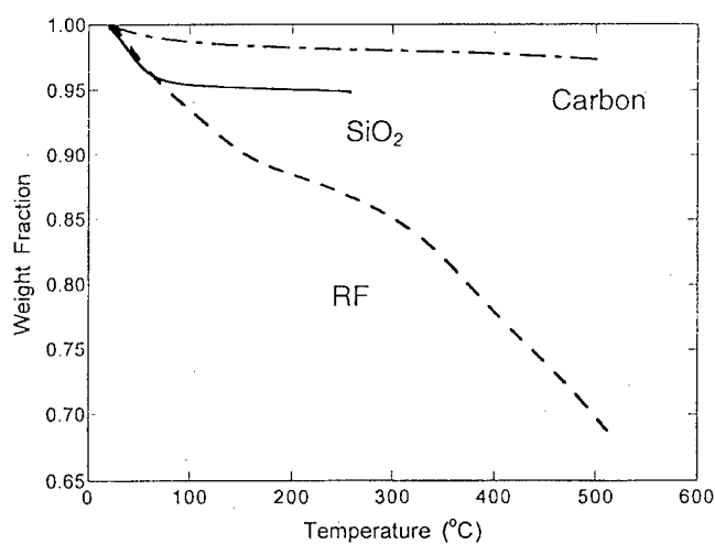
Fig. 4. TGA of aerogel substrates. The SiO 2 aerogel was heated previously to 500 °C, the RF aerogel was unheated, and the carbon aerogel was pyrolyzed at 1015 °C.
