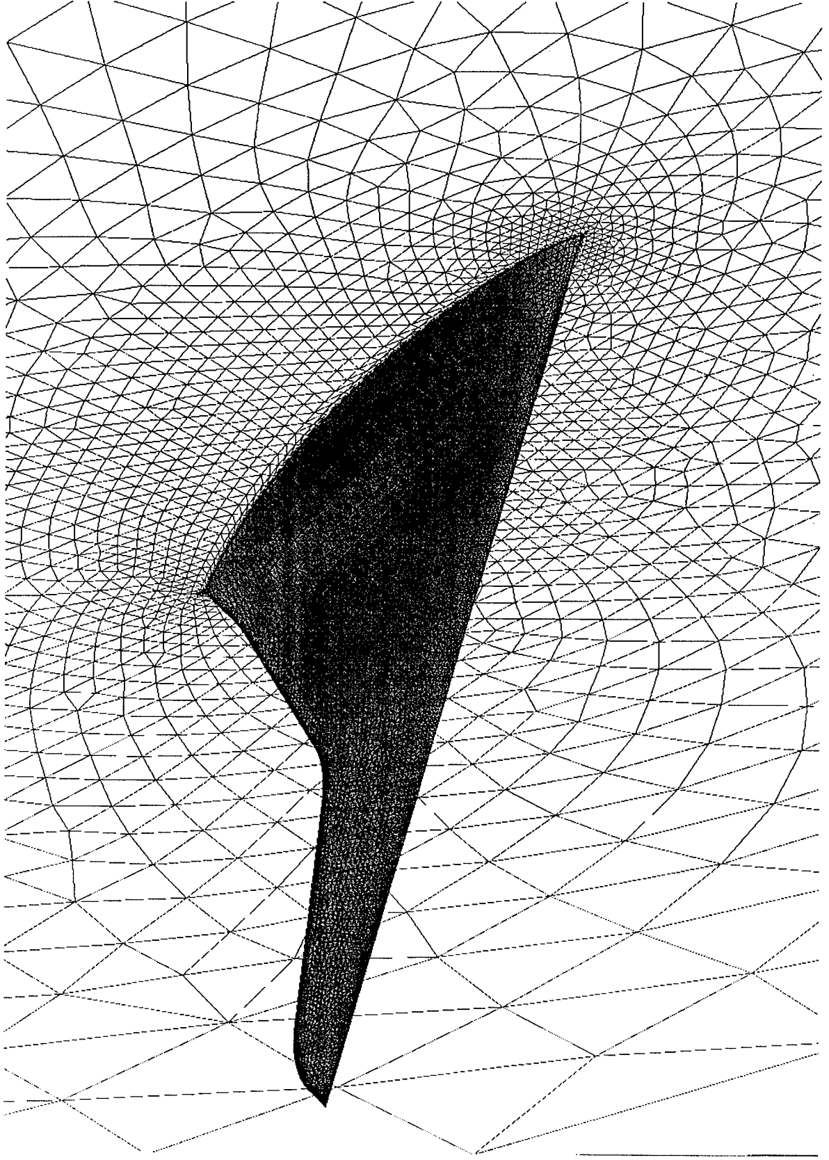
Fig. 7- CFD Grid
