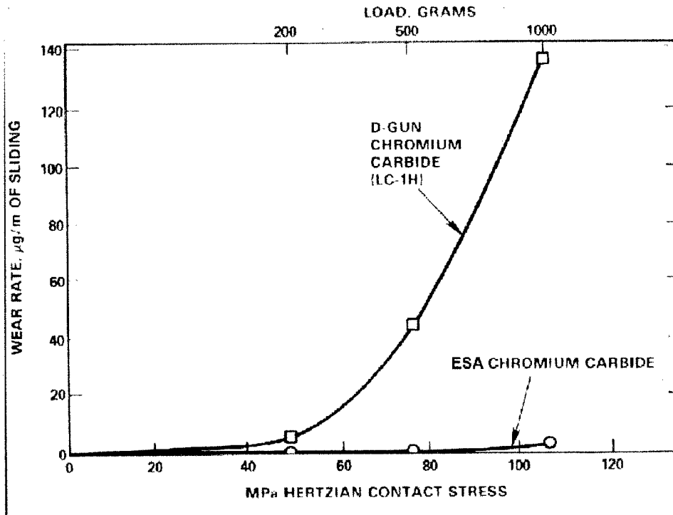
Figure 6. Wear data comparing chromium carbide (on stainless steel) coatings produced by ESA vs. detonation gun.
