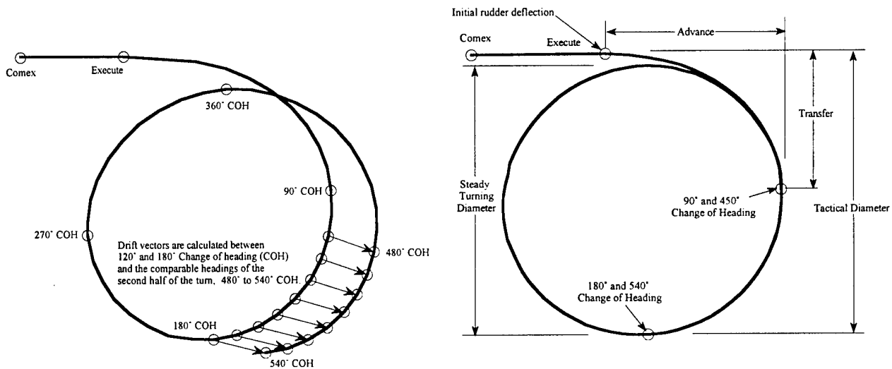
Fig. 8. Comparison of the paths for uncorrected and corrected conventional tactical turns.
