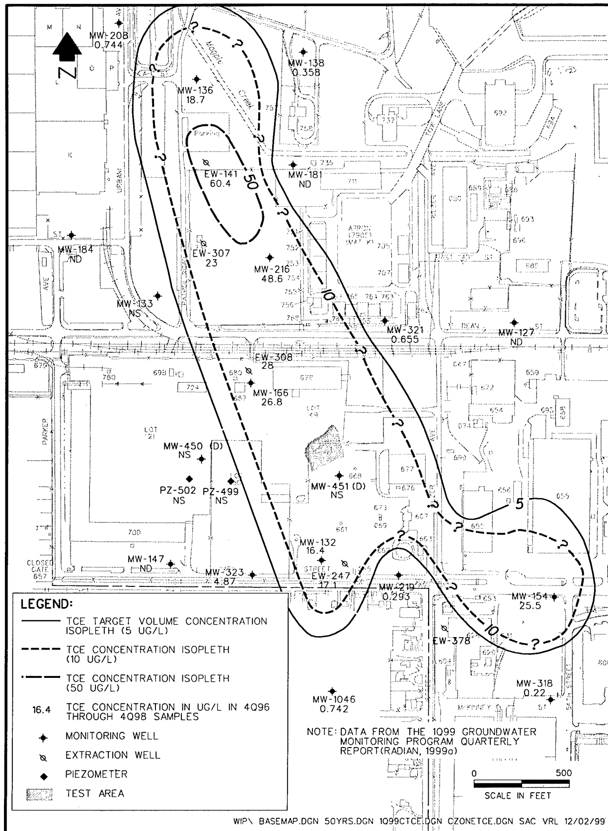
Figure 2-10. TCE Groundwater Contamination in the C Monitoring Zone at the Test Area , McClellan AFB
