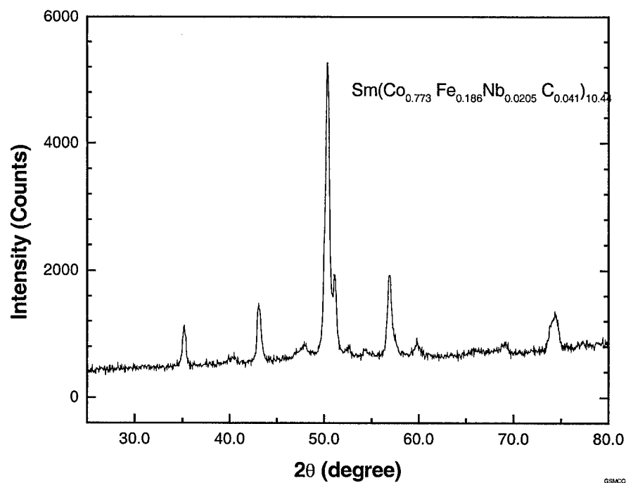
Figure 3.58. XRD patterns of as-spun ribbons for Sm(Co 0.773 Fe 0.186 Nb 0.0205 C 0.041 ) 10.44 .
