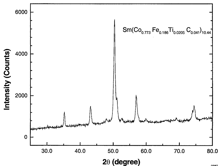
Figure 3.57. XRD patterns of as-spun ribbons for Sm(Co 0.773 Fe 0.186 Ti 0.0205 C 0.041 ) 10.44 .
