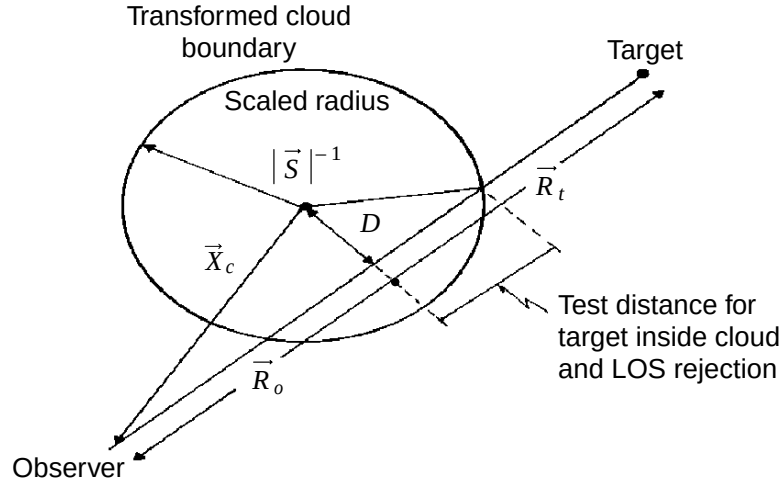
Figure A-3. Scaled parameters for path integration and cloud rejection.
