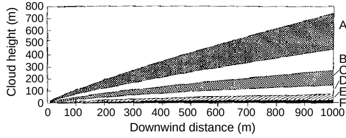
Figure A-7. Cloud diffusive height ( 2.15\sigma ) for different Pasquill categories.
