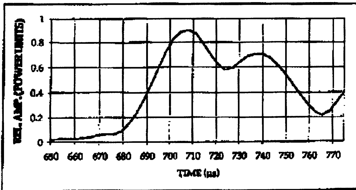
Figure 31 Transmitted signal through a package of meat indicates a good vacuum seal
