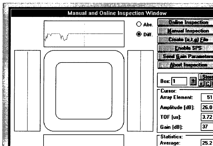
Figure 27 ALCAN Ultrasonic Scan of Contaminated Seal
