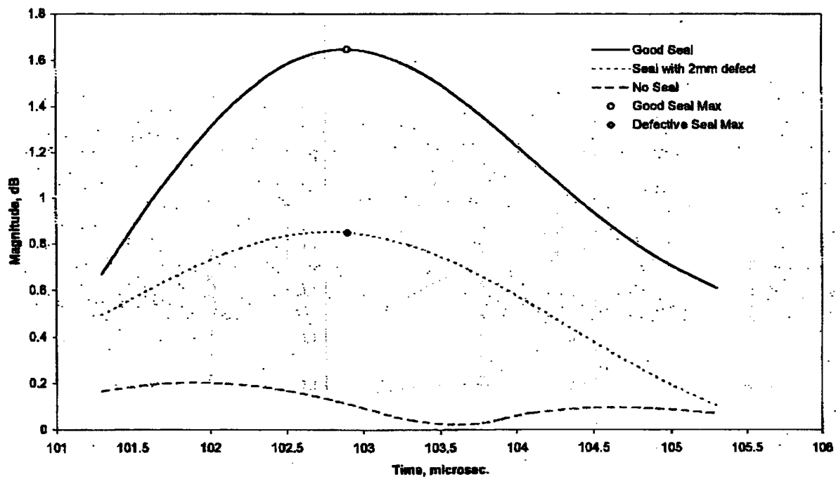
Figure 33 Air-Coupled Ultrasonic Seal Test
