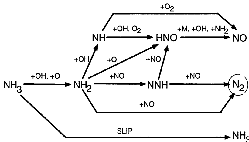
Figure 2.3: Reaction Path Diagram for the Thermal \text{DeNO}_x Process (Miller and Bowman, 1989)
