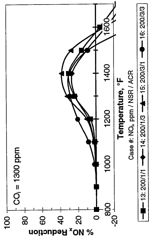
Figure 5.12: Effective NO x Reduction using Cyanuric Acid with Hydrogen Additive.
