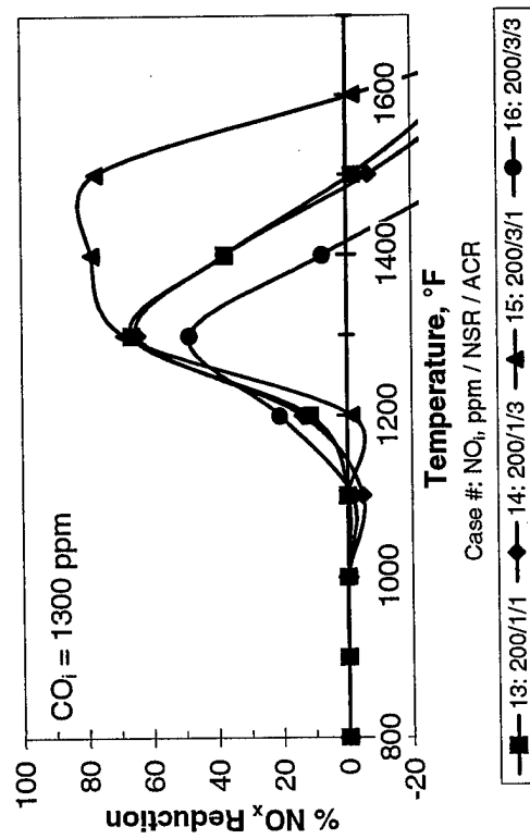
Figure 5.11: Effective NO x Reduction using Ammonia with Hydrogen Additive.
