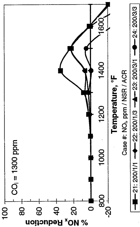
Figure 5.16: Effective NO x Reduction using Cyanuric Acid with Methane Additive.
