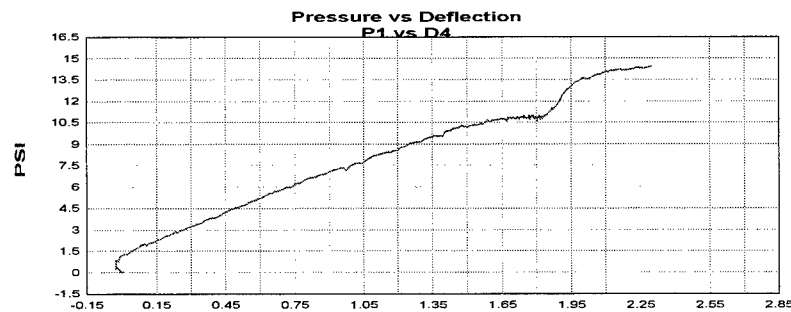
Figure A.35 Group B test 10 P1 pressure versus D4 deflection plot.
