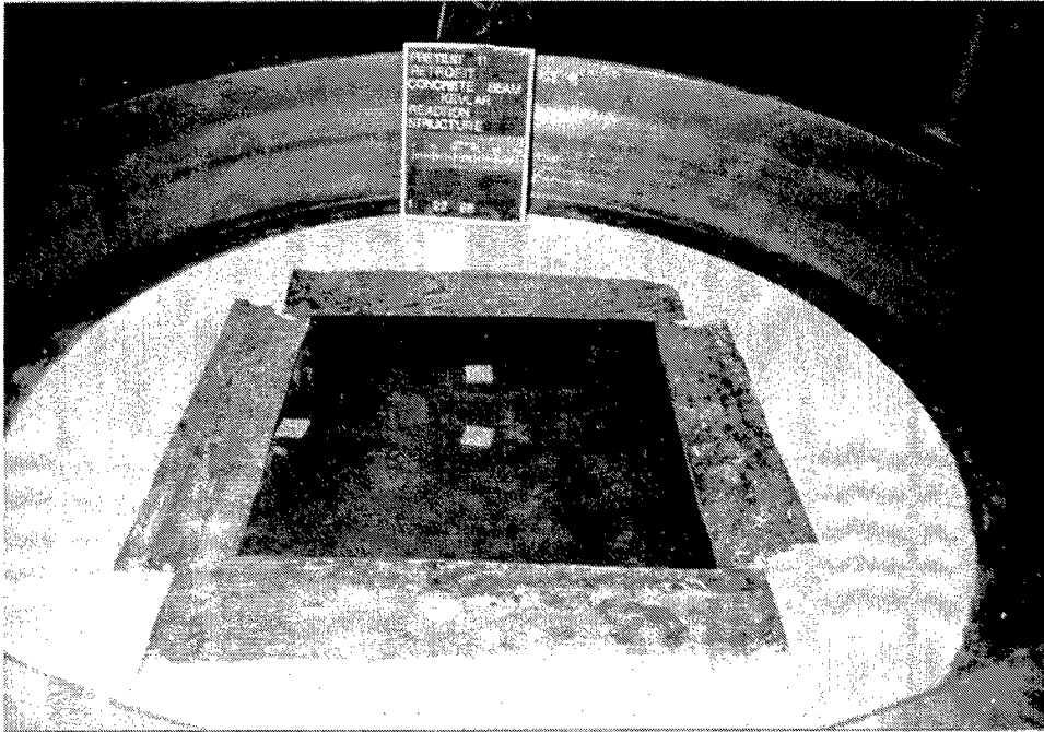
Figure 2.13. The sand is in place with strips of neoprene
