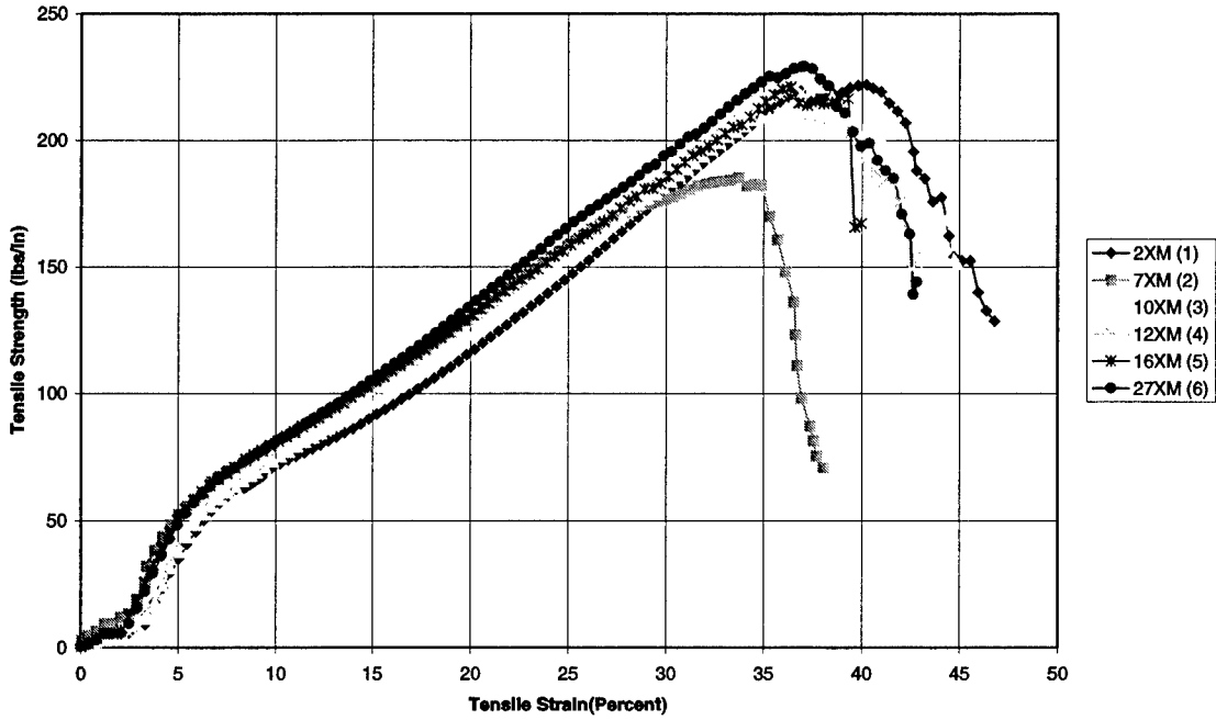
Figure C.10 ASTM 4595 Group B GG 24 Cross Direction.
