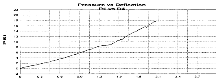
Figure A.8 Group A test 2 P1 pressure versus D4 deflection plot.
