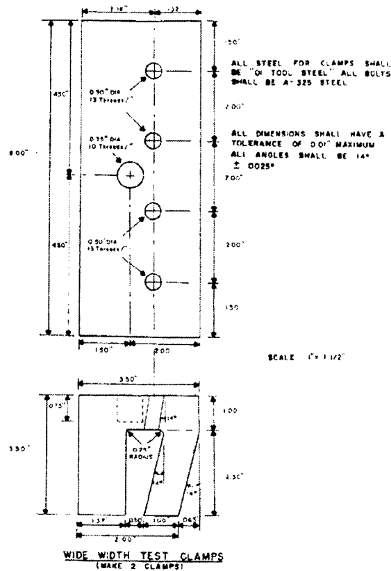
FIG. 1 Wide Width Test Clamps
