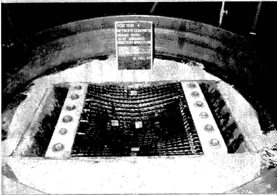
Figure 3.8. Group B test 4 posttest
