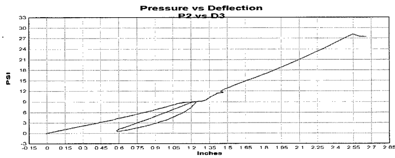
Figure A.14 Group B test 4 P2 pressure versus D3 deflection plot.
