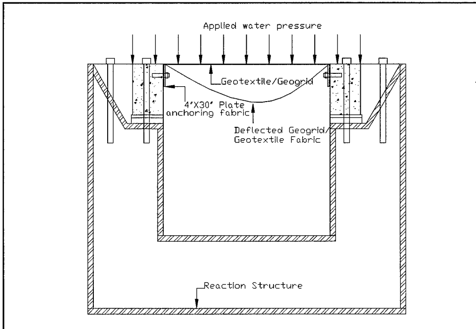
Figure 2.1. Experimental setup that models prototype system
