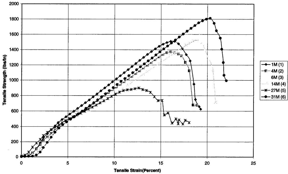
Figure C.13 ASTM 4595 Group A COM GT 500 Machine Direction.
