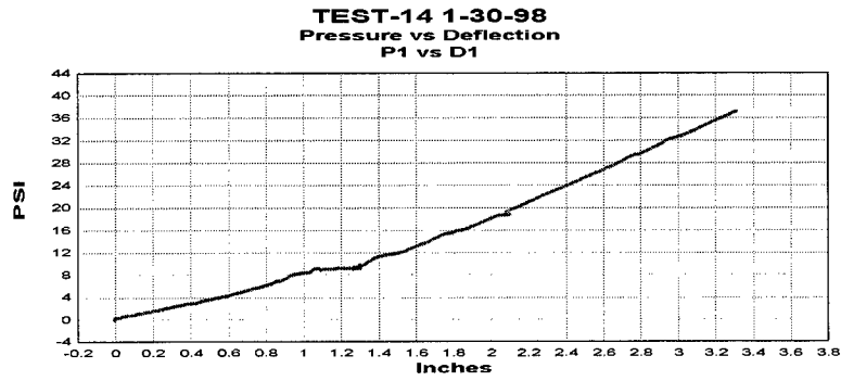
Figure A.47 Group A test 14 P1 pressure versus D1 deflection plot.
