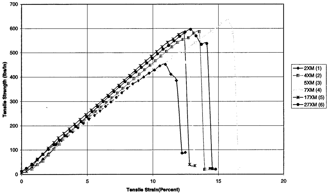
Figure C.6 ASTM 4595 Group A GT 1715 Cross Direction.
