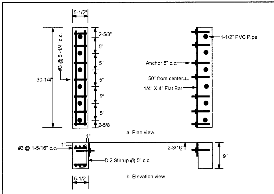
Figure 2.6. Connection details for geogrid/geotextile
