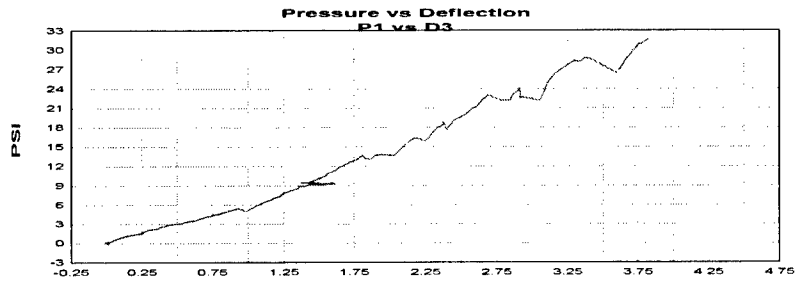
Figure A.25 Group A test 7 P1 pressure versus D3 deflection plot.
