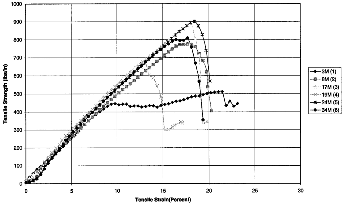
Figure C.3 ASTM 4595 Group A GT 800 Machine Direction.
