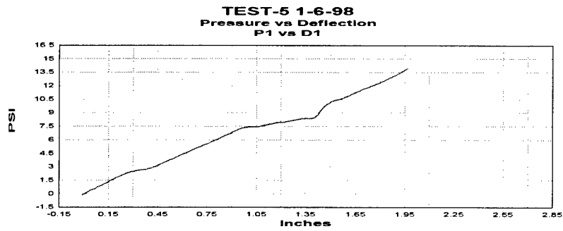
Figure A.16 Group B test 5 P1 pressure versus D1 deflection plot.
