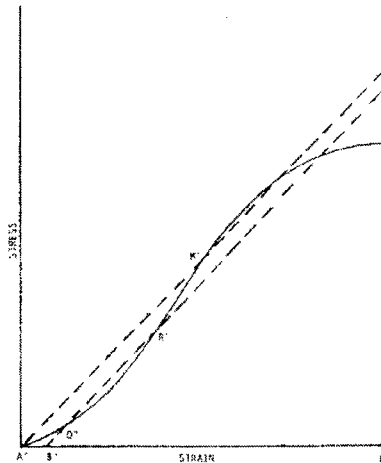
FIG. X3.1 Construction Line for Secant Modulus
