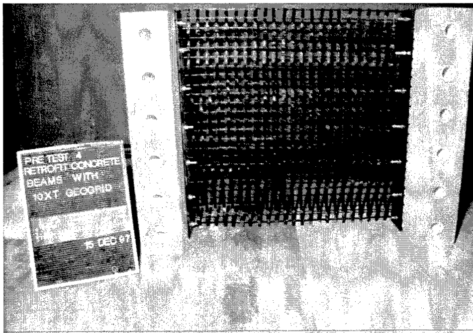
Figure 2.8. Typical pretest view of the geogrid connection
