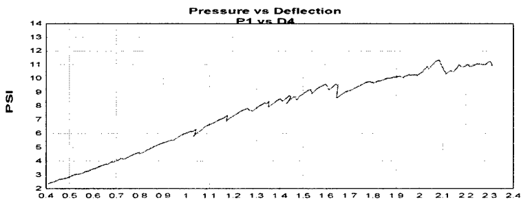
Figure A.4 Group A test 1 P1 pressure versus D4 deflection plot.
