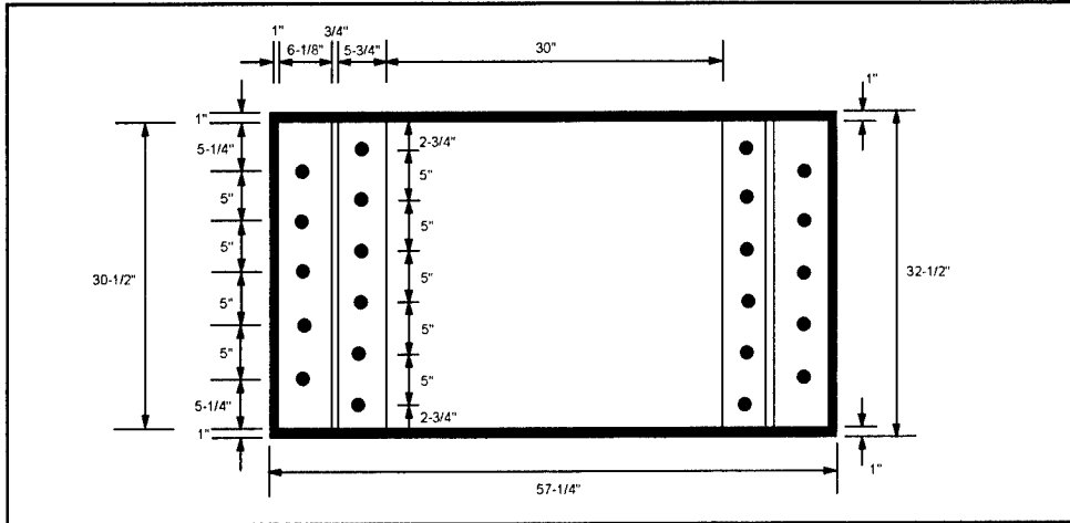
Figure 2.3. Reaction Structure Plan View
