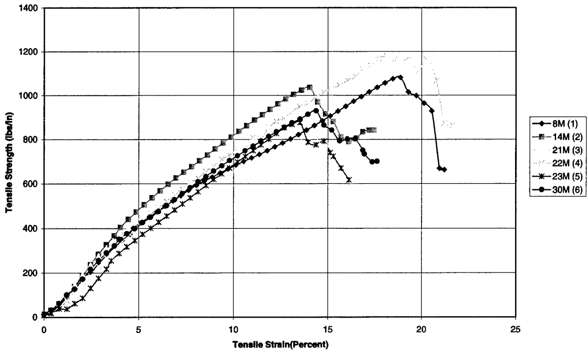
Figure C.5 ASTM 4595 Group A GT 1715 Machine Direction.
