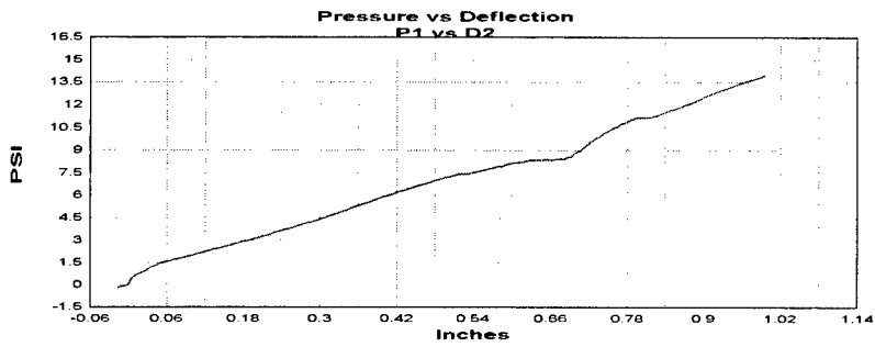
Figure A.17 Group B test 5 P1 pressure versus D2 deflection plot.
