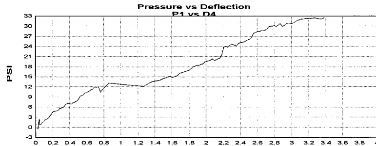
Figure A.42 Group A test 12 P1 pressure versus D4 deflection plot.
