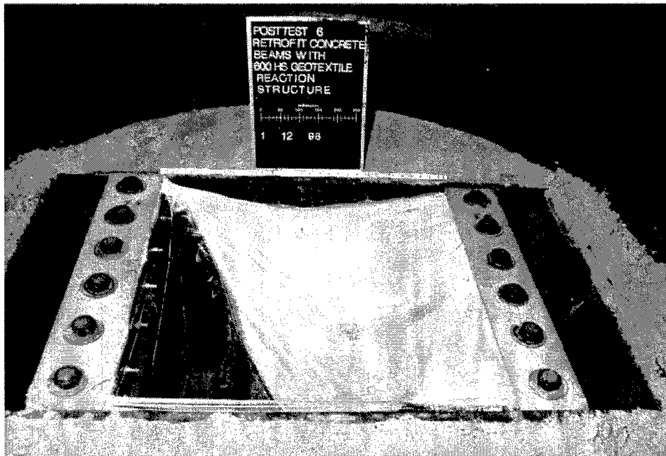
Figure 3.12. Group A test 6 posttest
