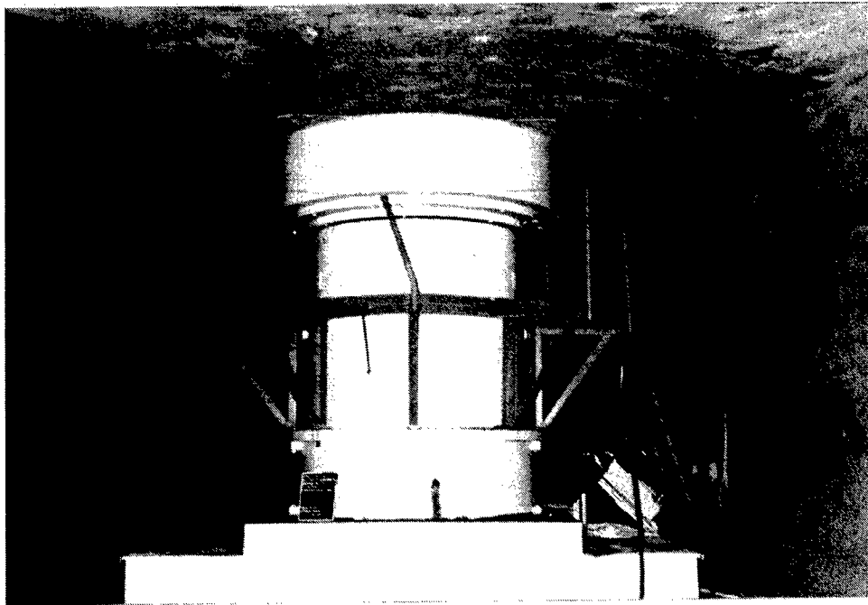
Figure 2.16. The test chamber was cabled into position
