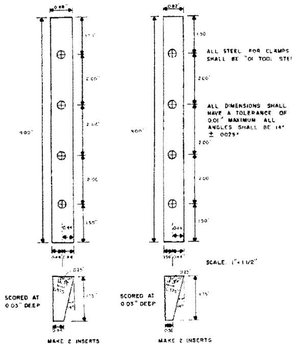
FIG. 2 Inserts for Wide Width Clamps
