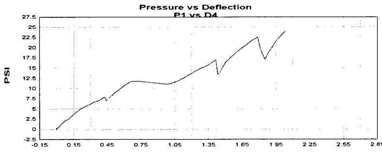
Figure A.32 Group A test 9 P1 pressure versus D4 deflection plot.
