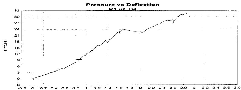
Figure A.26 Group A test 7 P1 pressure versus D4 deflection plot.
