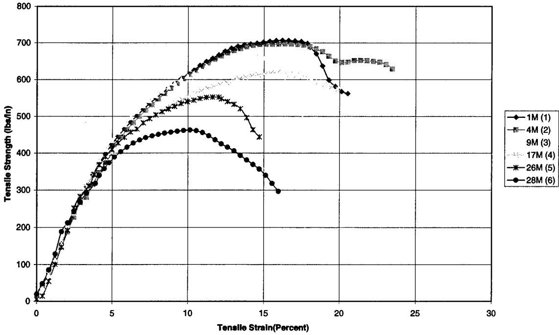
Figure C.9 ASTM 4595 Group B GG 24 Machine Direction.
