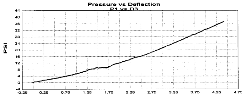
Figure A.49 Group A test 14 P1 pressure versus D3 deflection plot.
