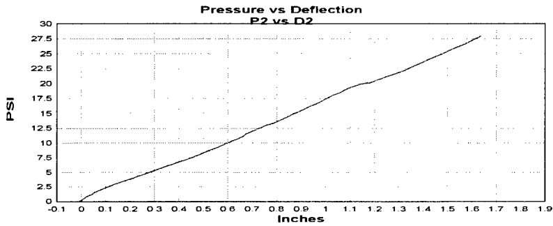
Figure A.44 Group A test 13 P2 pressure versus D2 deflection plot.
