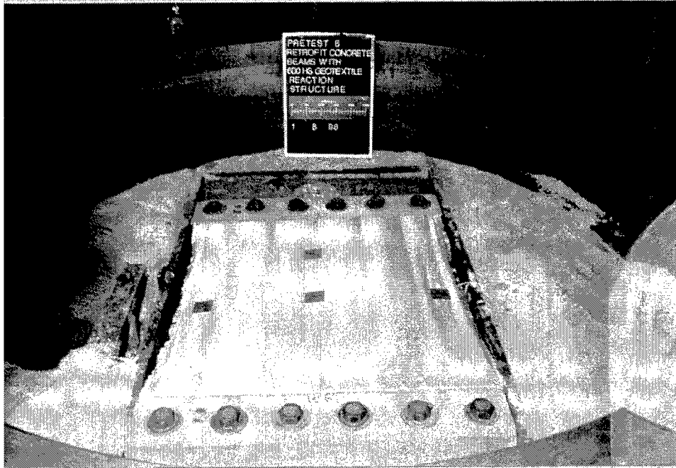
Figure 3.11. Group A test 6 pretest
