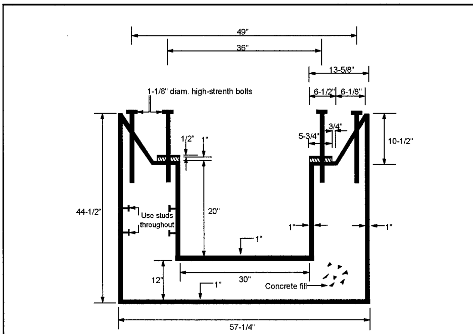
Figure 2.2. Reaction Structure Cross-Section View
