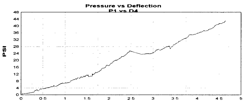
Figure A.38 Group A test 11 P1 pressure versus D4 deflection plot.
