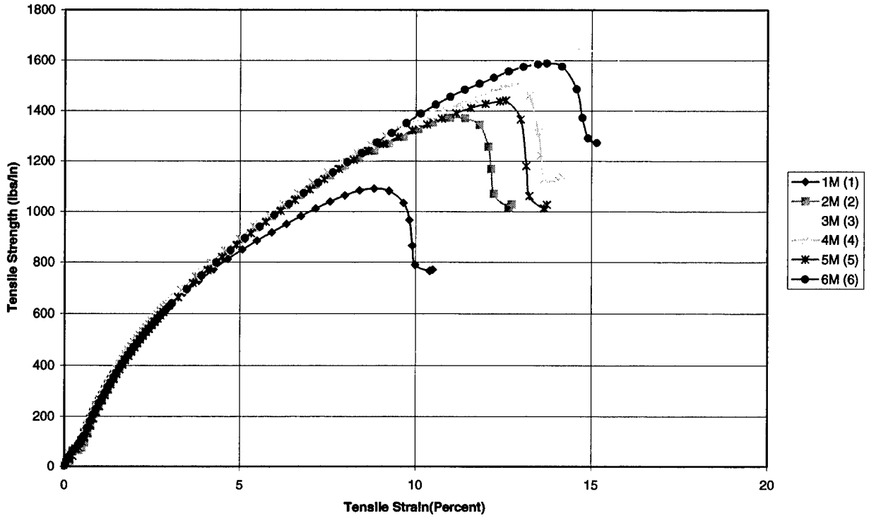
Figure C.17 ASTM 4595 Group B GG 1500 Machine Direction.
