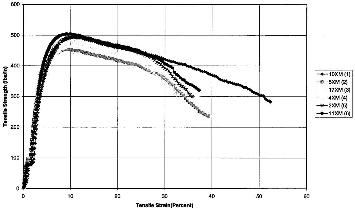
Figure C.18 ASTM 4595 Group B GG 1500 Cross Direction.
