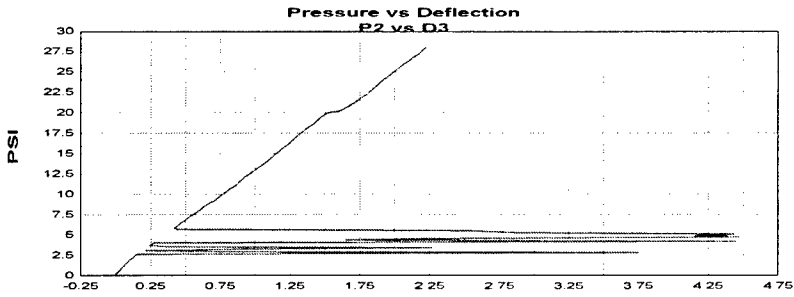
Figure A.45 Group A test 13 P2 pressure versus D3 deflection plot.
