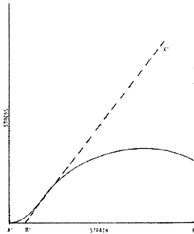
FIG. X2.1 Material with No Hookean Region
