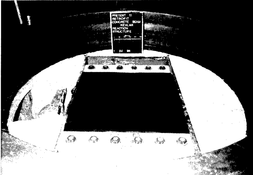
Figure 3.20. Group A test 11 pretest
