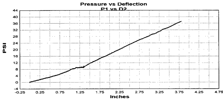
Figure A.48 Group A test 14 P1 pressure versus D2 deflection plot.
