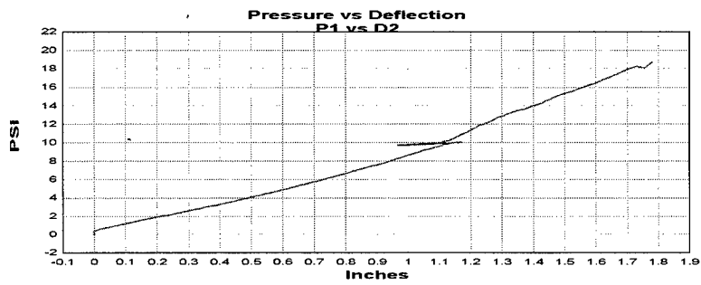
Figure A.21 Group A test 6 P1 pressure versus D2 deflection plot.
