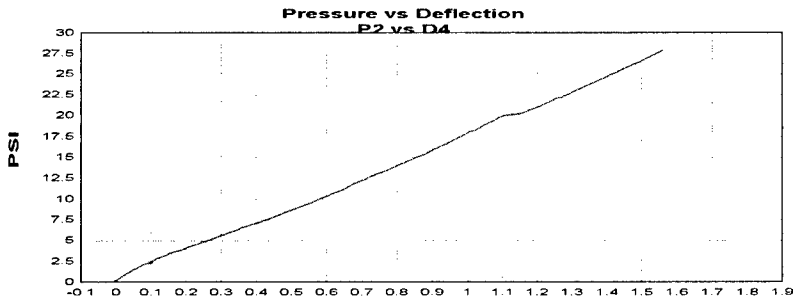
Figure A.46 Group A test 13 P2 pressure versus D4 deflection plot.
