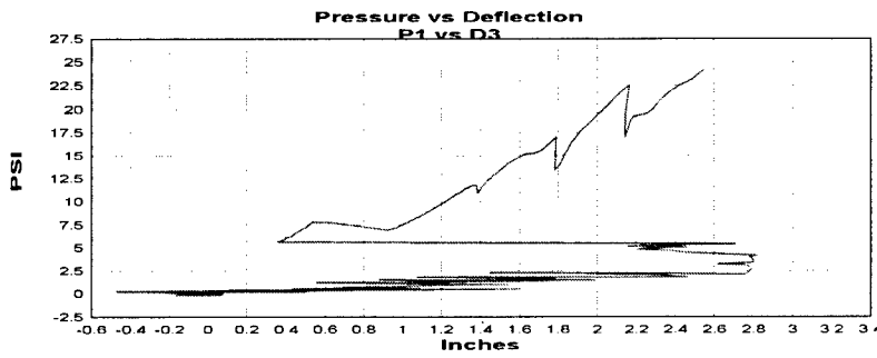
Figure A.31 Group A test 9 P1 pressure versus D3 deflection plot.
