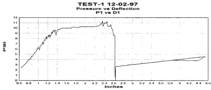
Figure A.1 Group A test 1 P1 pressure versus D1 deflection plot.
