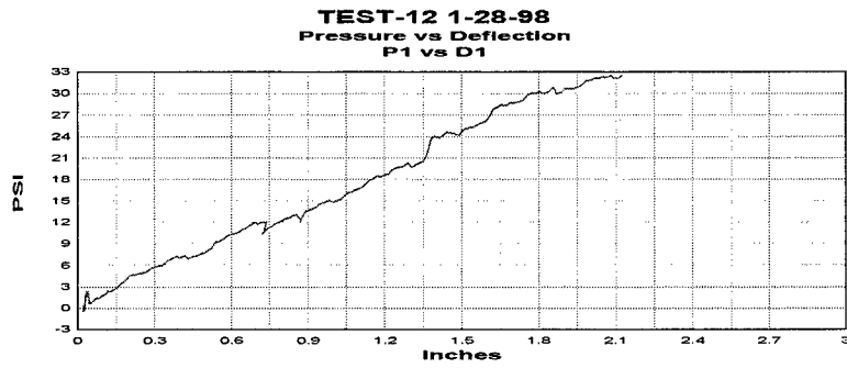
Figure A.39 Group A test 12 P1 pressure versus D1 deflection plot.
