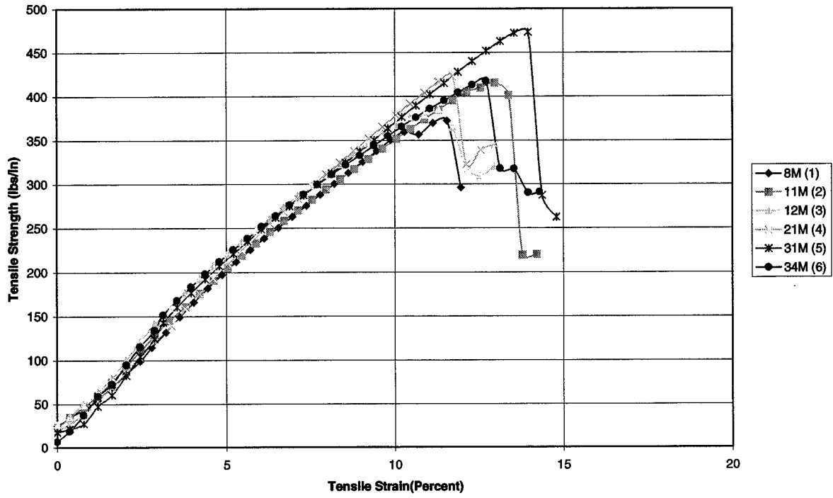
Figure C.7 ASTM 4595 Group B GG 10 Machine Direction.
