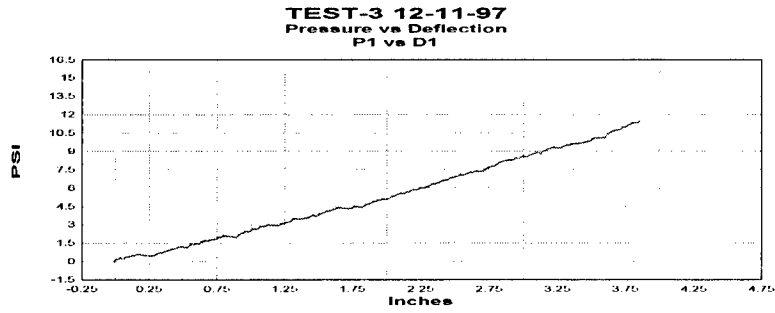
Figure A.9 Group A test 3 P1 pressure versus D1 deflection plot.
