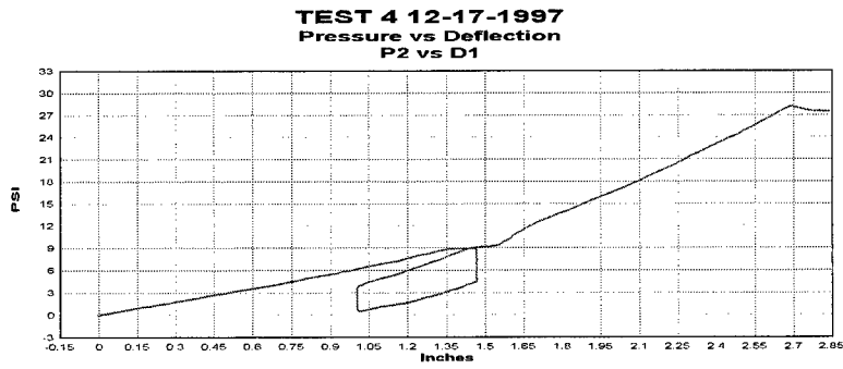
Figure A.13 Group B test 4 P2 pressure versus D1 deflection plot.
