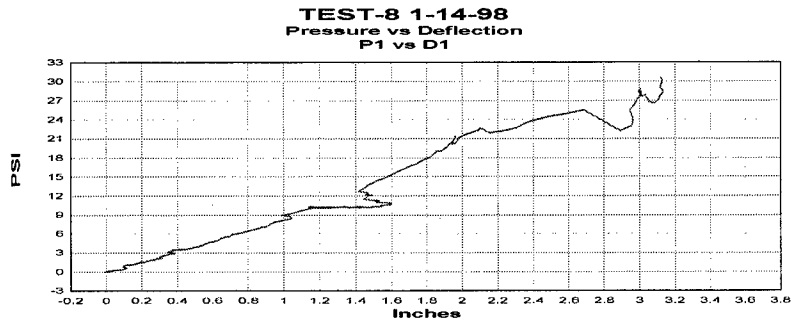
Figure A.27 Group A test 8 P1 pressure versus D1 deflection plot.
