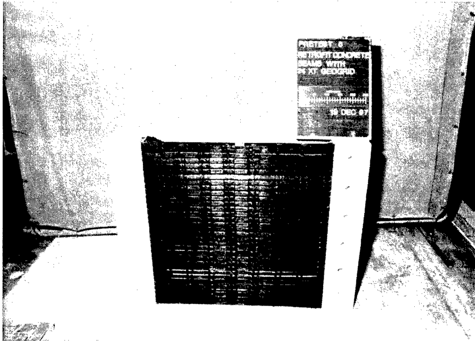
Figure 3.9. Group B test 5 pretest
