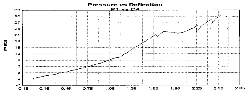
Figure A.29 Group A test 8 P1 pressure versus D4 deflection plot.
