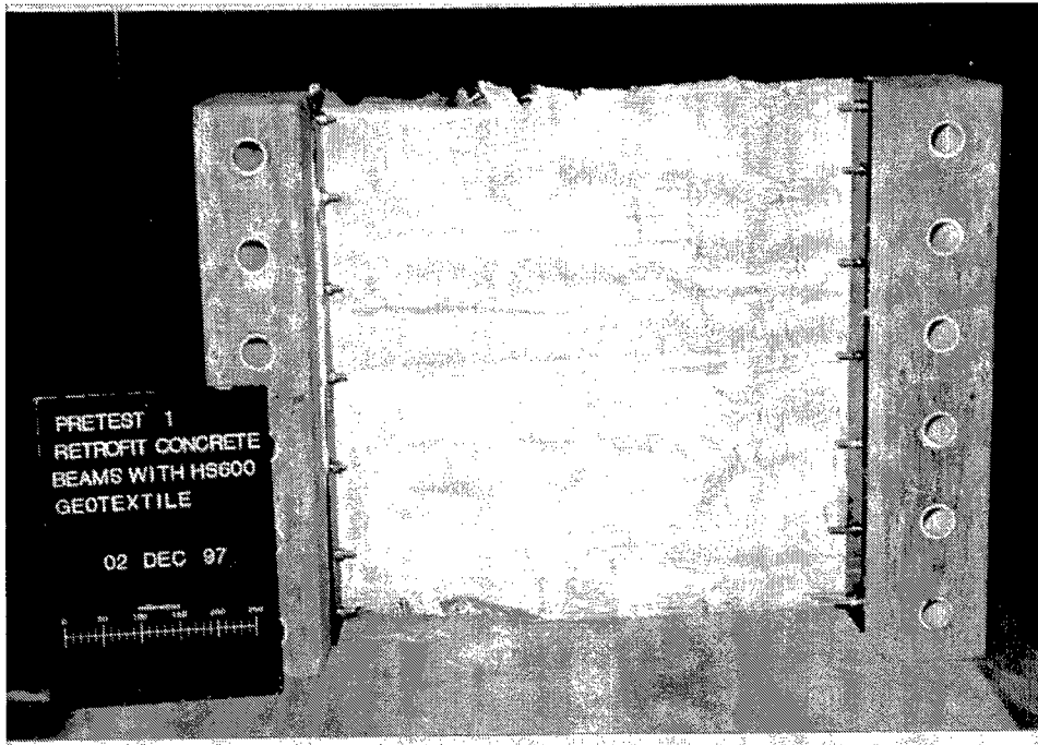
Figure 2.7. Typical pretest view of geotextile connection
