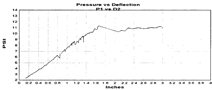
Figure A.2 Group A test 1 P1 pressure versus D2 deflection plot.
