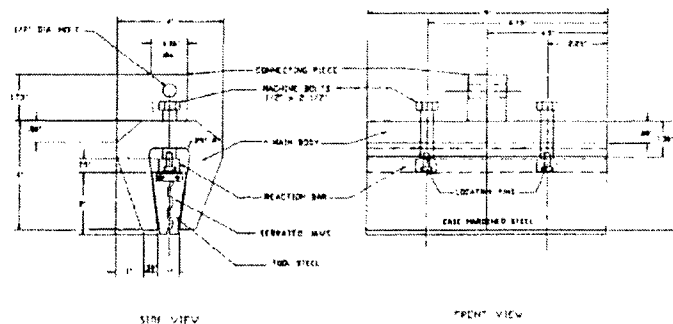
FIG. 4 Sanders Clamp
