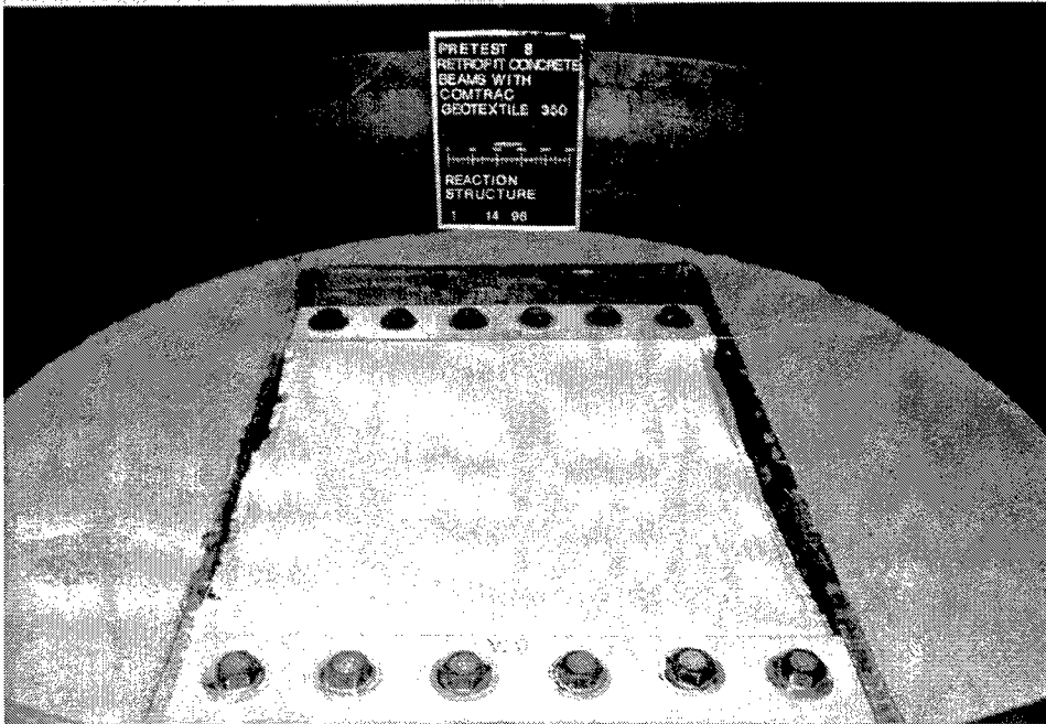
Figure 3.15. Group A test 8 pretest
