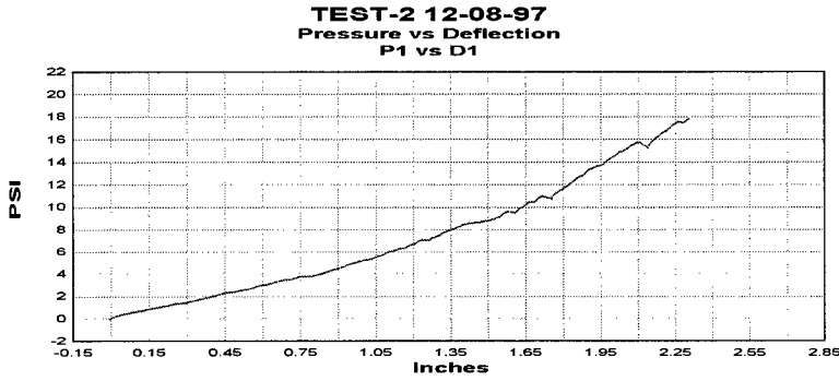
Figure A.5 Group A test 2 P1 pressure versus D1 deflection plot.
