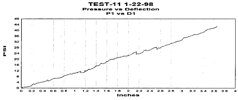
Figure A.36 Group A test 11 P1 pressure versus D1 deflection plot.
