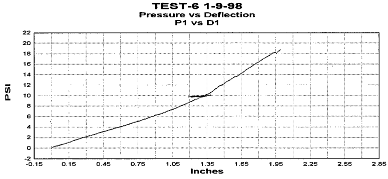
Figure A.20 Group A test 6 P1 pressure versus D1 deflection plot.
