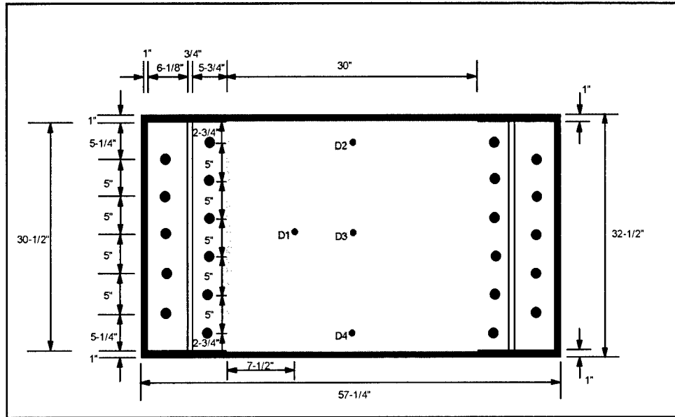
Figure 2.9. Instrumentation gage layout
