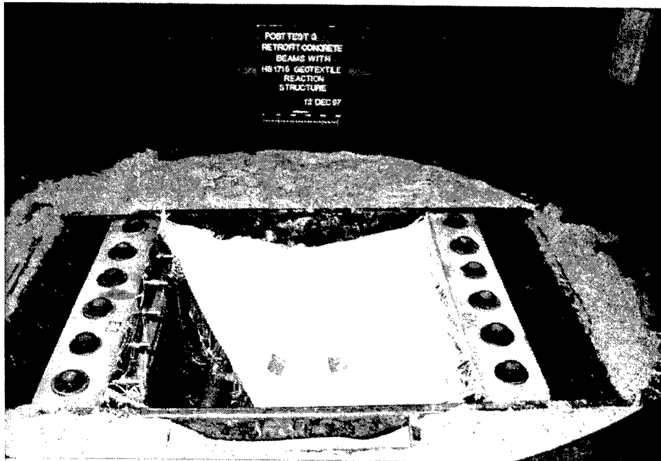
Figure 3.6. Group A test 3 posttest
