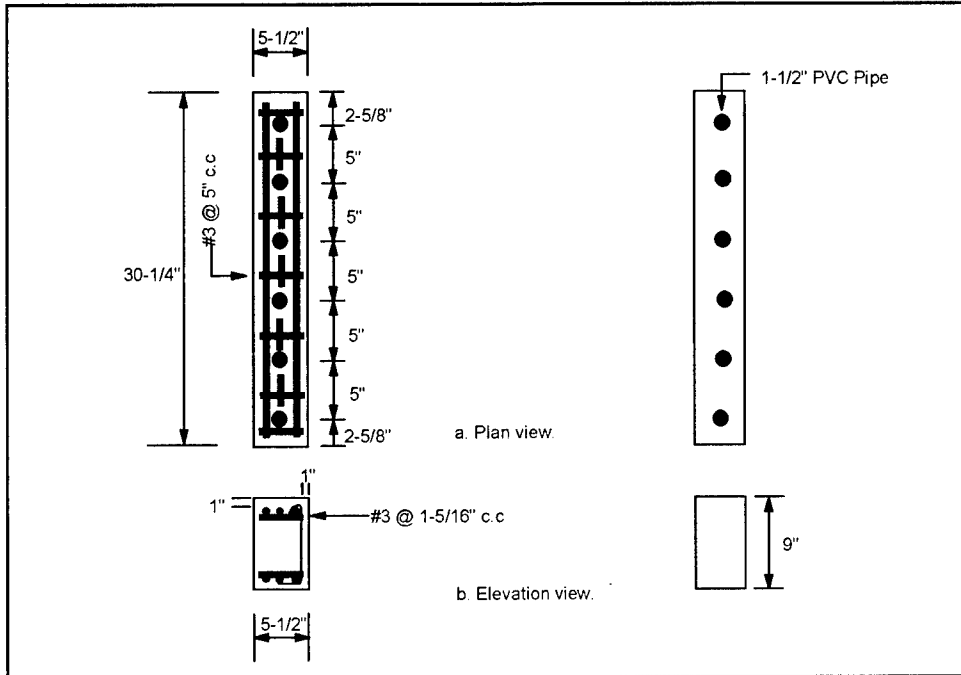
Figure 2.4. Detailed design of Concrete Beams
