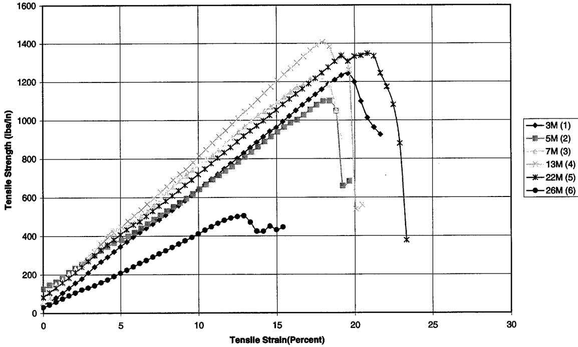
Figure C.11 ASTM 4595 Group A COM 350 Machine Direction.
