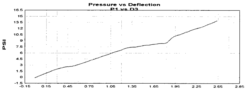
Figure A.18 Group B test 5 P1 pressure versus D3 deflection plot.
