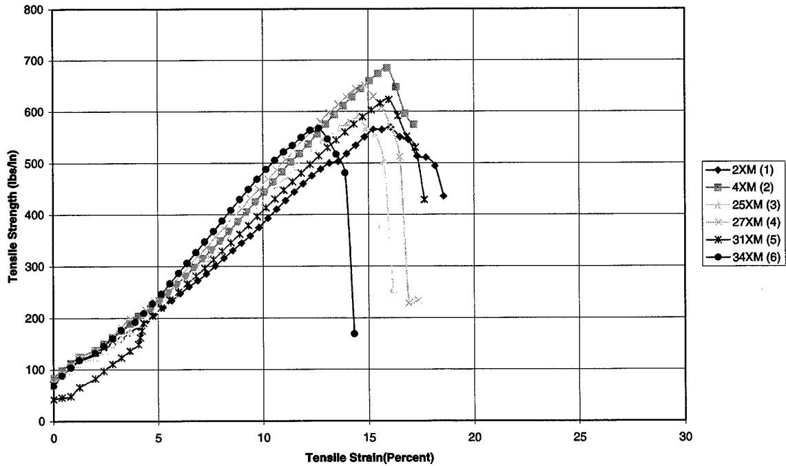
Figure C.12 ASTM 4595 Group A COM 350 Cross Direction.
