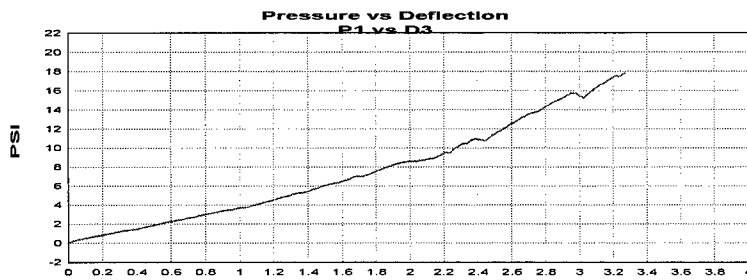
Figure A.7 Group A test 2 P1 pressure versus D3 deflection plot.
