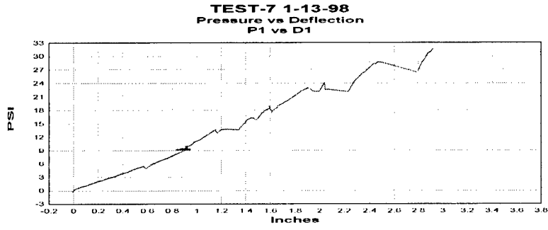
Figure A.23 Group A test 7 P1 pressure versus D1 deflection plot.
