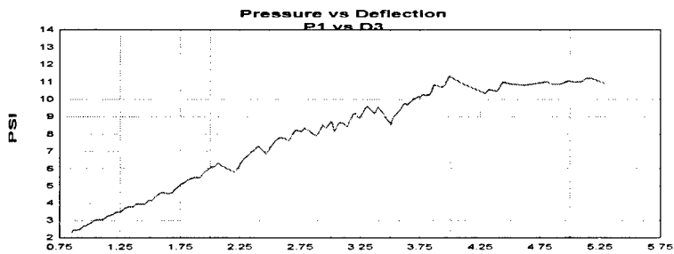
Figure A.3 Group A test 1 P1 pressure versus D3 deflection plot.
