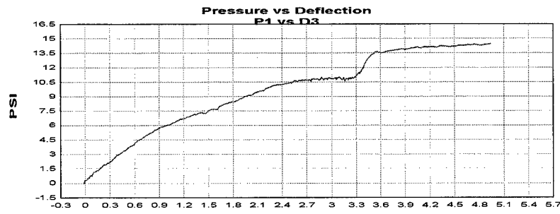
Figure A.34 Group B test 10 P1 pressure versus D3 deflection plot.
