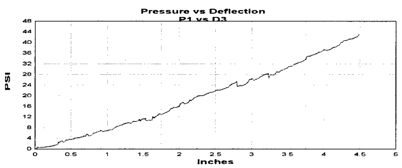
Figure A.37 Group A test 11 P1 pressure versus D3 deflection plot.
