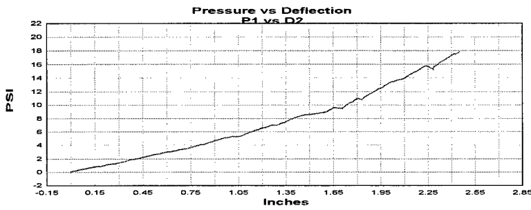
Figure A.6 Group A test 2 P1 pressure versus D2 deflection plot .
