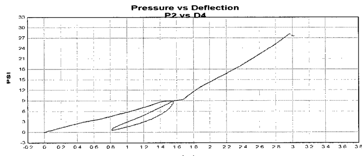
Figure A.15 Group B test 4 P2 pressure versus D4 deflection plot.
