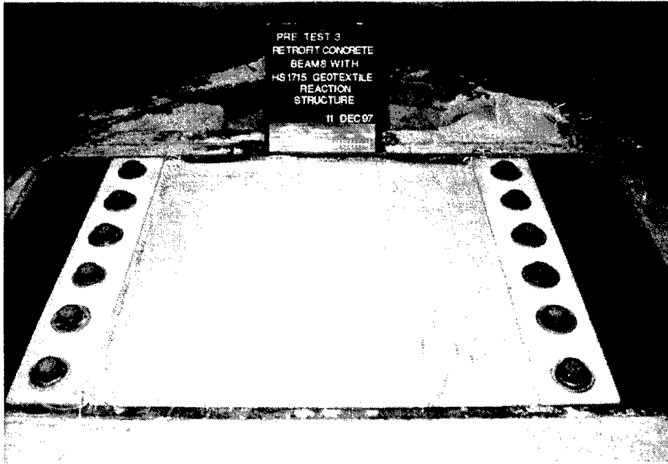
Figure 3.5. Group A test 3 pretest
