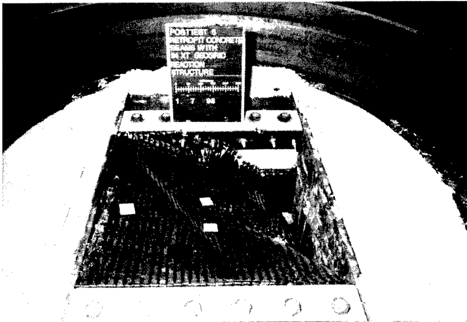
Figure 3.10. Group B test 5 posttest
