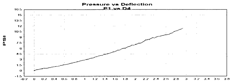
Figure A.12 Group A test 3 P1 pressure versus D4 deflection plot.
