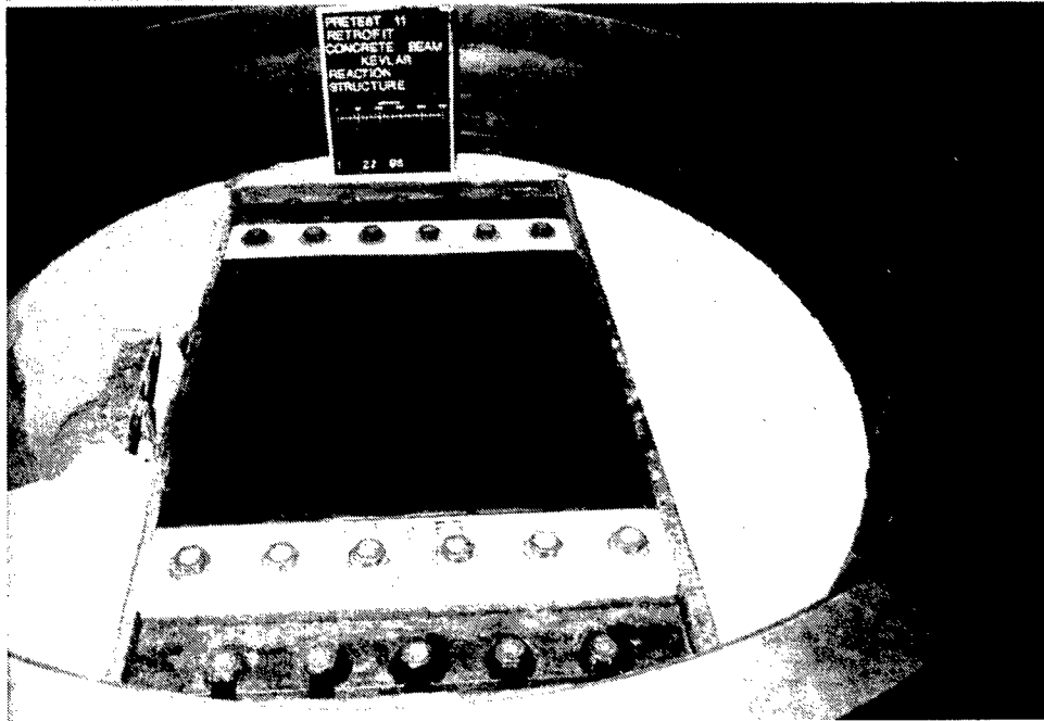
Figure 2.12. Typical test setup
