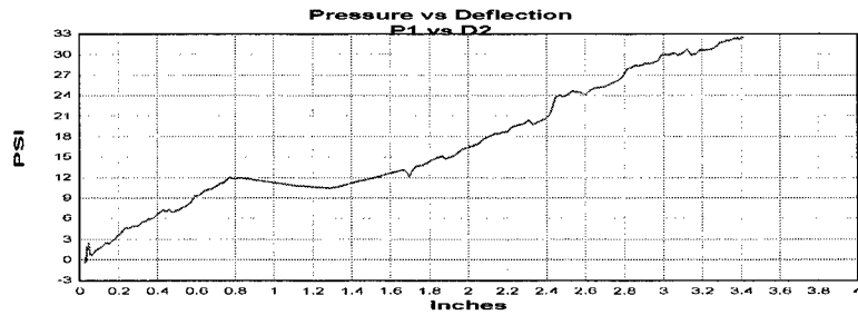
Figure A.40 Group A test 12 P1 pressure versus D2 deflection plot.
