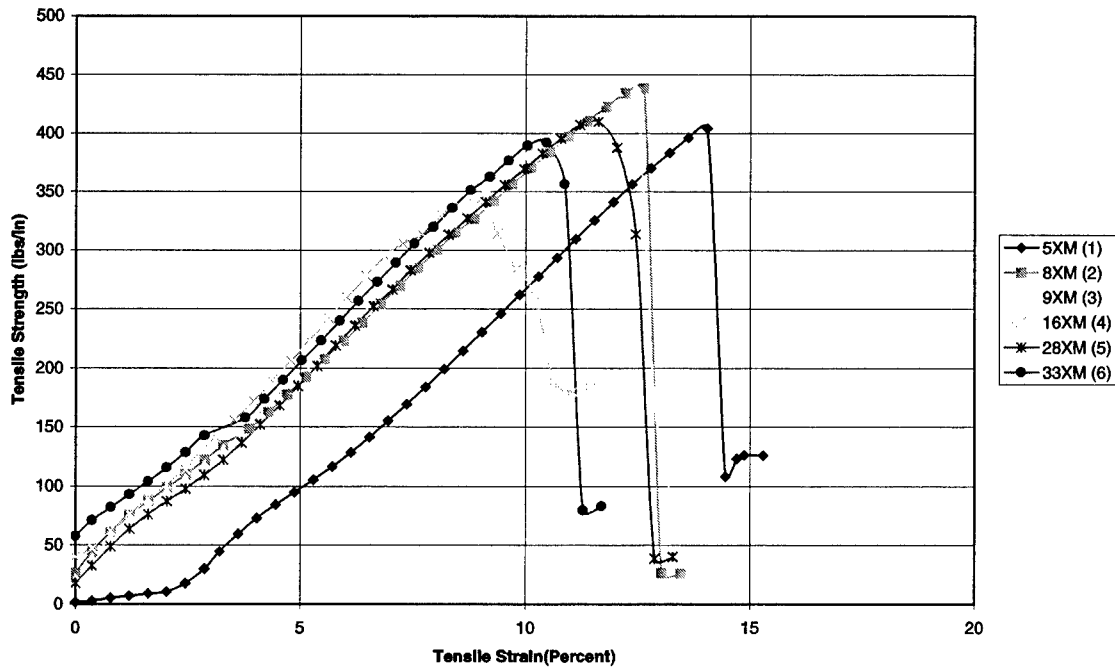
Figure C.14 ASTM 4595 Group A COM GT 500 Cross Direction.
