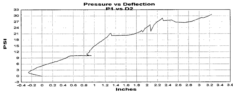
Figure A.28 Group A test 8 P1 pressure versus D2 deflection plot.
