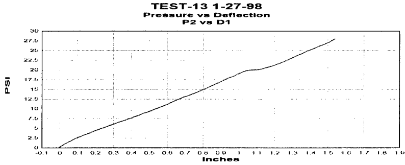
Figure A.43 Group A test 13 P2 pressure versus D1 deflection plot.
