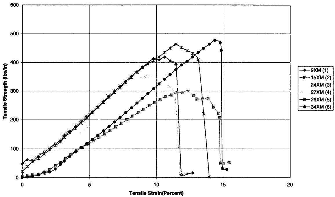
Figure C.2 ASTM 4595 Group A GT 600 Cross Direction.
