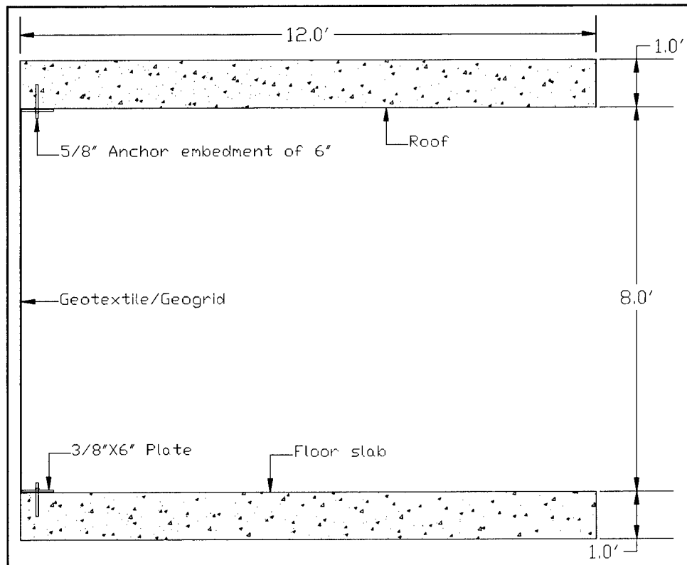
Figure 1.1. Proposed prototype retrofit system
