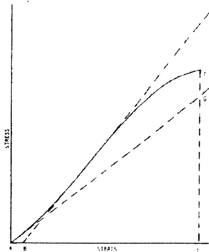
FIG. X1.1 Material with Hookean Region
