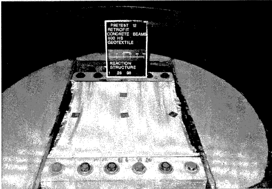
Figure 3.22. Group A test 12 pretest
