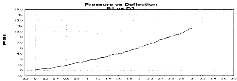
Figure A.11 Group A test 3 P1 pressure versus D3 deflection plot.
