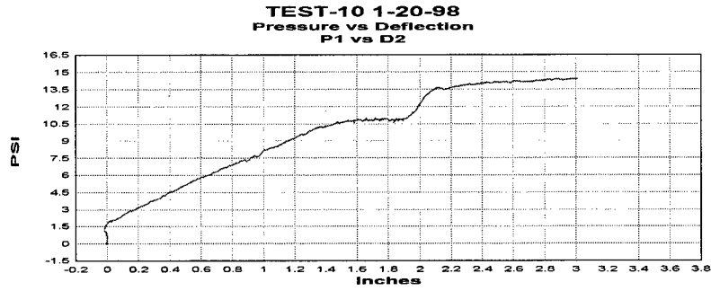
Figure A.33 Group B test 10 P1 pressure versus D2 deflection plot.
