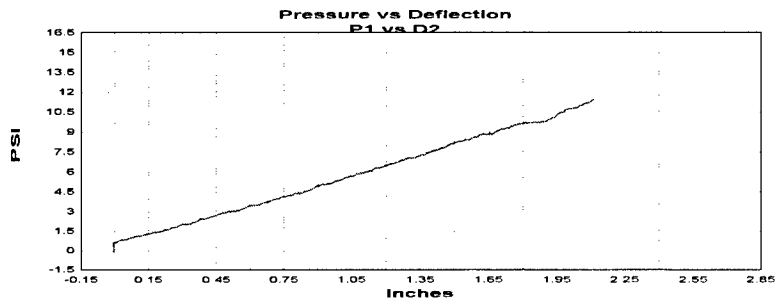
Figure A.10 Group A test 3 P1 pressure versus D2 deflection plot.
