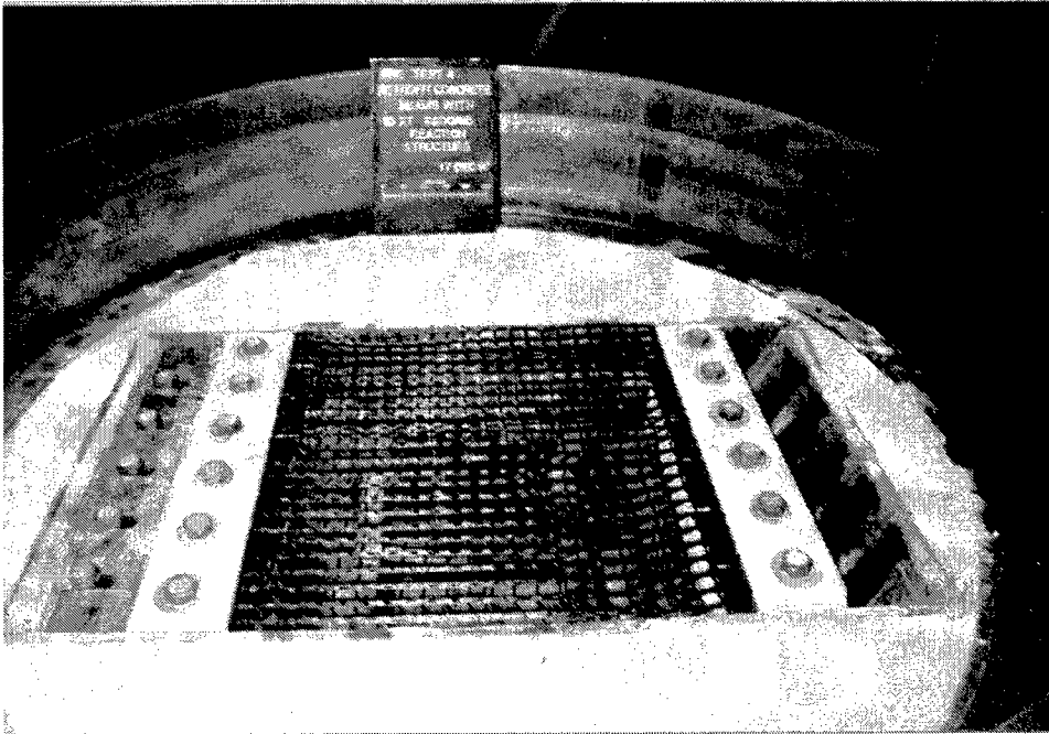
Figure 3.7. Group B test 4 pretest
