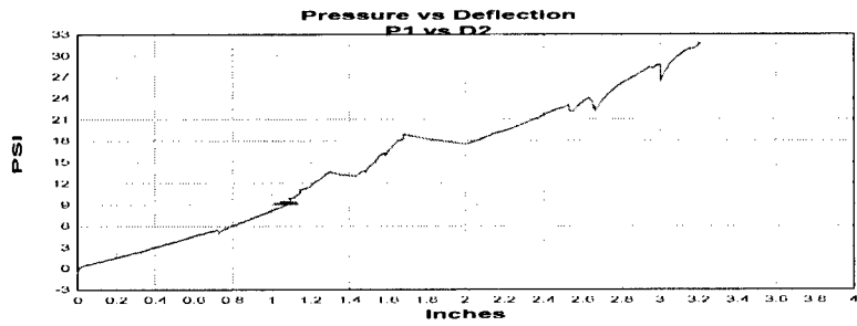
Figure A.24 Group A test 7 P1 pressure versus D2 deflection plot.
