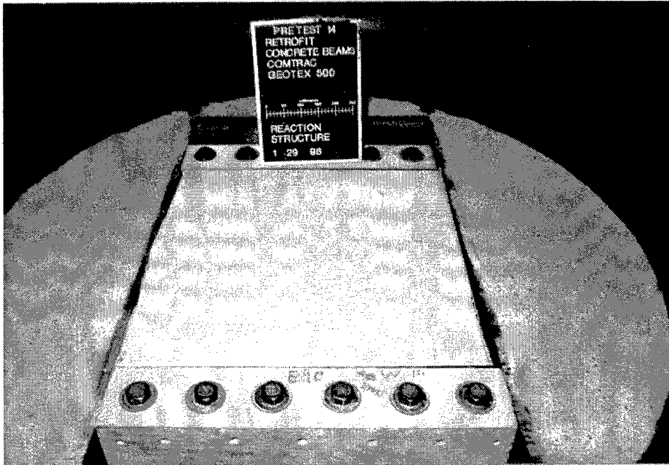
Figure 3.26. Group A test 14 pretest
