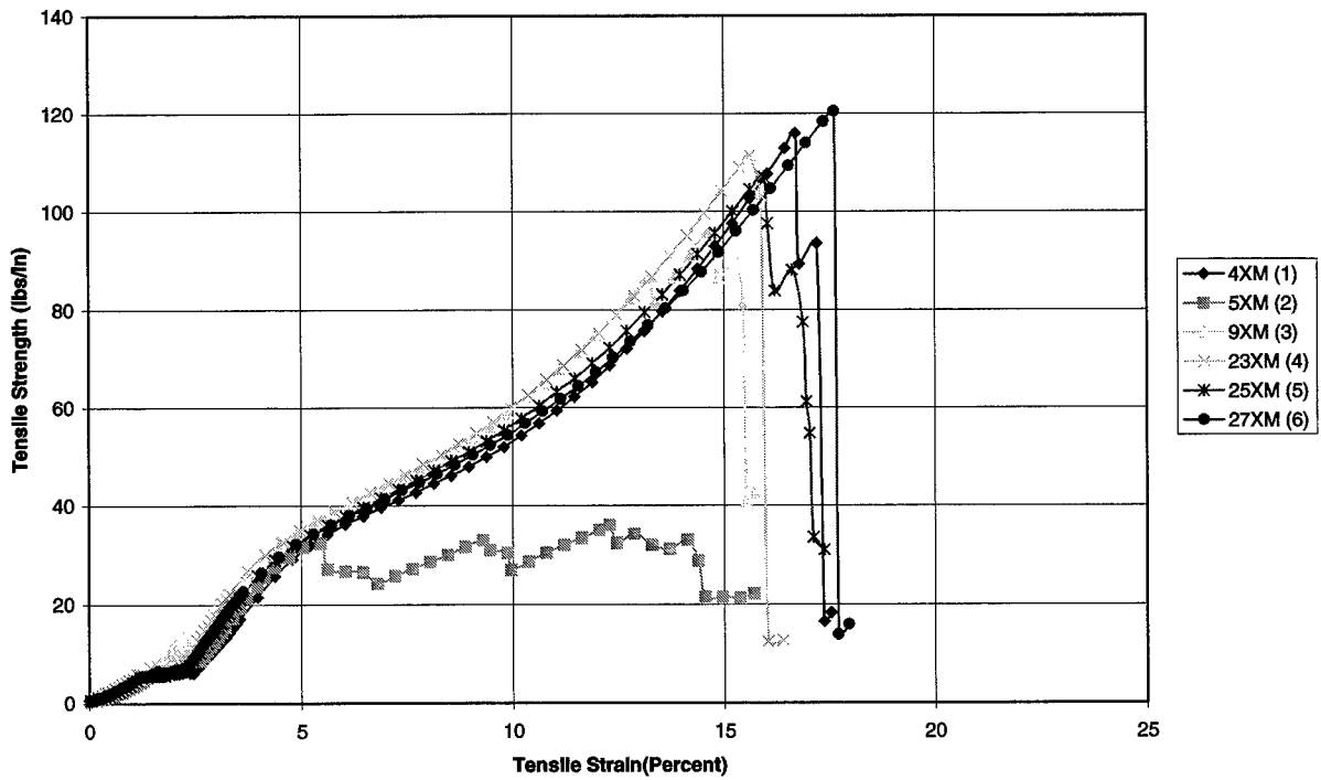
Figure C.8 ASTM 4595 Group B GG 10 Cross Direction.
