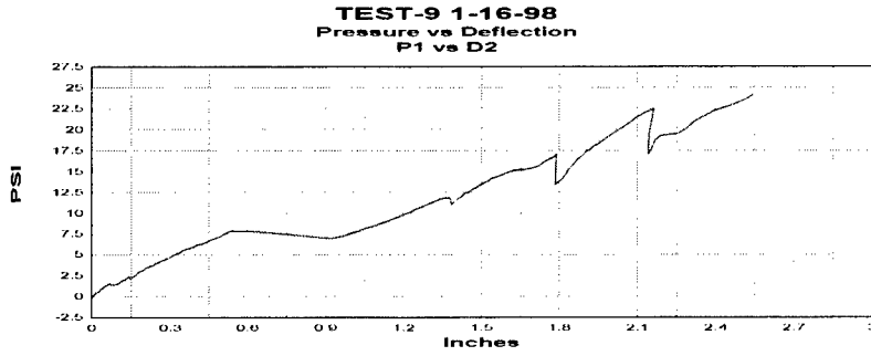
Figure A.30 Group A test 9 P1 pressure versus D2 deflection plot.
