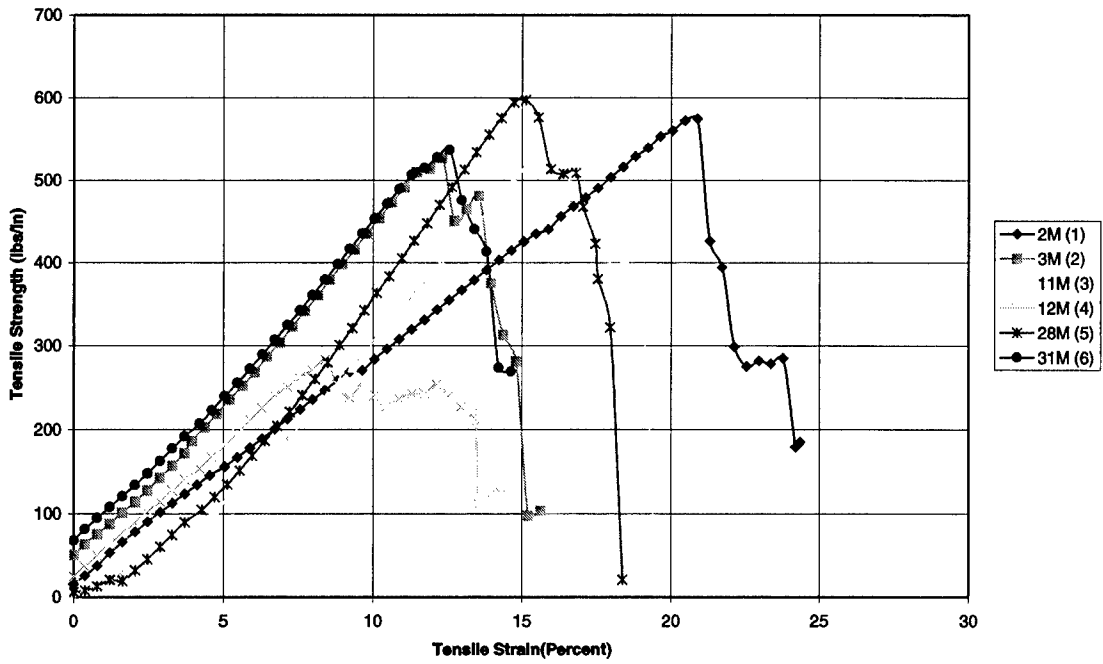
Figure C.1 ASTM 4595 Group A GT 600 Machine Direction.
