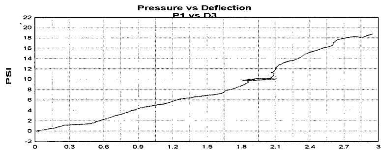
Figure A.22 Group A test 6 P1 pressure versus D3 deflection plot.
