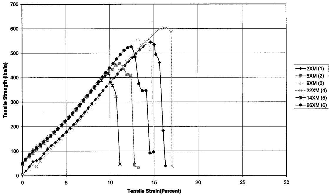
Figure C.4 ASTM 4595 Group A GT 800 Cross Direction.
