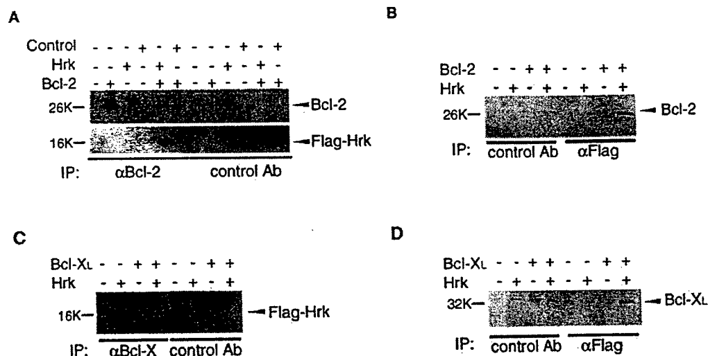
Fig. 2. Hrk interacts with Bcl-2 and Bcl-XL in mammalian cells. 293T cells ( 5 \times 10^6 per 100 mm plate) were transiently transfected with 10 \mu g of the indicated plasmids, pSFFV-Flag-tagged BP25 (control), pSFFV-Flag-Hrk16K (Hrk), pSFFV-hBcl-2 (Bcl-2), pSFFV-HA-hBcl-XL (Bcl-XL) or pSFFV-HA-mBax (Bax). In the case of transfection with a single plasmid, cells were co-transfected with 10 \mu g of empty pSFFV-neo vector and the total amount of plasmid DNA was always 20 \mu g. (A) Lysates were immunoprecipitated with anti-Bcl-2 or control antibody. Immunoprecipitates were immunoblotted with anti-Bcl-2 or anti-Flag antibody. (B) Anti-Flag or control antibody immunoprecipitates were immunoblotted with anti-Bcl-2 antibody. (C) Anti-Bcl-X or control antibody immunoprecipitates were immunoblotted with anti-Flag antibody. (D) Anti-Flag or control antibody immunoprecipitates were immunoblotted with anti-Bcl-X antibody. Notice that pSFFV-Flag-Hrk16K produces 16 kDa protein, as the entire harakiri cDNA including its 5' untranslated region was fused in-frame with the Flag sequence and the amino-terminus of Hrk.
