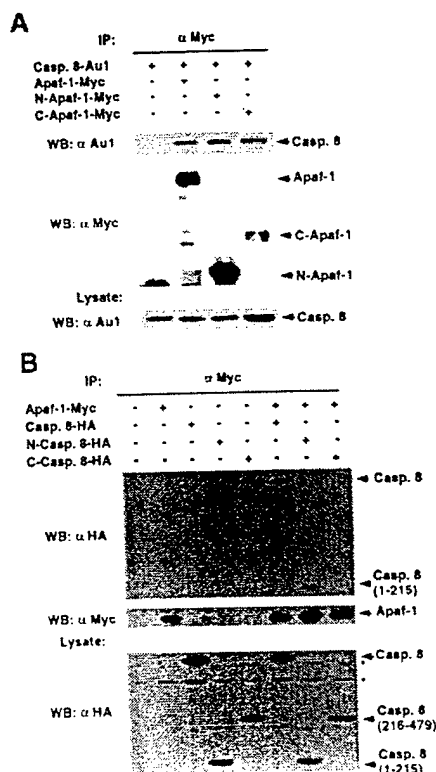
FIG. 2. Apaf-1 interacts with the prodomain of caspase-8. (A) Interaction of Apaf-1 with caspase-8. (B) Apaf-1 interacts with the prodomain of caspase-8. Immunoprecipitation analysis was performed as described in Fig. 1. (Upper) Western blot analysis of immunoprecipitated protein complexes with indicated antibodies. (A and B, Lower) show the expression of caspase-8 (A) or Apaf-1 (B) in total lysates by Western blot analysis. IP: immunoprecipitation, WB: Western blot analysis. Asterisks indicate nonspecific bands.
