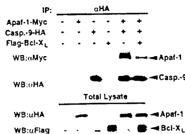
FIG. 5. Bcl-X L inhibits the association of Apaf-1 with caspase-9. 293T cells were transfected with indicated plasmids and the lysates immunoprecipitated with anti-HA antibody. (Upper) Western blot analysis of immunoprecipitated caspase-9 and coimmunoprecipitated Apaf-1. (Lower) Western blot analysis of total lysates with anti-Myc and anti-Flag antibody.
