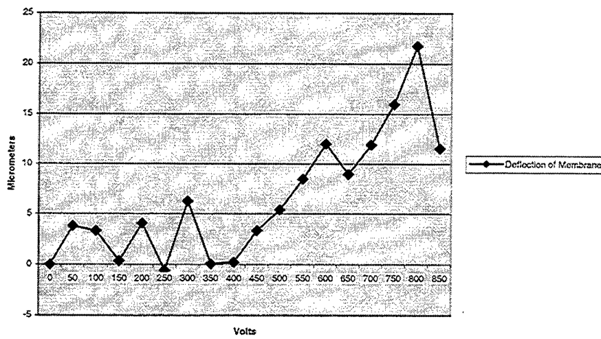
Deflection of Membrane due to Piezoelectric Effect (0.3 psi) - Positive Lead Attached to Positive Sign Side
