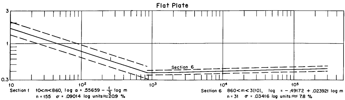
Fig. 4.20—Summary of the glass-fragment data. This shows regression lines describing \alpha vs. mass for (1) all the glass, (2) window glass dropped flat, (3) window glass dropped on edge, and (4) plate glass dropped flat.
