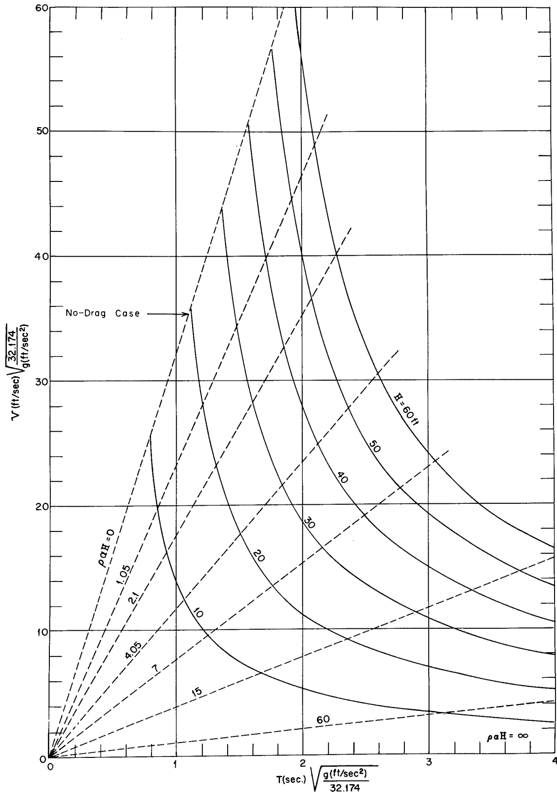
Fig. 2.5—Impact velocity vs. time of fall computed for several drop heights. Velocity and time can be evaluated for any acceleration of gravity. \rho \alpha H lines are included for orientation.
