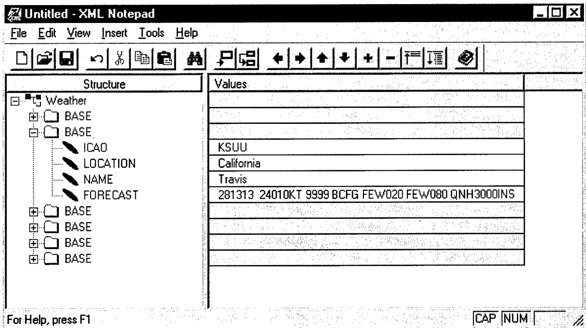
Screen 3-3 XMLNotepad
