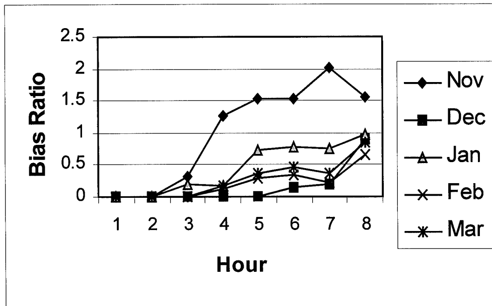
Figure 15 Bias ratio by month for Tower 1101 at the 162-foot level.
