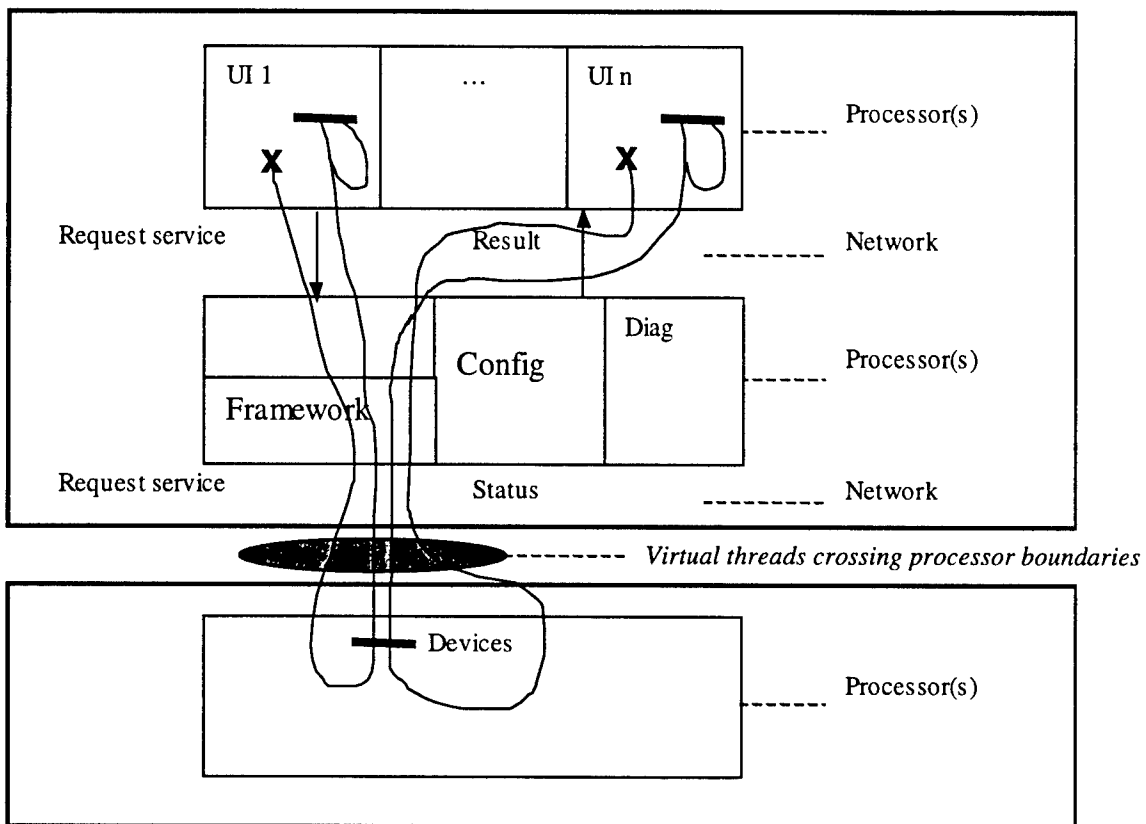
Figure 10: Use-Case Map for Two Simultaneous Users on Deployed System
