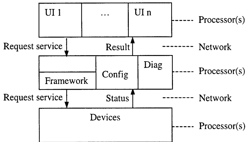
Figure 3: Allocation of Encapsulated Function to Style
