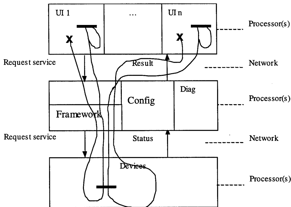
Figure 7: Use-Case Map for Two Simultaneous Users
