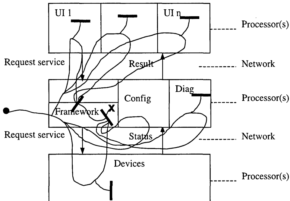
Figure 6: Use-Case Map for Start-Up
