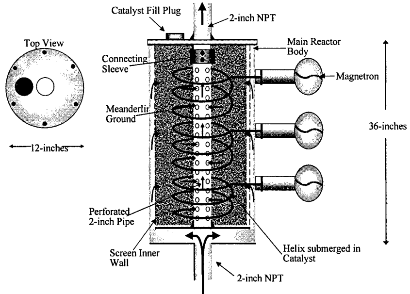
Figure 10 Radial Microwave Reactor for 58-hp Diesel Engine Exhaust.
