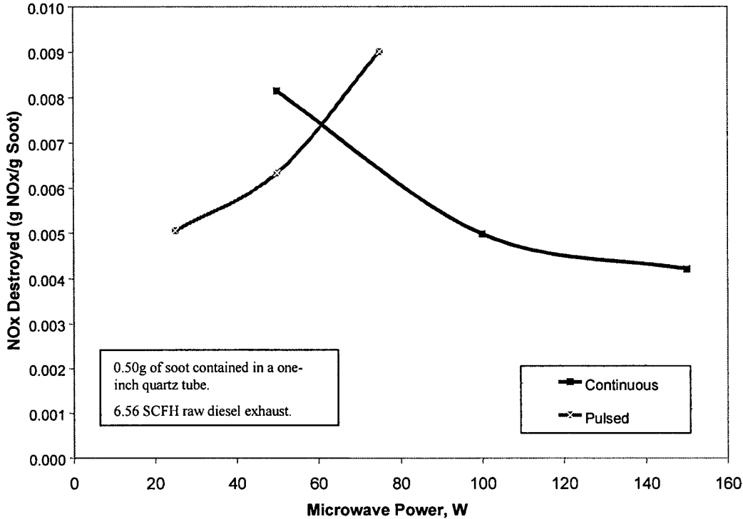
Figure 4. NOx Destruction through Microwave Induced Soot Oxidation
