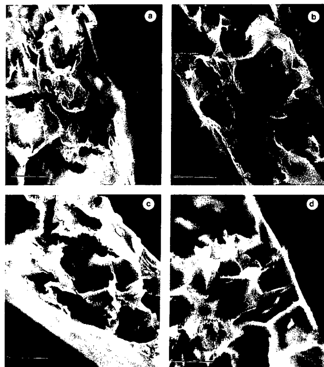
FIG. 7. SEM images of porous polymer foams. (a) PLLA; (b) PLLA/PCBZL mixture; (c) deprotected PLLA/PCBZL; and (d) deprotected PLLA/PCBZL with covalently attached collagen. Bar = 100 \mu m.
