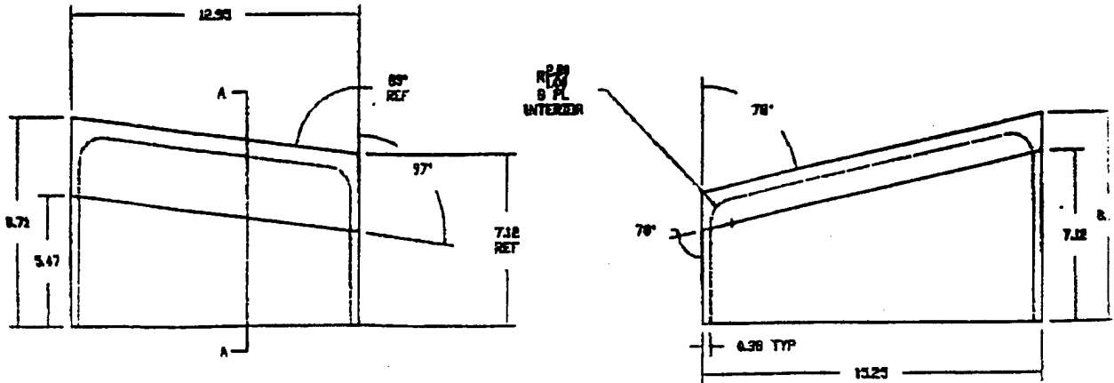
Figure 2. A Drawing of the Proposed Bumper Panels Required for the Project (Mirror Image Versions of Both the Skirt and Bumper Panels Were Also Needed).
