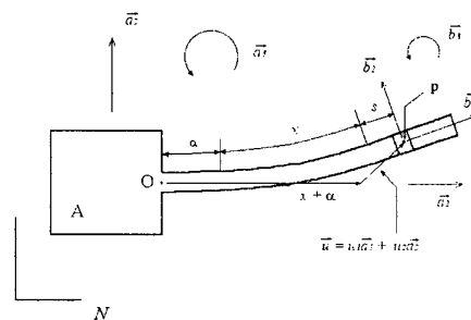
Fig. 1 Deployment of a Beam in 2 - Dimensional Space
