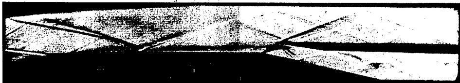
Fig.2 Schlieren photograph of inlet and dual combustors ( h_p=12.93\text{mm} )
