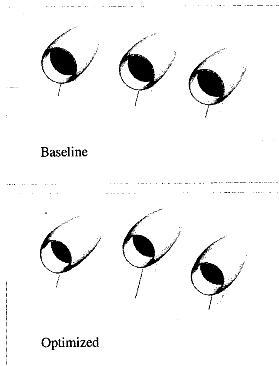
Figure 7: Comparison of baseline and optimized podded BWB configurations.
