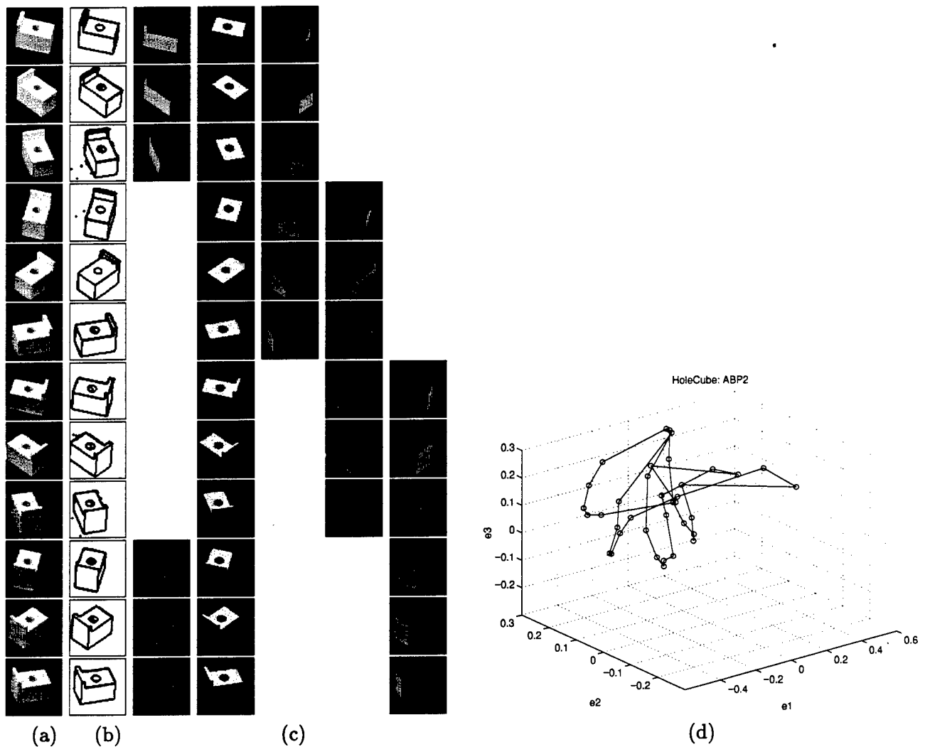
Figure 6: Collection of appearances of parts for “HoleCube”. (a) Images of “HoleCube” every 30°. (b) MDL segmentations of the images in (a). (c) Appearances of five parts. (d) Manifold corresponding to the second part, shown as three dimensional for visualization purposes.
