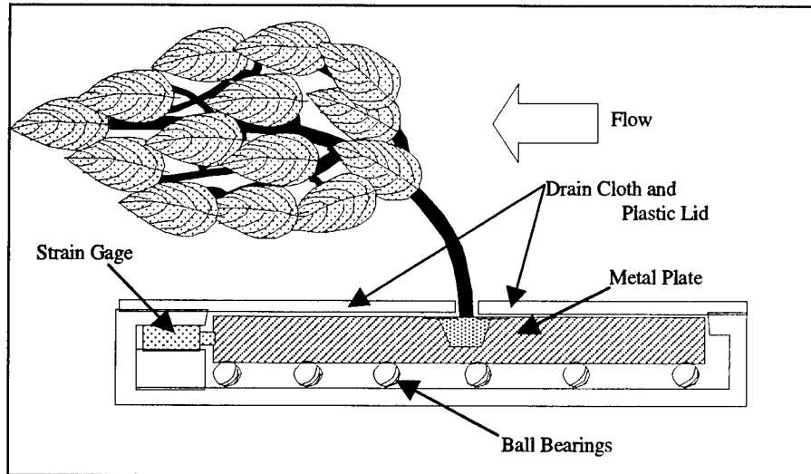
Figure 4. Experimental setup to measure plant drag
