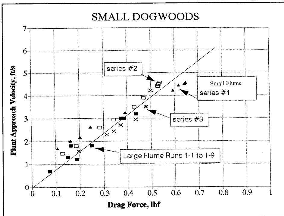
Figure 13. Plant approach velocity versus drag force (To convert feet to meters, multiply by 0.3048) [To convert pounds (force) to newtons, multiply by 4.448222]
