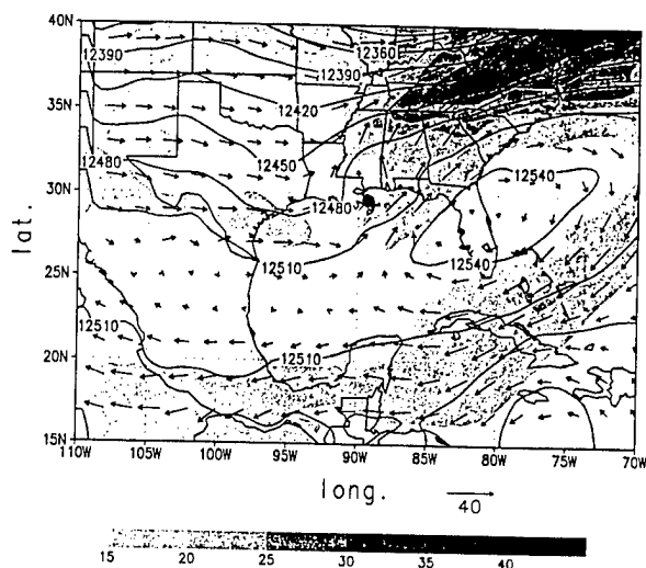
FIG. 11. Same as Fig. 10 except for at 24 h valid at 0000 UTC 10 September 1988.
