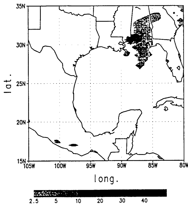
FIG. 18. Same as Fig. 16 except for experiment control + SSMI.
