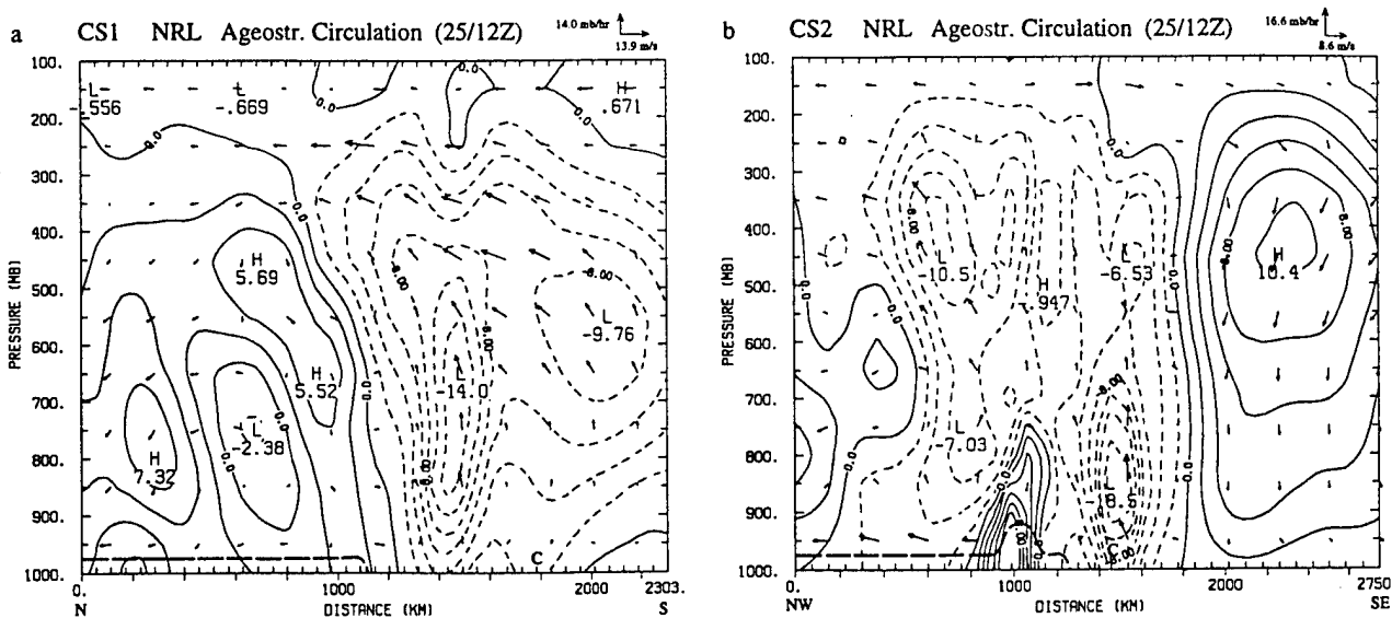
FIG. 12. As in Fig. 11 but for the vertical motion and ageostrophic wind in the plane of the cross sections (a) CS1 and (b) CS2. Contours of the vertical motion are every 2 \text{ mb h}^{-1} . Scale of vectors indicated by labeled arrows.
