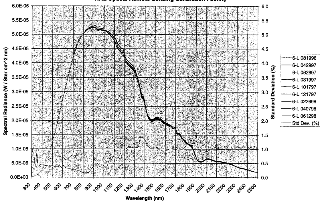
Labsphere Unisource 4000 Calibration (6 Lamps) 08/96-06/98 NRL Optical Remote Sensing Calibration Facility
