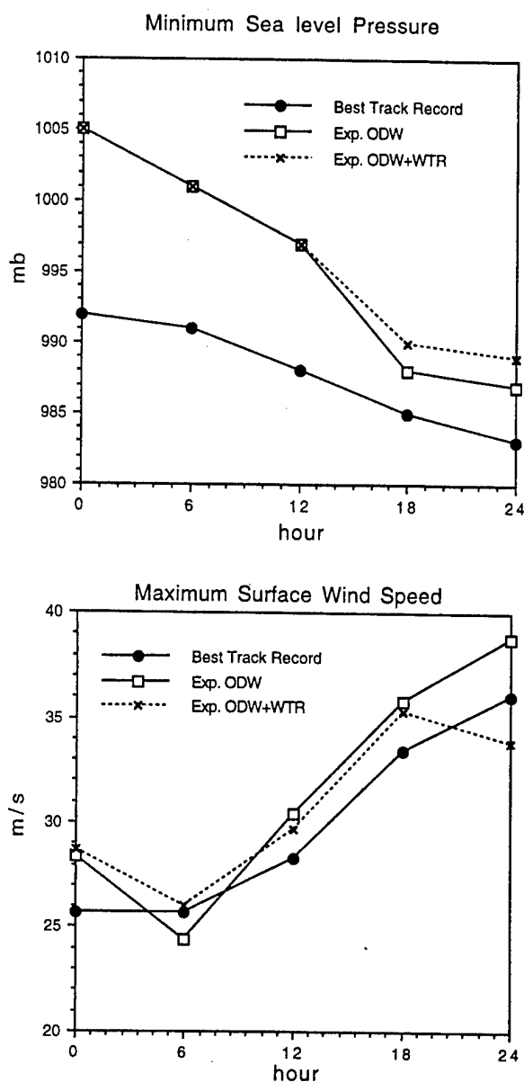
FIG. 18. Time variation of the minimum sea level pressure (mb) and maximum surface wind speed ( \text{m s}^{-1} ) of Expt. ODW and ODW+WTR.
