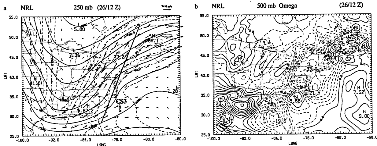
FIG. 18. (a) The geopotential height (gpm), temperature (°C), and winds at 250 mb; and (b) the vertical velocity (mb h⁻¹) at 500 mb for the NRL analysis at 1200 UTC 26 January. Contours as in Fig. 10.
