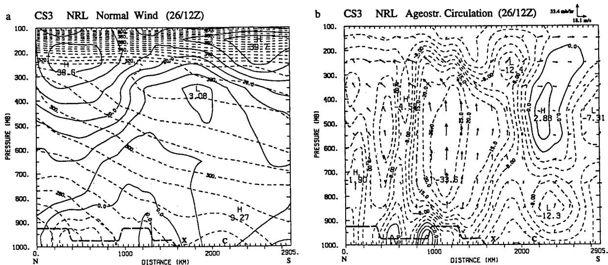
FIG. 19. (a) The wind normal to the cross section CS3 from 53°N, 70°W to 28°N, 80°W and (b) the vertical motion (mb h⁻¹) and ageostrophic wind (m s⁻¹) in the plane of cross section for 1200 UTC 26 January. Contours as in Figs. 11 and 12 except that contours of vertical motion less than -12 and -40 mb h⁻¹ are every 5 and 15 mb h⁻¹, respectively.
