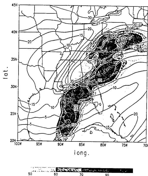
FIG. 12. 200-mb relative humidities (%) (shaded area) and isotachs (contour) of Expt. ODW at 12 h valid at 1200 UTC 9 September 1988.
