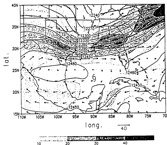
FIG. 5. 200-mb geopotential height contours (m), wind vectors, and shaded isotachs ( \text{m s}^{-1} ) of the NMC/RAFS 2.5^\circ analysis at 1200 UTC 8 September 1988. The hurricane symbol depicts the current center location of Florence from the best track record.
