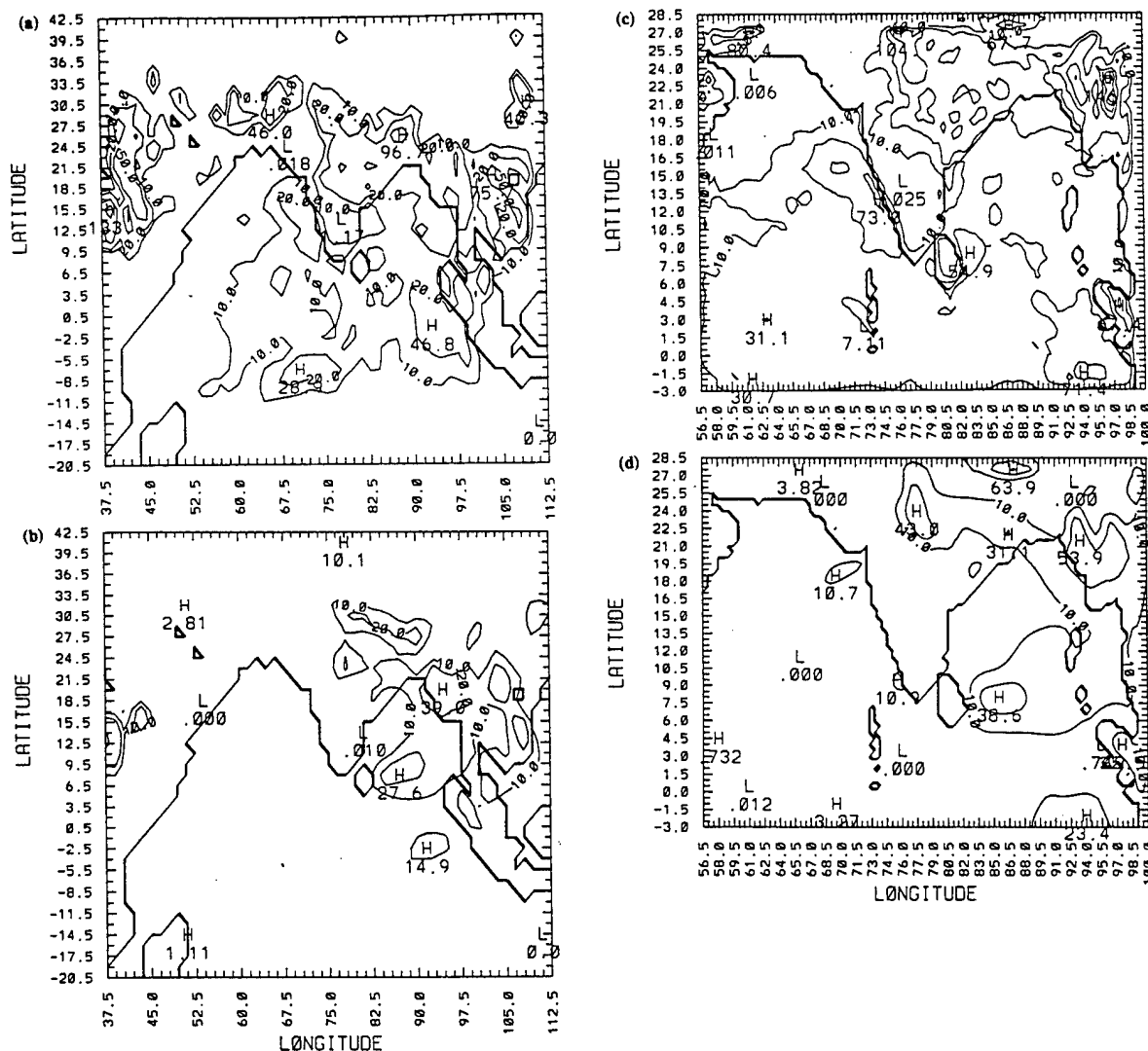
Fig. 5. Predicted rainfall for the CGM domain for a period of 24 hours ending at 12 UTC 13 July 1988 in the (a) KUO and the (b) BMS, respectively. Contour intervals are 10, 20, 50, 80 \text{mm d}^{-1} . Predicted rainfall for the FGM domain for a period of 24 hours ending at 12 UTC 13 July 1988 in the (c) KUO and the (d) BMS, respectively. Contour intervals are 10, 25, 50, 75, 100 \text{mm d}^{-1} .
