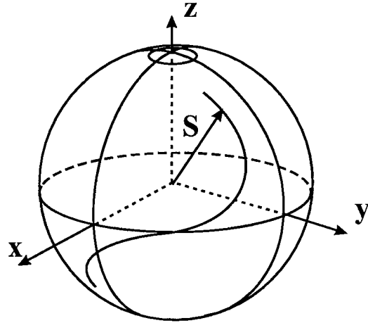
Figure 2.3: The two-state optical response is represented by the motion of the Bloch vector \mathbf{S} in the Bloch sphere. The \hat{\mathbf{x}} component of \mathbf{S} corresponds to the polarization in-phase with the electric field, which is responsible for dispersive effects. The \hat{\mathbf{y}} component is the in-quadrature polarization responsible for absorption and gain. The \hat{\mathbf{z}} component is the inversion.
