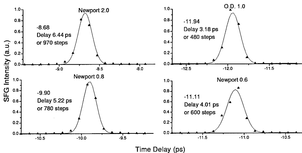
Figure F.3: More optical density filters. See Figure F.2 for notes.
