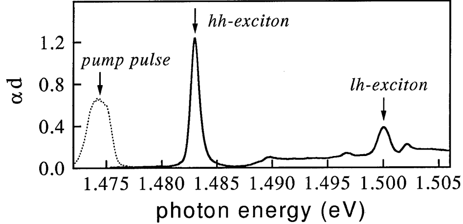
Figure 7.1: Linear absorption spectrum of the \text{In}_{0.04}\text{Ga}_{0.96}\text{As} MQW sample used in the Stark shifting experiment (solid line). The 1s hh -exciton and 1s lh -exciton resonances are labeled, and the other smaller resonances are not positively identified. The pump pulse spectrum is shown (dotted line) for a detuning of 8.5 meV (5 nm), with amplitude scaled in arbitrary units.
