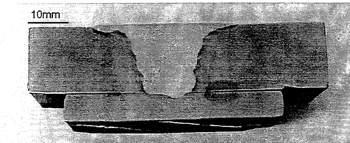
Figure 4.15 Macroscopic image of SNI-10
