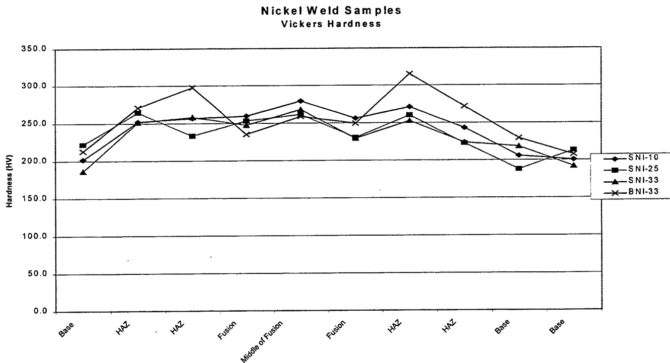
Figure 4.14 Plot of hardness results
