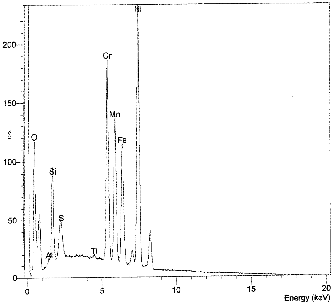
Figure 4.11 EDX spectrum of typical oxide inclusion
