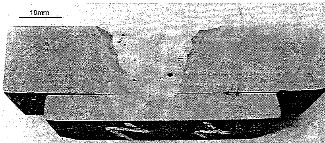
Figure 4.16 Macroscopic image of SNI-25
