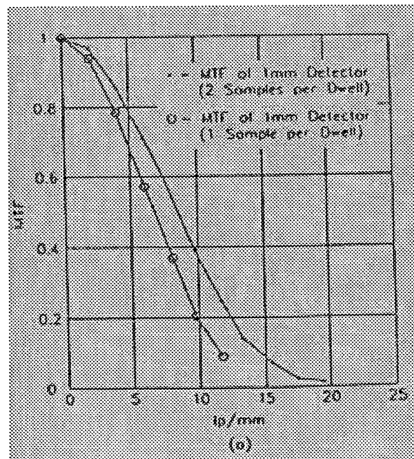
Figure 6: Comparison of MTF (film and DXM-1)
