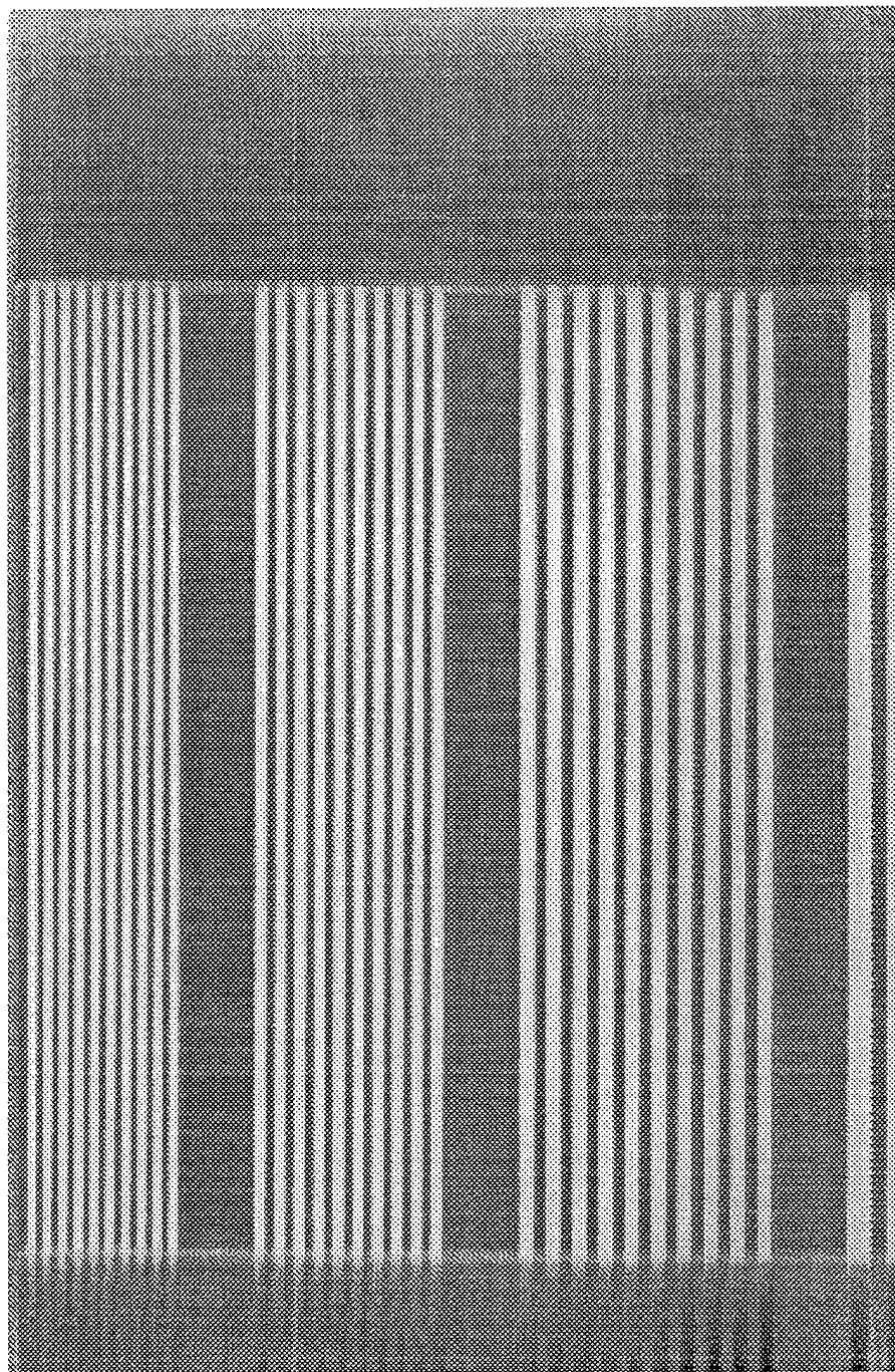
Figure E4: Lead-foil Penetrameter Image Acquired with a Thallium Bromide Coated Semiconductor Sensor Array (3.0, 2.5 and 2.0 lp/mm)
