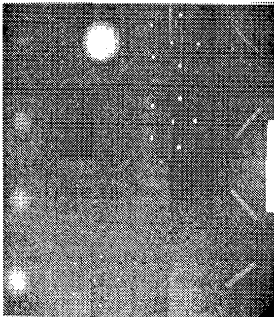
Figure B-27: ACR Accreditation Phantom Image Acquired with the DXM-1 15 of 16 spec groups visible
