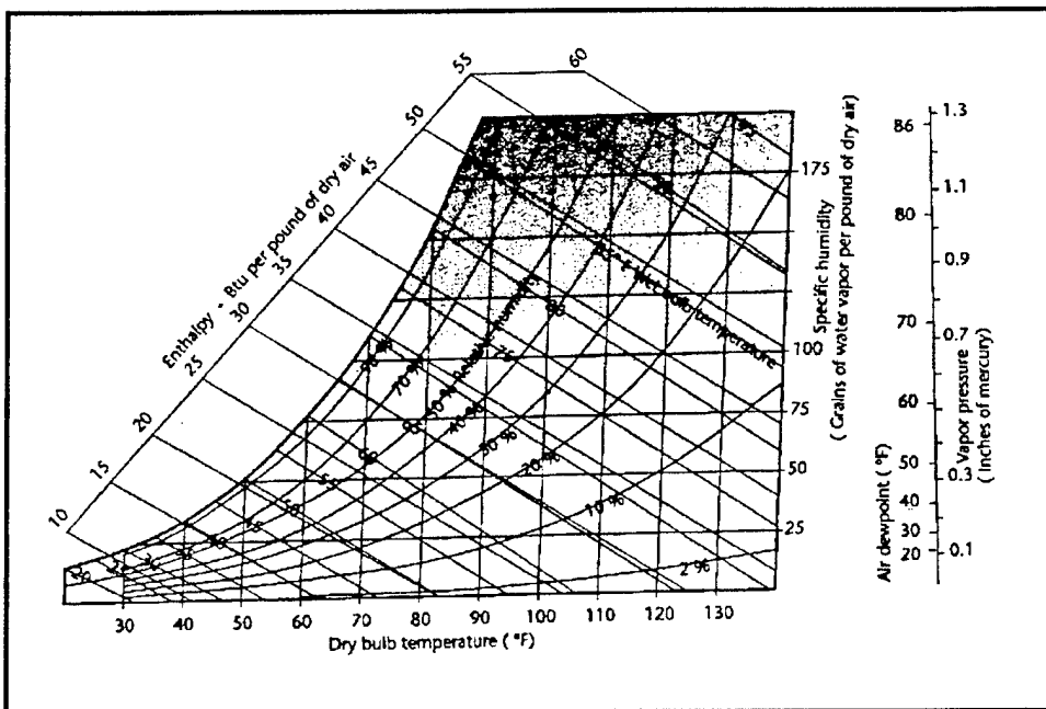
Figure 2. Psychrometric chart.
