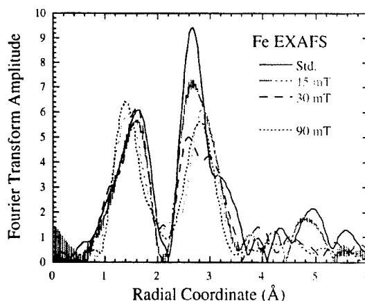
Figure 2. Fourier transform of Fe EXAFS-amplitude for single crystalline MnZn-ferrite films deposited at 300°C for O_2 pressures between 15 and 90 milliTorr.
