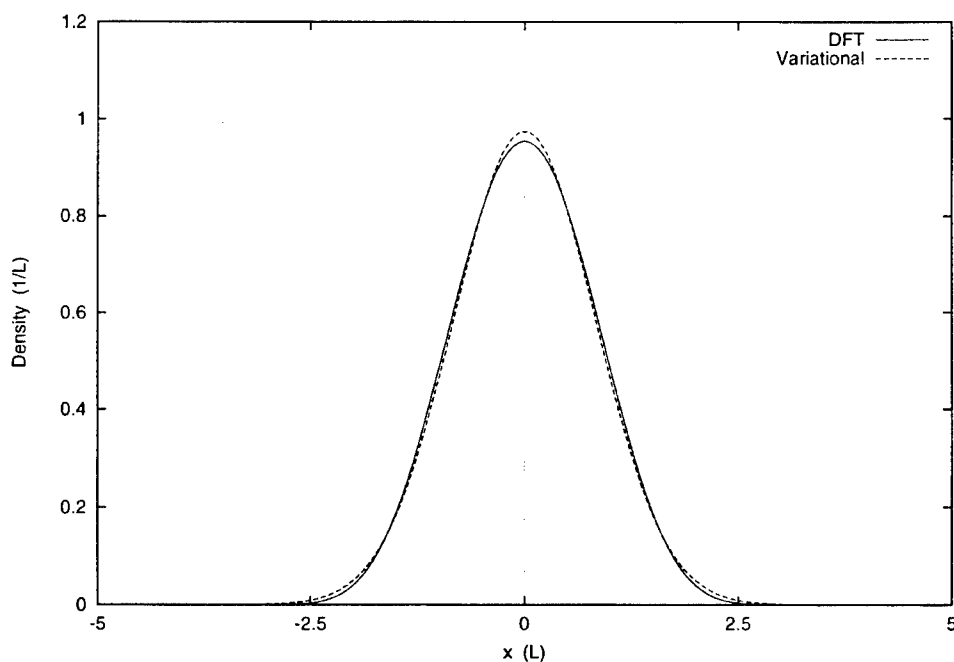
FIGURE 2. Plot of \rho(x) versus x for the external potential given by v(x) = \alpha \exp(\beta x^2) . The DFT calculation ( E = 2.98021 J, \mu=1.64453 J) is compared to a variational calculation ( E = 2.98168 J). The values of \alpha and \beta are 1 Joule and 1 \text{ L}^{-2} , respectively.
