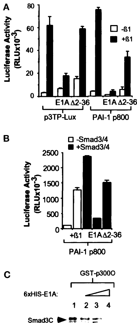
Figure 4. E1A inhibits Smad-dependent transcriptional activation. (A) E1A, but not the p300 binding mutant E1A \Delta 2-36 , blocks transcriptional activation of 3TP-Lux and PAI-1-Luc. HaCaT cells were cotransfected with 3 \mu g of 3TP-Lux or PAI-1-Luc reporter constructs and 4 \mu g of the indicated E1A expression constructs. The total amount of DNA was kept constant with the addition of vector control pCDNA3. TGF- \beta was added 12 h after transfection, and luciferase activity was measured 24 h later. Error bars represent the SD for duplicate transfections in a single experiment. "E1A" stands for wild-type E1A, and " \Delta 2-36 " stands for E1A \Delta 2-36 mutant. (B) The transcriptional activation induced by Smad3/Smad4 overexpression is inhibited by E1A in a p300-dependent manner. HaCaT cells were cotransfected with 3 \mu g of PAI-1, 3 \mu g of Smad3/Smad4, and 4 \mu g of E1A expression constructs as indicated. The total DNA amount was kept constant with the addition of pCDNA3. After transfection and TGF- \beta treatment, luciferase activity was measured as above. (C) E1A can compete with Smad3 for interaction with p300. COS-overexpressed HA-tagged Smad3C (aa 199–424) was used to assess the ability of Smad3 to interact with p300 in the presence of E1A. Eluted bacterial-produced 6XHis E1A was added in increasing amounts from lanes 2 to 4 to the GST-p300C pull-down
