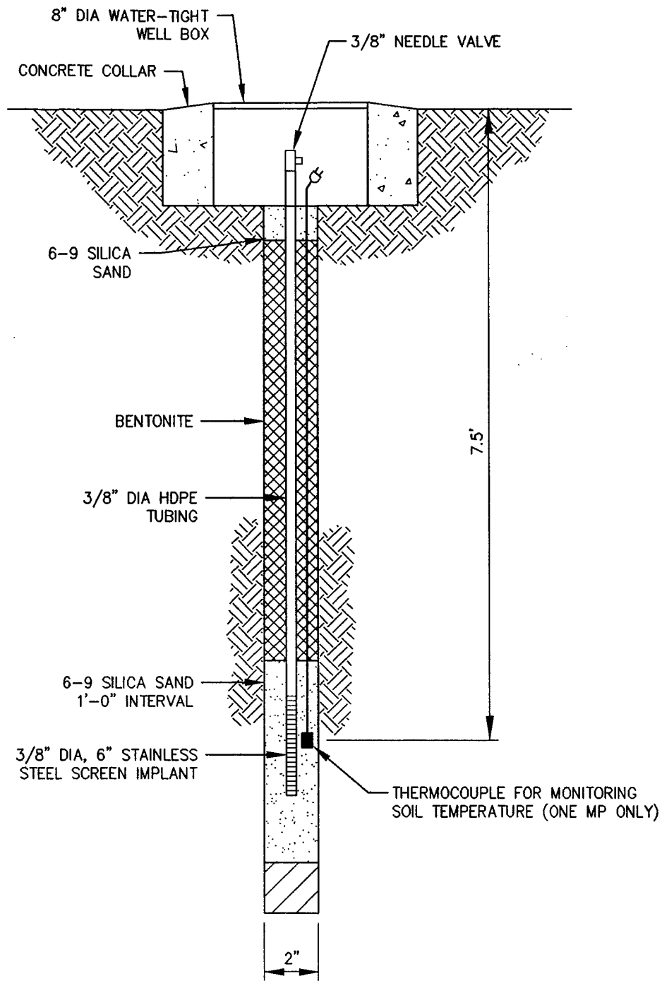
FIGURE 3.6 PROPOSED MONITORING POINT CONSTRUCTION DETAIL BUILDING 457 AREA (TYPICAL) Eaker AFB, Arkansas PARSONS ENGINEERING SCIENCE, INC. Denver, Colorado
