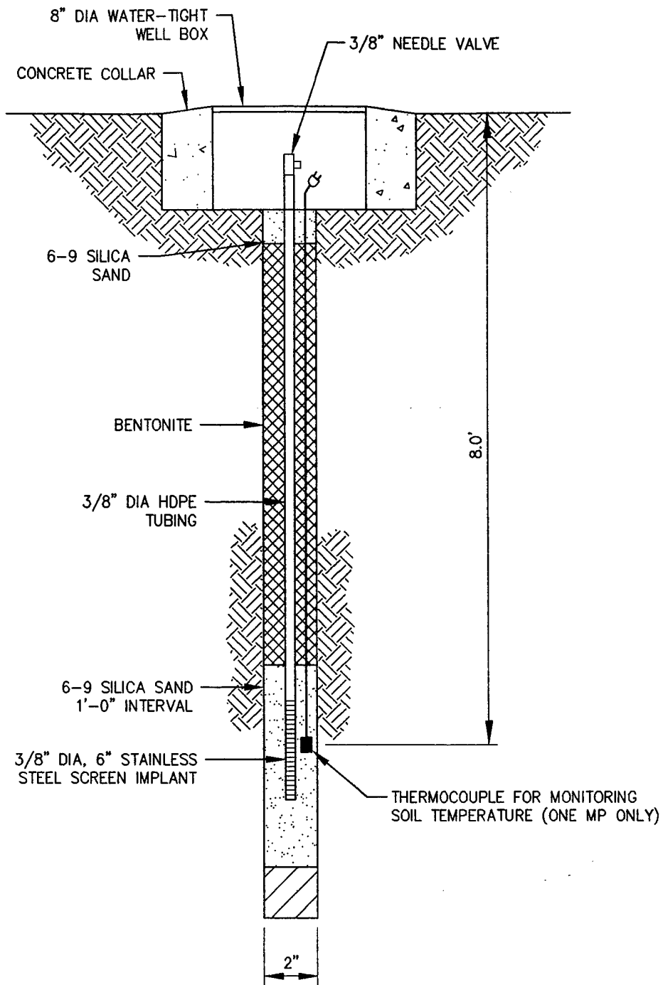
FIGURE 3.9 PROPOSED MONITORING POINT CONSTRUCTION DETAIL UST 702 (TYPICAL) Eaker AFB, Arkansas PARSONS ENGINEERING SCIENCE, INC. Denver, Colorado
