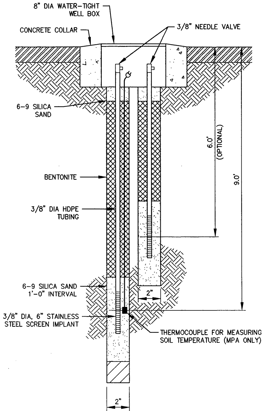
FIGURE 3.3 PROPOSED MONITORING POINT CONSTRUCTION DETAIL SPILL SITE NO. 1 (TYPICAL) Eaker AFB, Arkansas PARSONS ENGINEERING SCIENCE, INC. Denver, Colorado
