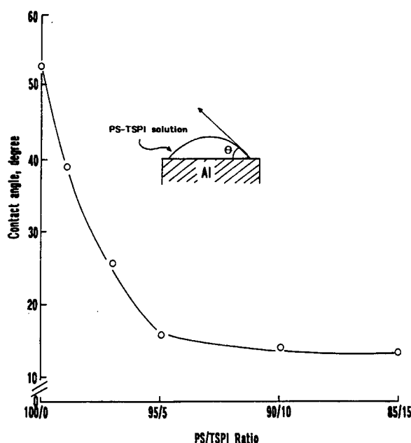
Fig. 5. Contact angles for various different [PS]/[TSPI] ratio solutions dropped onto the Al substrate surface.
