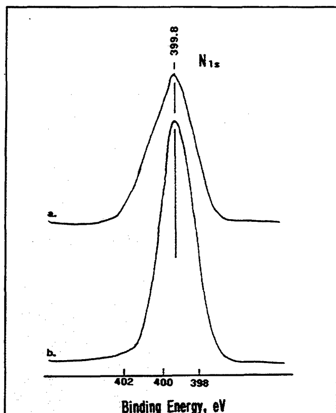
Figure 7— N_{1s} region for (a) 70/30 and (b) 0/100 ratio-coated Al.
