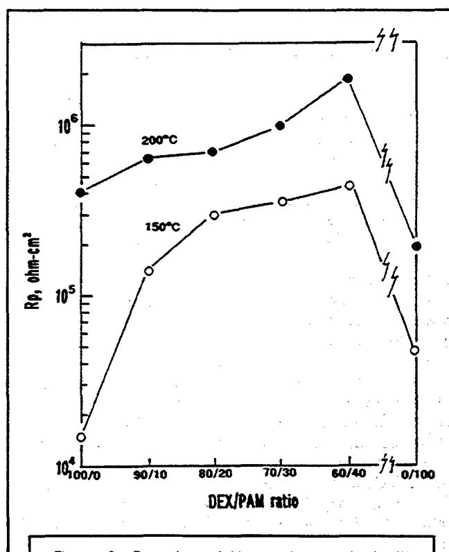
Figure 8— R_p value of Al samples coated with 100/0, 90/10, 80/20, 70/30, 60/40, and 0/100 ratios at 150° and 200°C.
