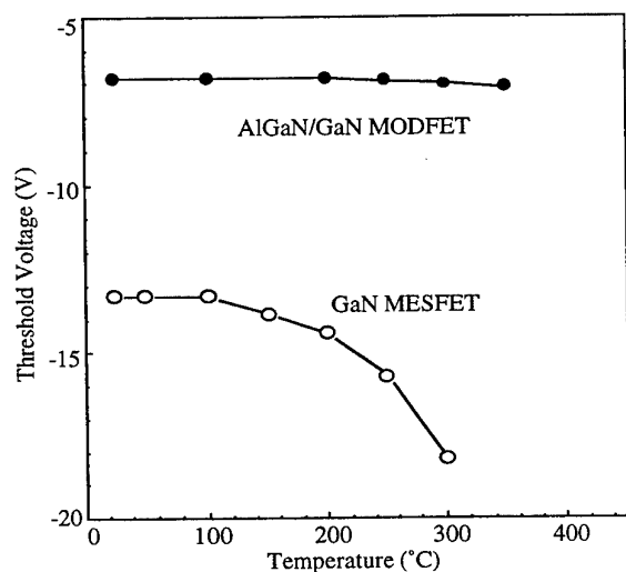
Fig. 5. Dependence of V_{\text{th}} on temperature for the \text{GaN} MESFET and \text{AlGaIn}/\text{GaN} MODFET on sapphire.
