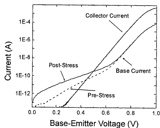
Fig. 5. Gummel plot for the device used for Fig. 4, before and after the application of stress. The emitter area was 0.8 \times 3 \mu m^2 .
