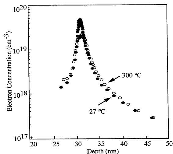
Fig. 6. Carrier concentration profiles measured by C-V method at 25 and 300 °C for the \text{AlGaIn}/\text{GaN} MODFET.
