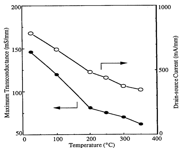
Fig. 4. Transconductance g_m and drain-source current I_{\text{DS}} as a function of temperature for the \text{AlGaIn}/\text{GaN} MODFET with L_g = 2.1 \mu\text{m} .
