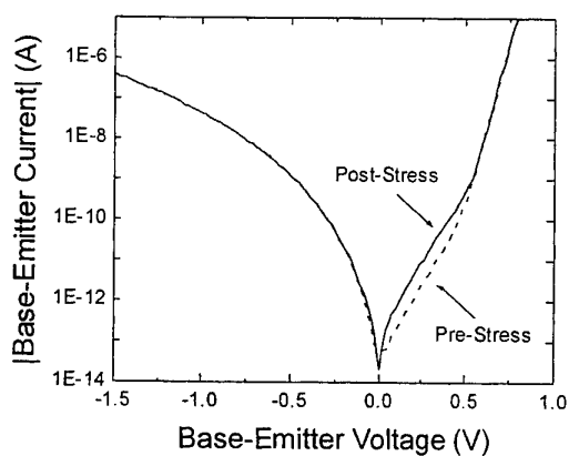
Fig. 4. The absolute value of the emitter-base diode current before and after the reverse-bias stress. The collector and base were connected together and -2.5V was applied to the emitter for 3000 secs.
