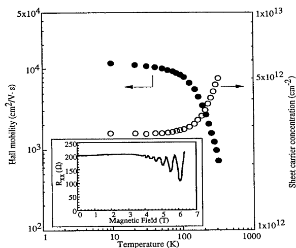
Fig. 2. 2DEG mobility and sheet carrier density as a function of temperature for the \text{AlGaIn}/\text{GaN} heterostructure. Inset shows the magnetoresistance R_{xx} as a function of magnetic field at 4.2 K.
