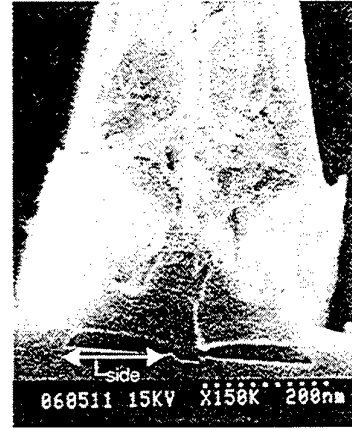
Fig. 2: Scanning electron microscope photograph of a 30-nm-gate HEMT. Lateral depth of the gate recess is defined as recess length ( L_{side} ).
