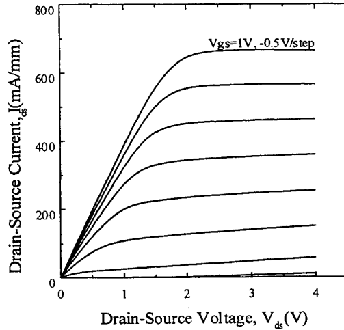
Device I_{ds} - V_{ds} characteristics of D-DCFETs with A gate-length of 1.0\mu m
