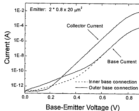
Fig. 3. Gummel plot for a pinched base device measured by contacting either the inner or outer base contacts.
