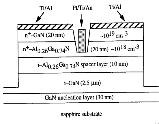
Fig. 1. Cross-sectional structure of recessed gate \text{Al}_{0.26}\text{Ga}_{0.74}\text{N}/\text{GaN} MODFET grown on sapphire by MOCVD.
