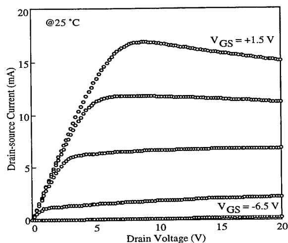
Fig. 3. I_{\text{DS}}-V_{\text{DS}} characteristic of \text{AlGaIn}/\text{GaN} MODFET at 25 °C. The gate length and width are 1.5 and 15 \mu\text{m} , respectively.
