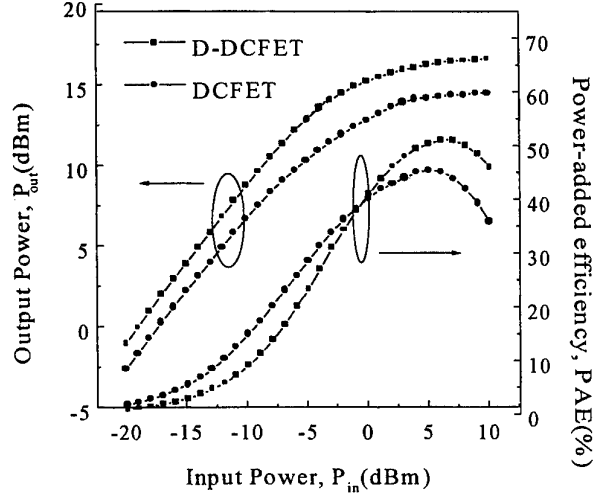
Output power and PAE performances of DCFETs and D-DCFETs (gate width: 150\mu m )
