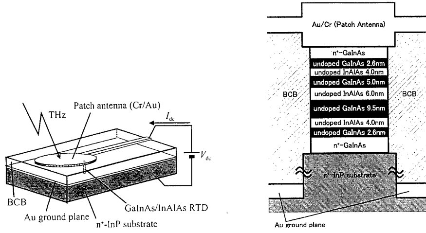
Fig.1 (a)RTD intergrated with a THz patch antenna used for the measurement of photon-assisted tunneling. (b)Cross-section of the diode buried benzo-cyclo-butane(BCB) layer of the antenna.
