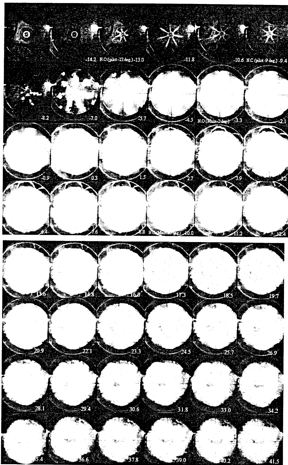
Figure A11. Combustion images (CASE with Multiple Stage Injection ) Test condition: 1000 rpm, 20 degree BTDC injection timing, 0.8 / 0.6 / 2.25 ms injection duration, 80 C/ 1.6 bar inlet air, 620 mini-sac nozzle tip, 12" rate shaping pipe
