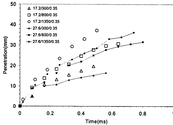
Figure 37 Effect of Injection Pressure and Ambient Pressure on the Spray Penetration of the Common-rail System, with Duration of 0.35 ms, Ambient Pressures of 17.2 and 27.6 bar, and Injection Pressures of 300, 800, and 1350 bar
