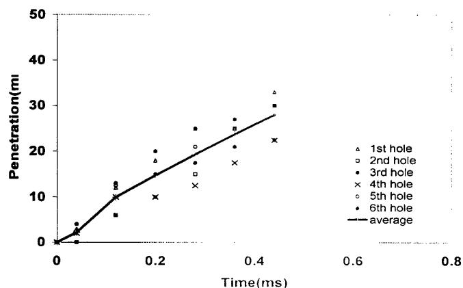
Figure 26 Hole-to-hole penetration variation of the HEUI sprays, with 610 VCO nozzle. pressure of 126 MPa, duration of 2.25 ms, and ambient pressure of 27.6 bar.
