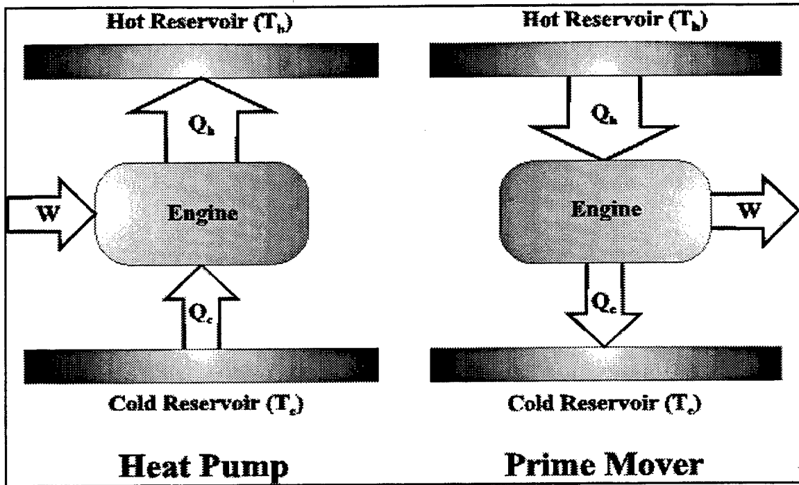
Figure 2.1. Heat Engine Operation
