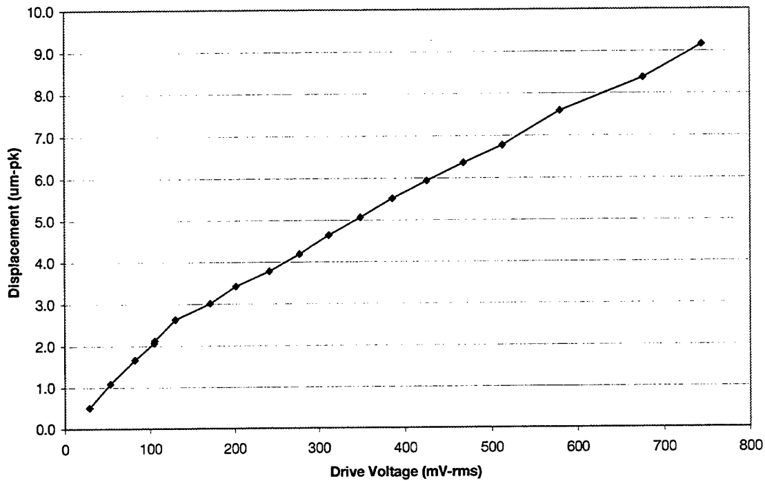
Driving Voltage vs Displacement
