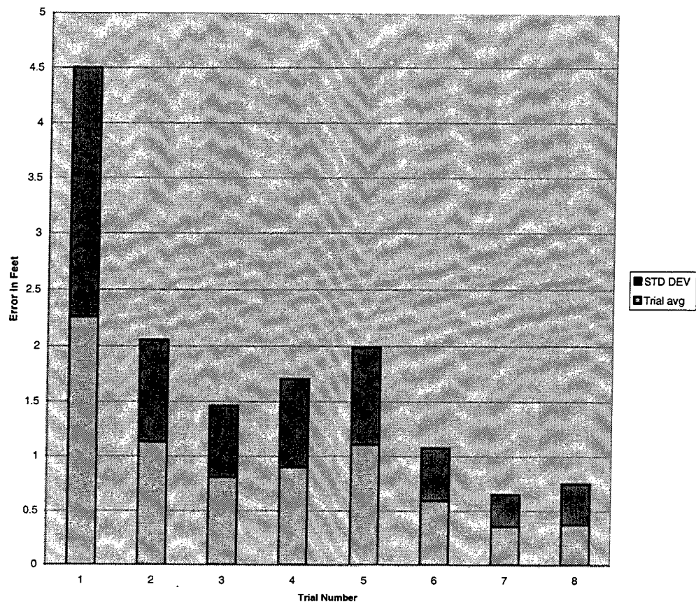
Figure 13. Average Error Versus Trial Number
