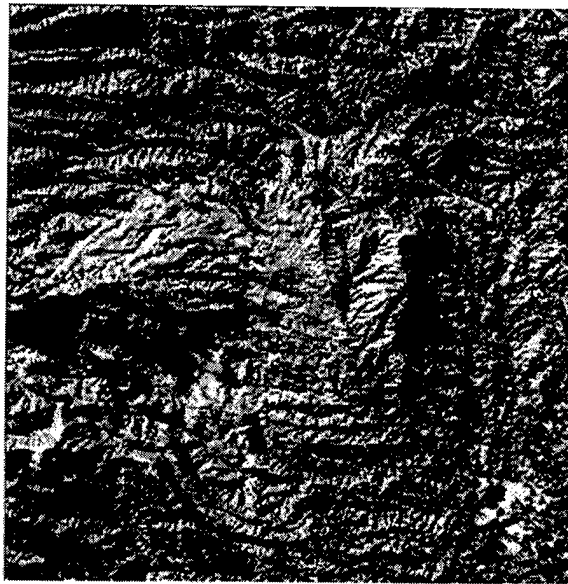
Figure 27. Rendered hillshading.
