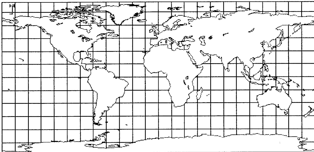
Figure 9. Geographic Projection. From: Picture Gallery of Map Projections, Havlicek, 2000
