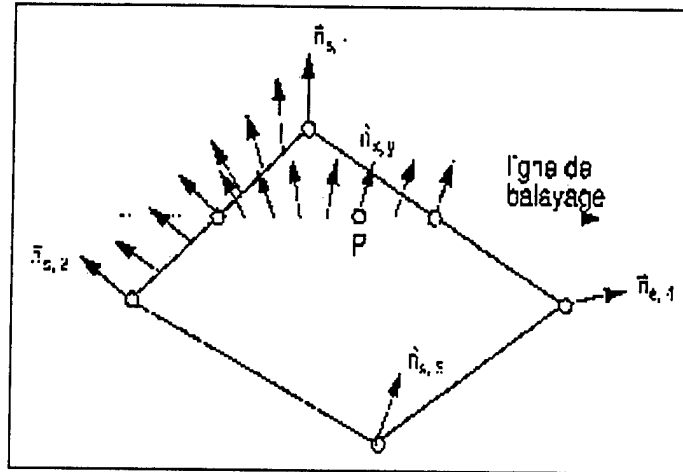
Figure 6. Phong Shading
