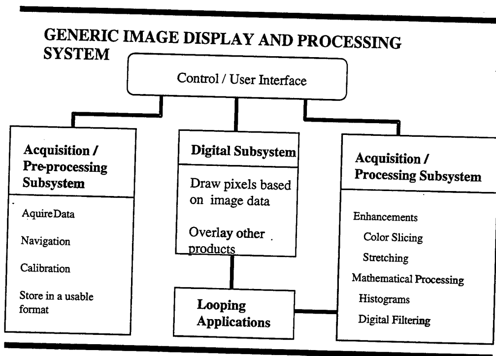
Figure 2. Components of a generic image display and processing system From: Green, 1983
