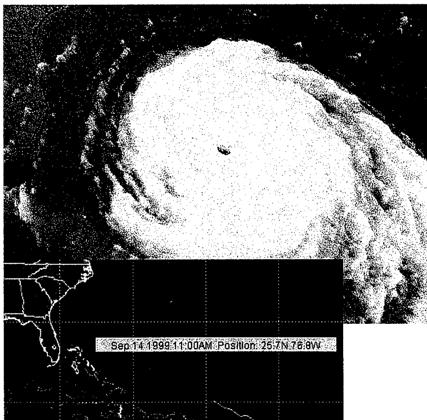
Figure 3. 3-D vs. 2-D views of Hurricane Floyd September 1999. From: Storm Track System and Earth Watch, 2000.
