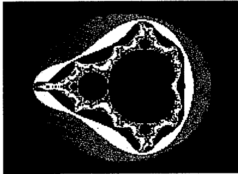
Figure 4. An Example of a Mandelbrot Fractal
