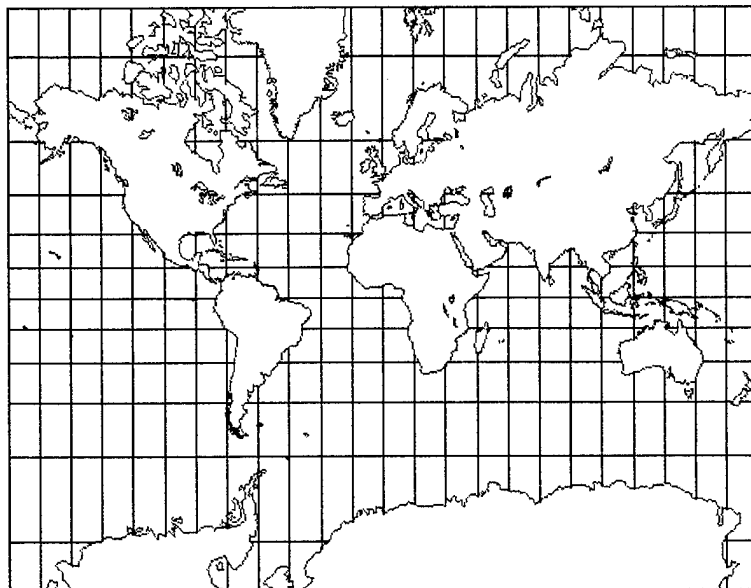
Figure 8. Mercator Projection. Source: Picture Gallery of Map Projections, Havlicek, 2000
