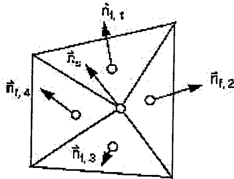
Figure 5. Gouraud Shading
