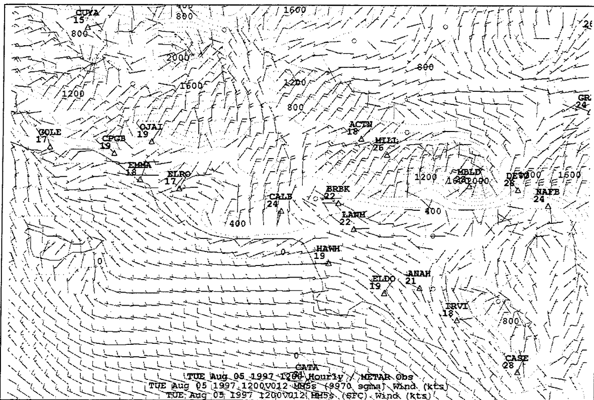
Figure 48 051200Z August MM5 3 kilometer domain winds and SCOS observations.
