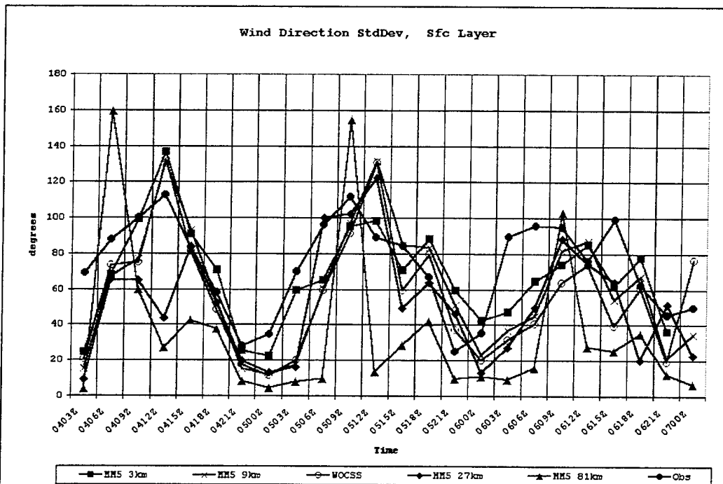
Figure 72. Surface layer wind direction standard deviation time series.
