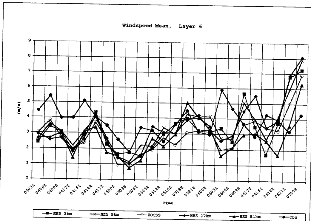
Figure 70. Layer 6 wind speed mean time series.
