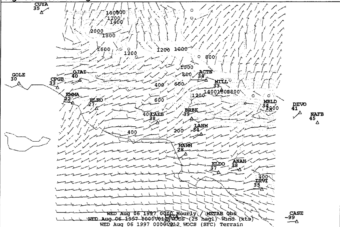
Figure 53 060000Z August WOCSS winds and SCOS observations.
