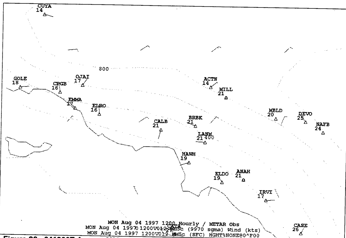
Figure 38. 041200Z August MM5 27 kilometer domain winds and SCOS observations.
