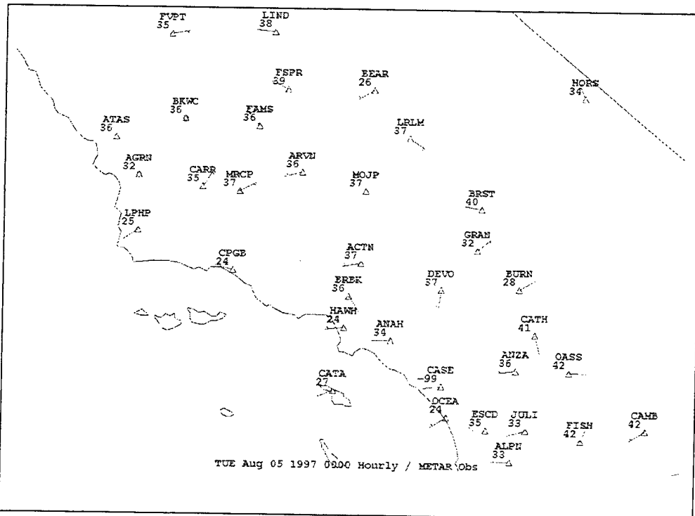
Figure 30. 050000Z August Surface Observations.
