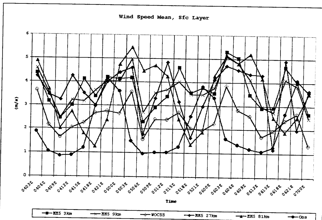
Figure 62. Surface layer wind speed mean time series.
