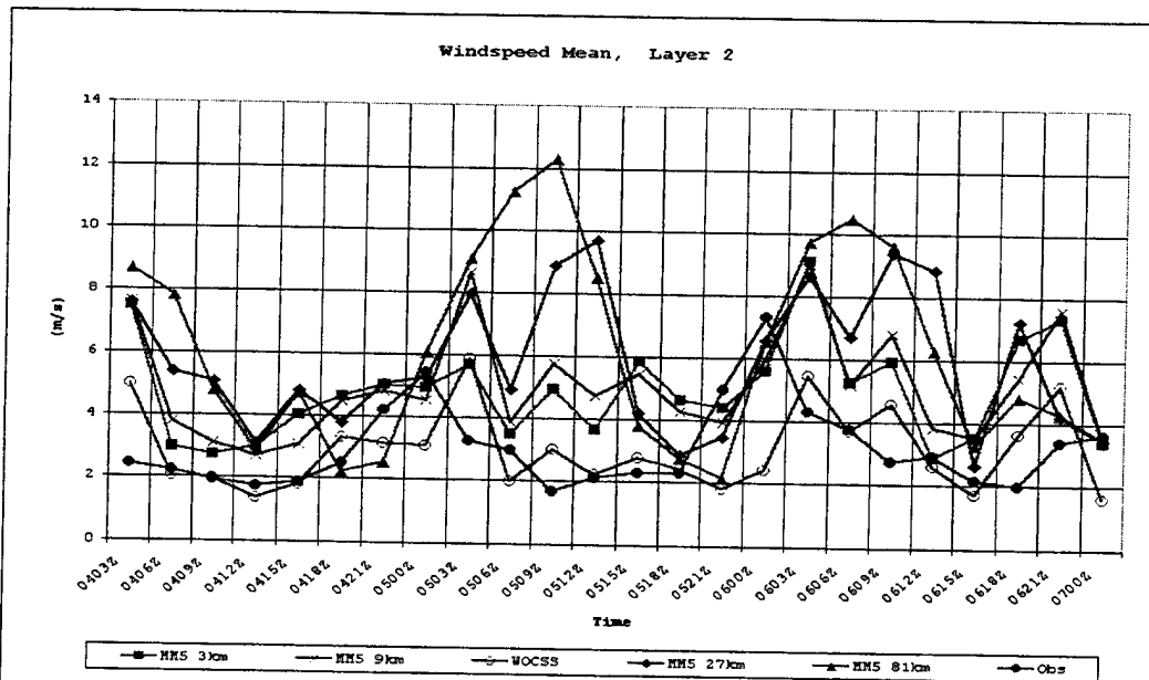
Figure 66. Layer 2 wind speed mean time series.
