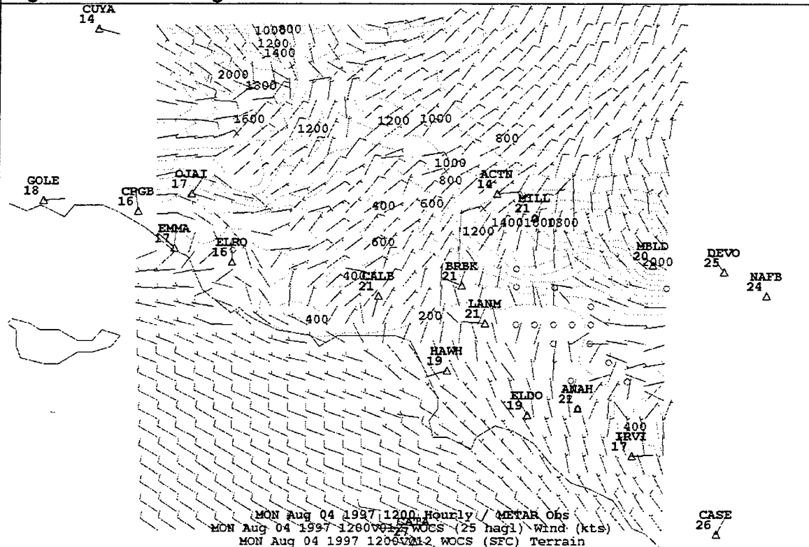
Figure 41. 041200Z August WOCSS winds and SCOS observations.
