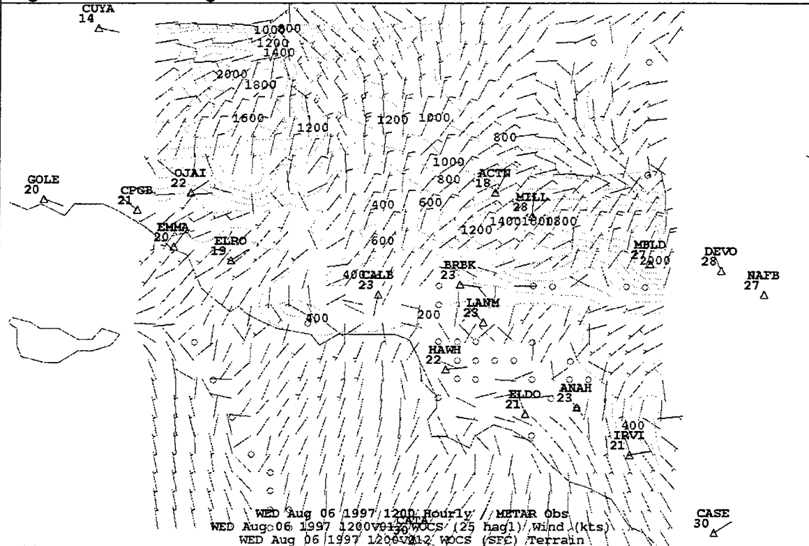
Figure 57 061200Z August WOCSS winds and SCOS observations.
