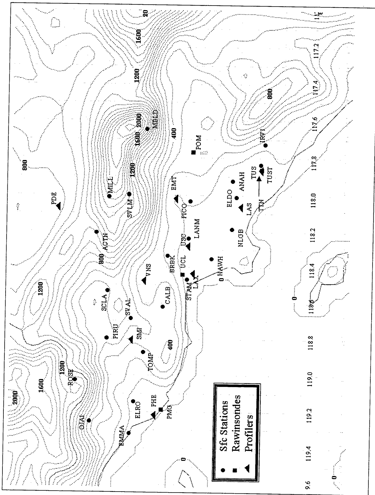
Figure 3. Area of study observation stations and 3 kilometer grid spacing terrain.
