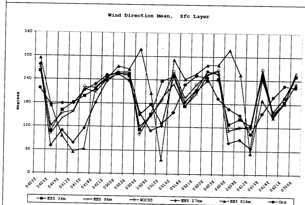
Figure 71. Surface layer wind direction mean time series.
