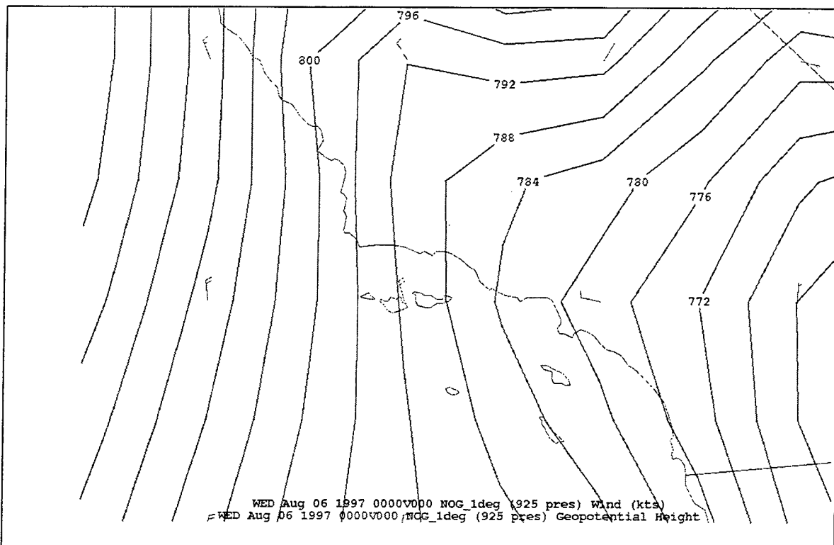
Figure 86. 06000Z August 97 925 mb geopotential heights and winds (NOGAPS 1°).
