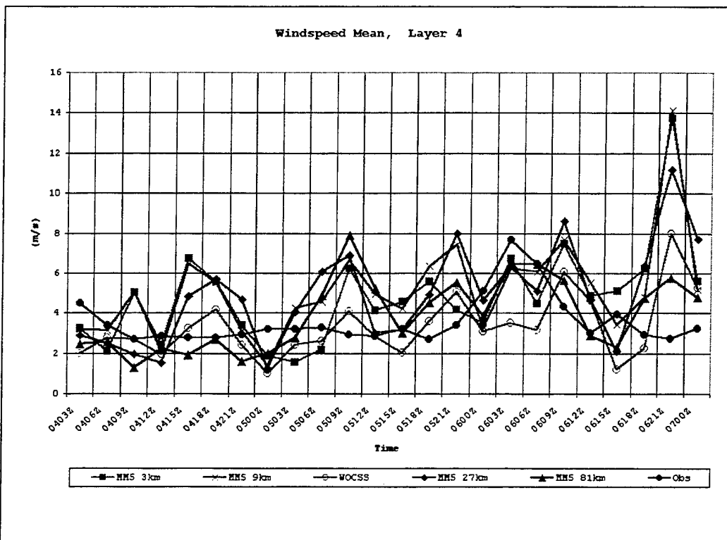
Figure 68. Layer 4 wind speed mean time series.
