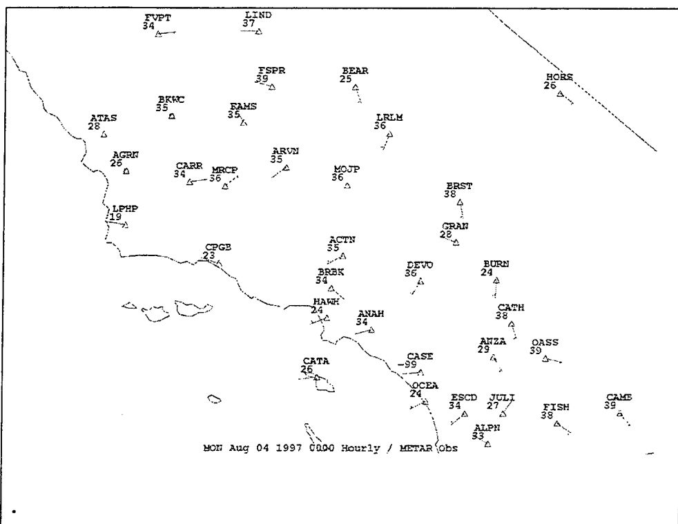
Figure 28. 040000Z August Surface Observations.
