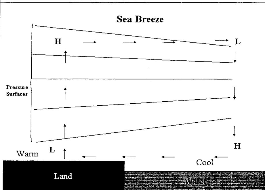
Figure 6b. Schematic of sea breeze circulation.
