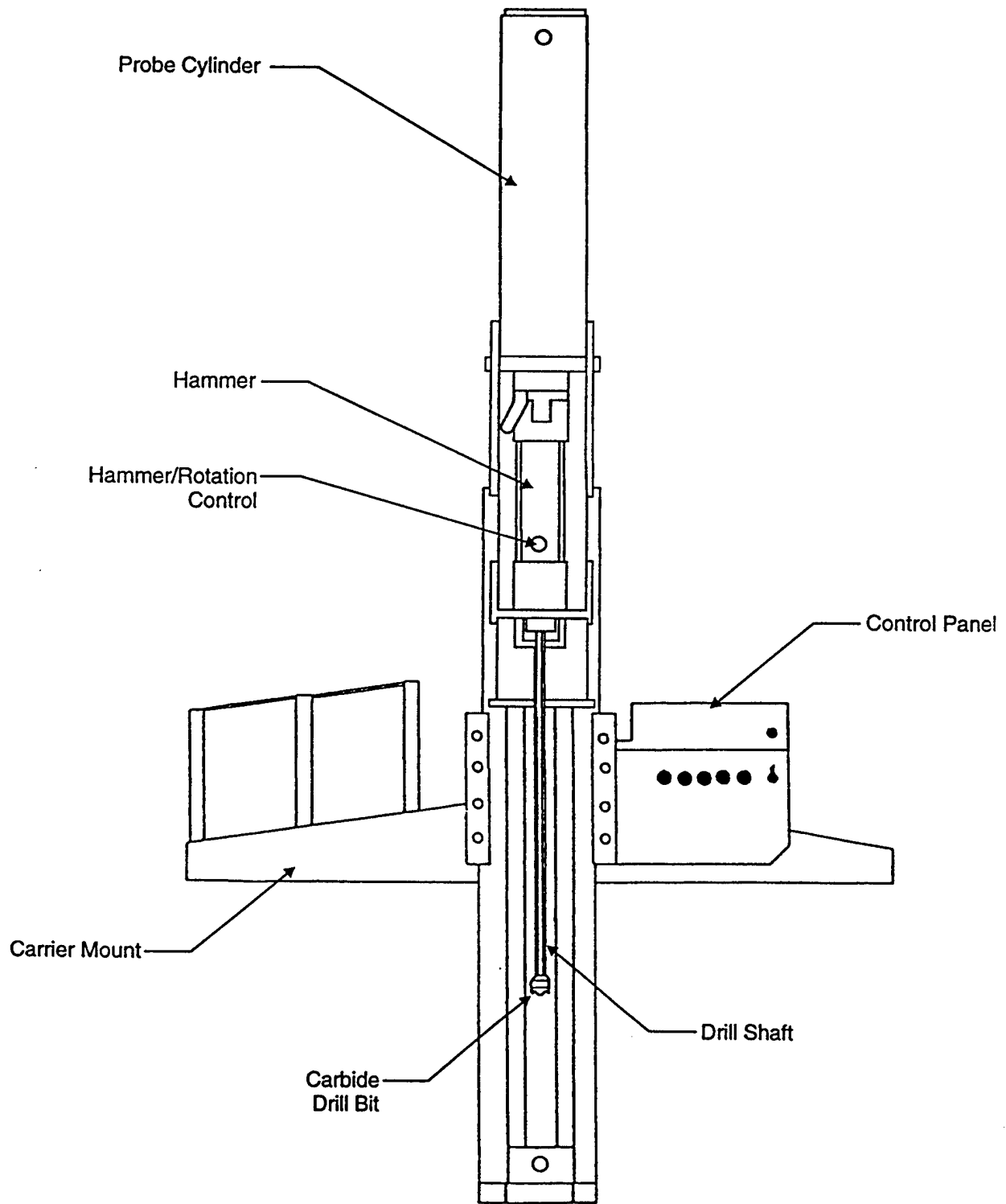
FIGURE 3.1 CROSS-SECTION OF GEOPROBE®
