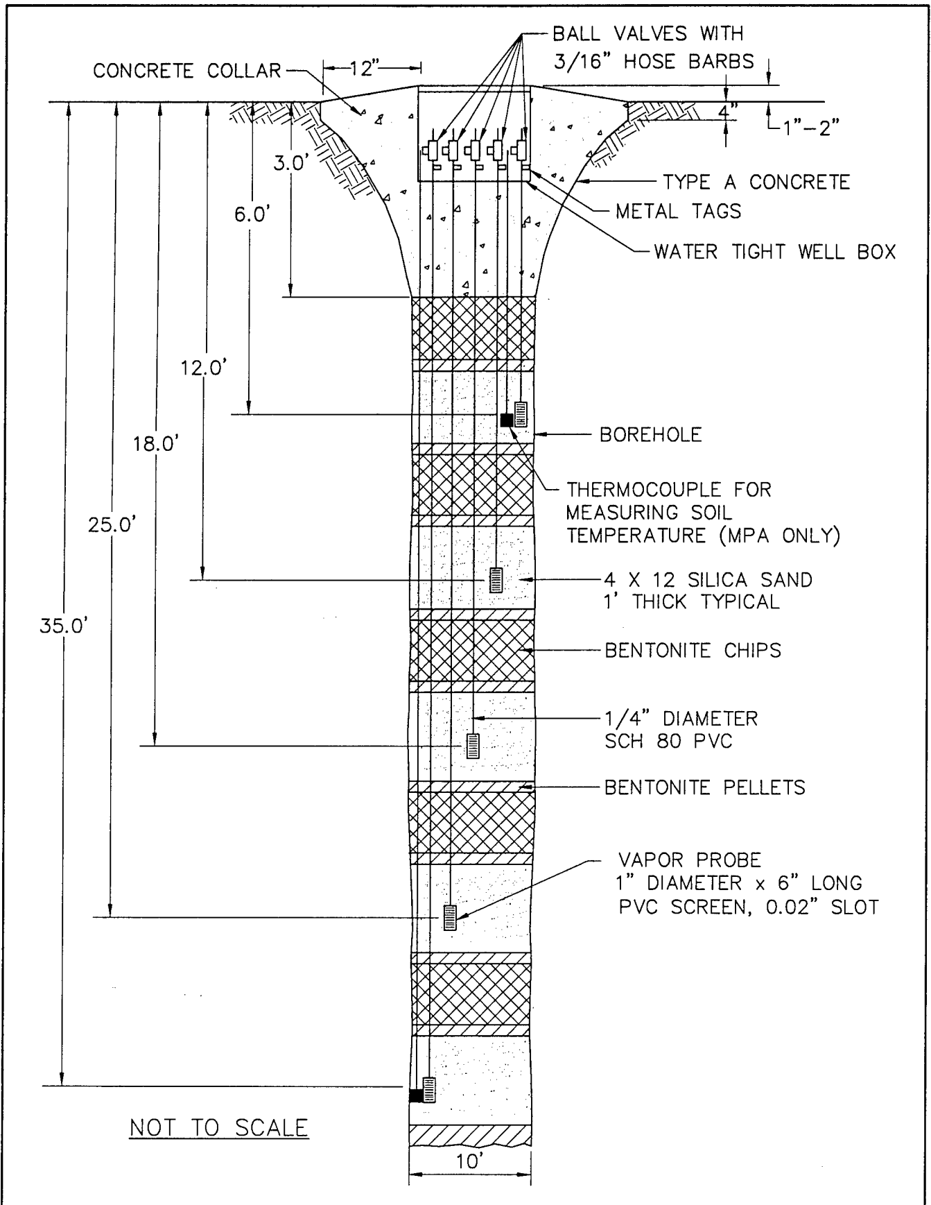
FIGURE 3.3 PROPOSED MONITORING POINT CONSTRUCTION DETAIL SITE 13115 - HEATING OIL UST MCB CAMP PENDLETON, CALIFORNIA
