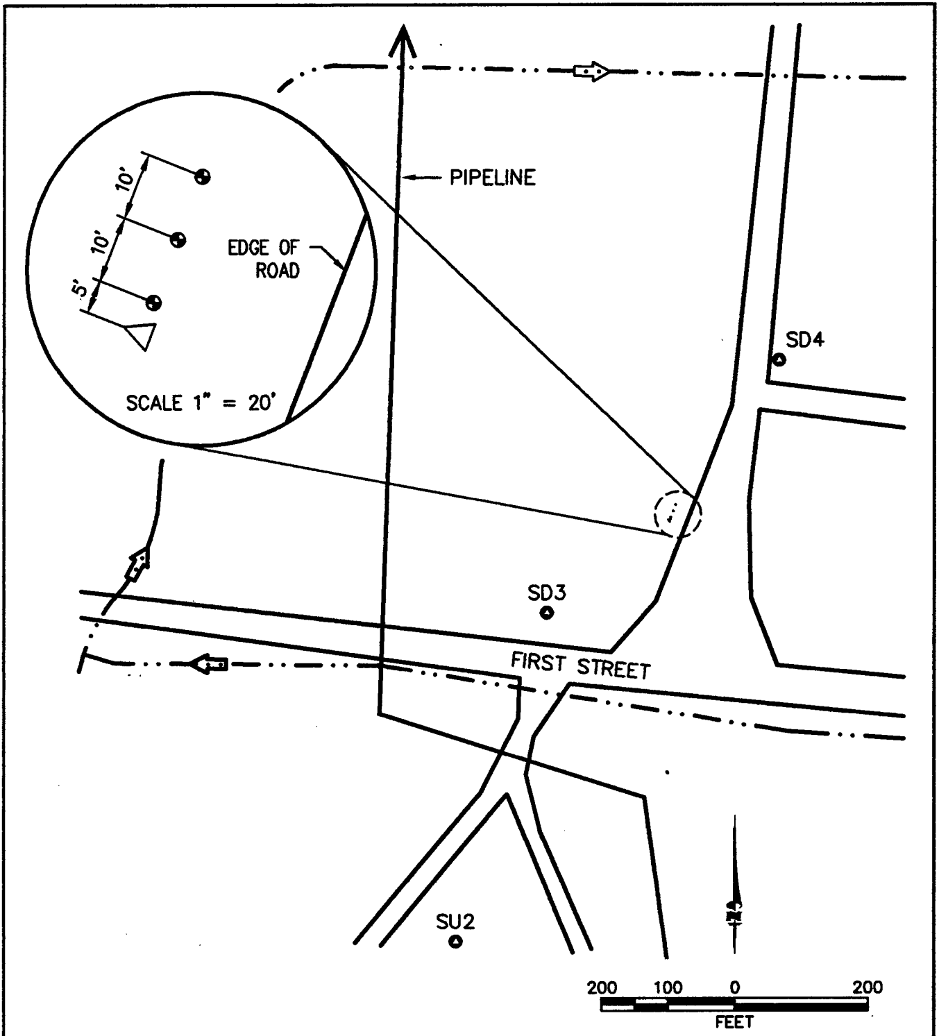
FIGURE 3.4 SITE SS-18 PROPOSED VENT WELL/ MONITORING POINT LOCATIONS LITTLE ROCK AFB, ARKANSAS ENGINEERING-SCIENCE, INC. Denver, Colorado ES
