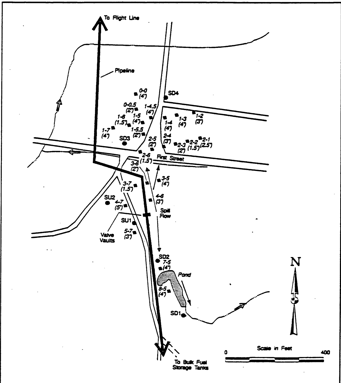
FIGURE 2.3 SITE SS-18 SOIL GAS SAMPLE LOCATIONS JET FUEL RELEASE LITTLE ROCK AFB, ARKANSAS ENGINEERING-SCIENCE, INC. Denver, Colorado
