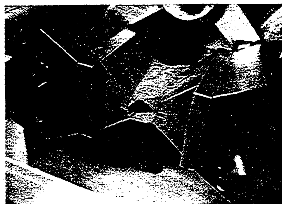
Fig. 2 Photograph of the magnetic abrasive brush formed between the magnetic heads by the magnetic abrasives (Fox et al., 1994)
