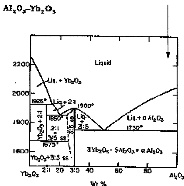
Figure 1 Phase diagram of Al 2 O 3 -Yb 2 O 3 . The arrow indicates the composition of ytterbia-sapphire SELP is close to alumina end [4].
