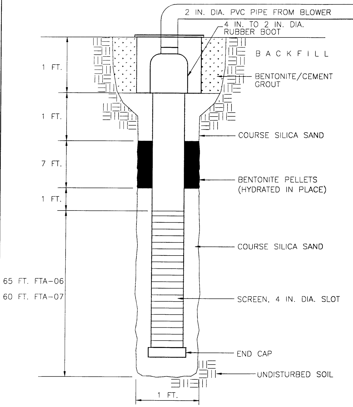
FIGURE 1.1 INJECTION VENTING WELL CONSTRUCTION DETAIL FTA-06 & FTA-07 K.I. SWAYER AFB, MICHIGAN ENGINEERING-SCIENCE, INC. Syracuse, New York ES
