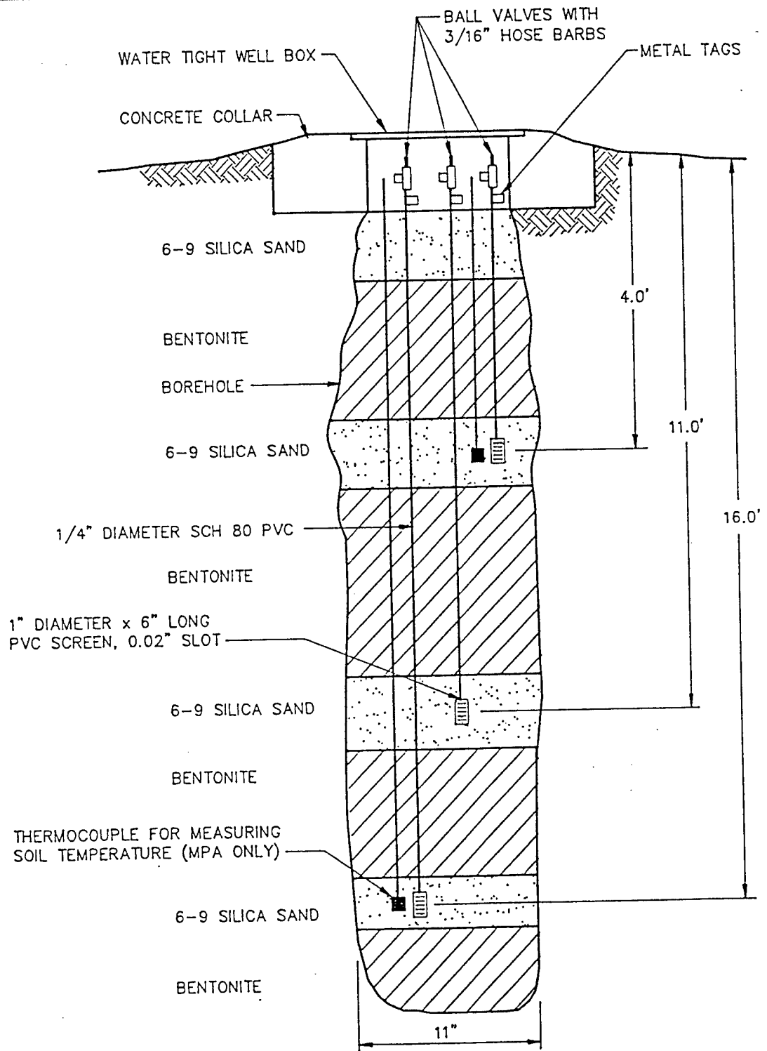
FIGURE 3.6 SITE FC-2 MONITORING POINT CONSTRUCTION DETAIL
