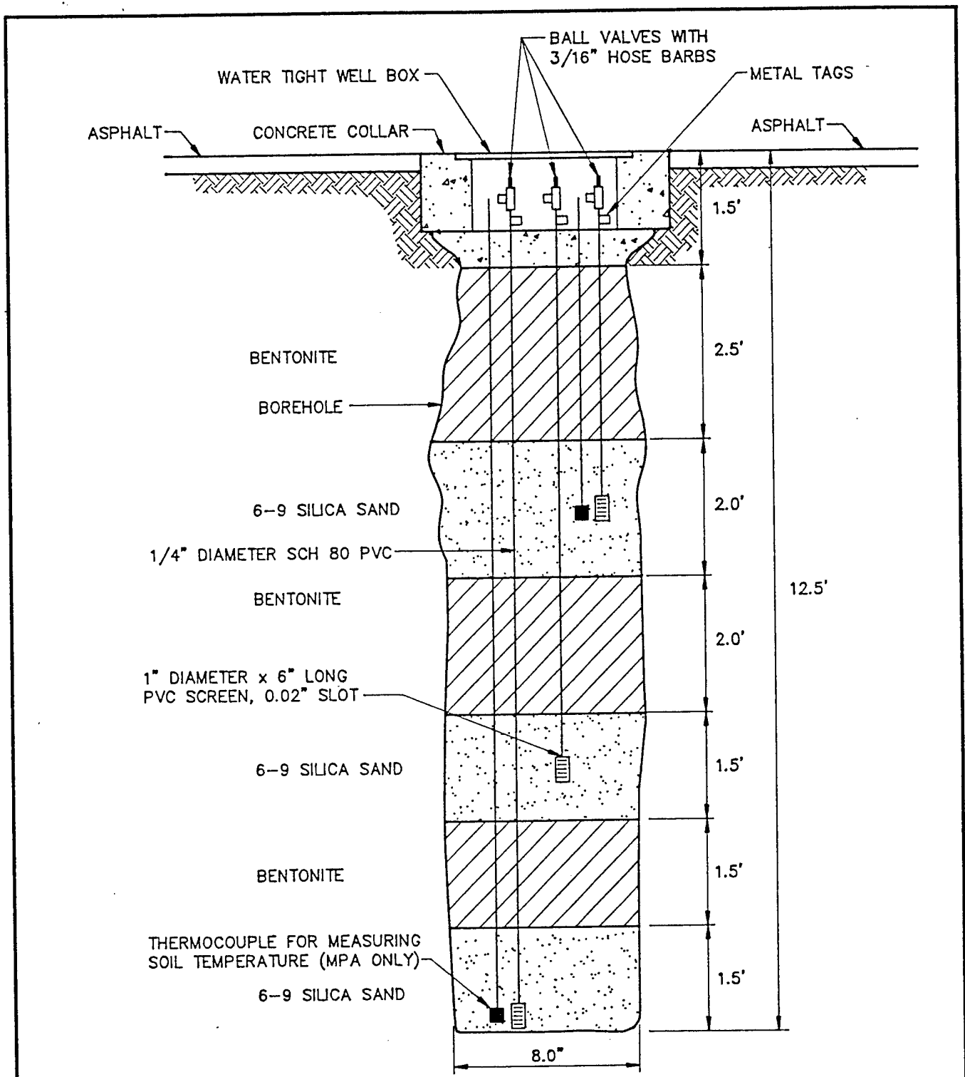
FIGURE 1.4 SITE S-4 AS-BUILT MONITORING POINT CONSTRUCTION DETAIL KELLY AFB, TEXAS ENGINEERING-SCIENCE, INC. Denver, Colorado
