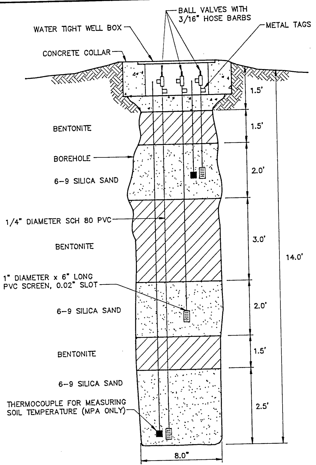
FIGURE 2.4 SITE FC-2 AS-BUILT MONITORING POINT CONSTRUCTION DETAIL KELLY AFB, TEXAS ENGINEERING-SCIENCE, INC. Denver, Colorado
