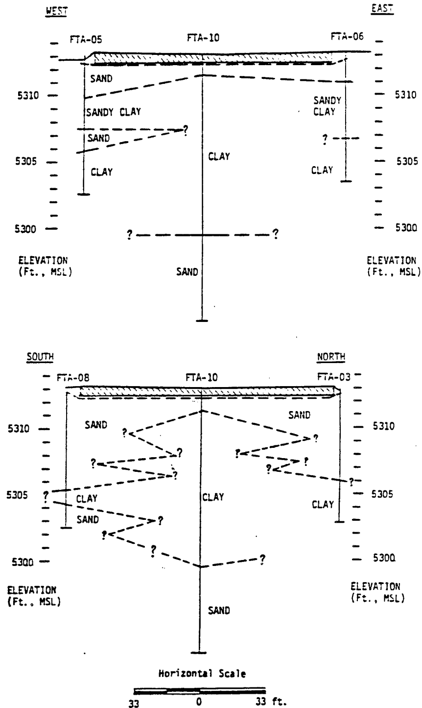
FIGURE 2.3 GEOLOGIC CROSS SECTION FORMER FIRE TRAINING AREA
