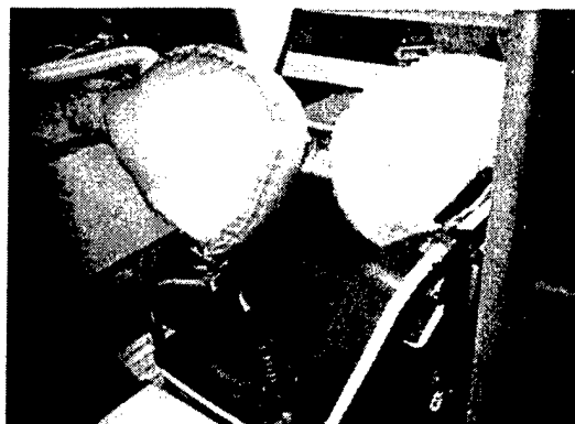
Figure 8: Airbags Installed in 9D5 Dunker Cockpit
