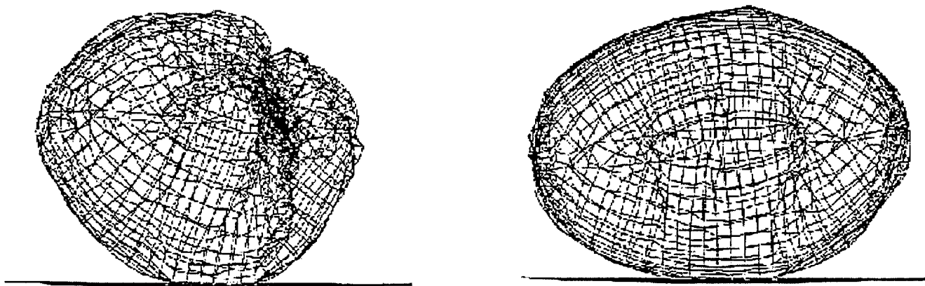
Figure 2. Sequential display of the airbag-sphere interaction with direct rotational impact. Linear velocity = 15 m/s and angular velocity = 15 rad/s
