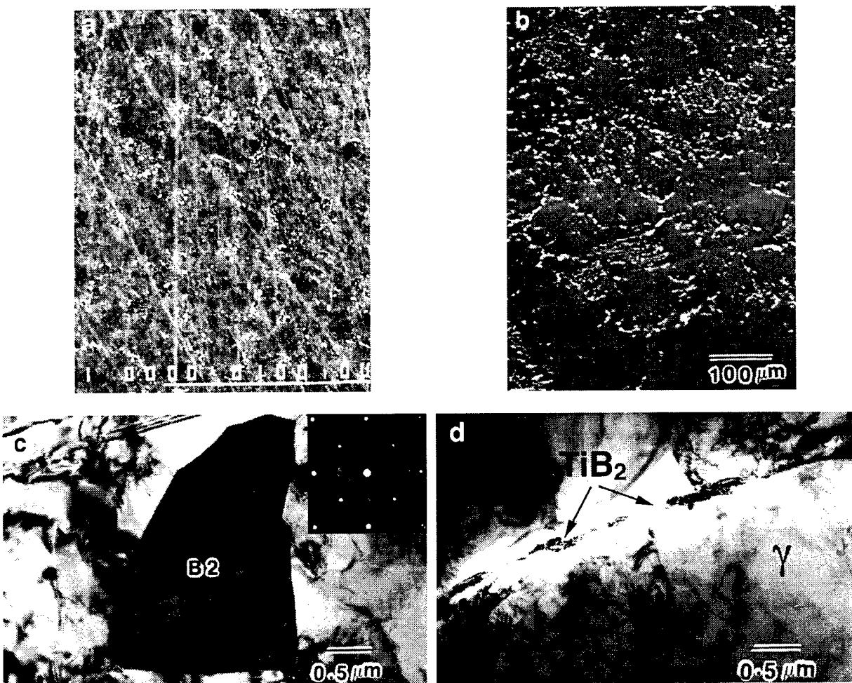
Figure 10. Microstructure of as-forged alloys. (a) 0.0B, BSEI; (b) 0.2B, BSEI; (c) 0.0B, TEM micrograph showing B2 particles with equiaxed \gamma grains (inset [001] B2 SAD pattern); and (d) 0.2B, TEM micrograph showing borides at \gamma grain boundaries.
