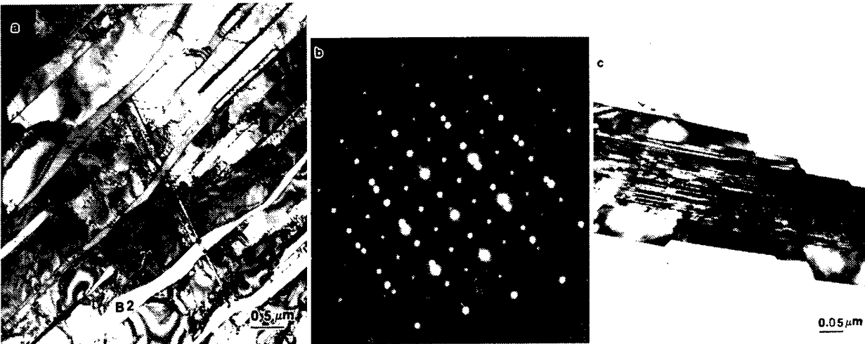
Figure 9. As-cast microstructure of 0.2B alloy. (a) TEM micrograph showing B2 cores with \gamma - \alpha_2 lamellae; (b) [111] B_2 // [011] \gamma // [11\bar{2}0] \alpha_2 SAD pattern; and (c) TEM micrograph showing boride morphology.
