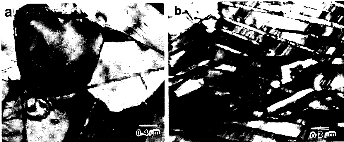
Figure 3. BF TEM micrographs showing microstructure of 37Nb-37Ti-26Al alloy solutionized at 1400°C, 1 h, WQ then aged at (a) 900°C, 1h, WQ and (b) 900°C, 200h, WQ. Fully O.
