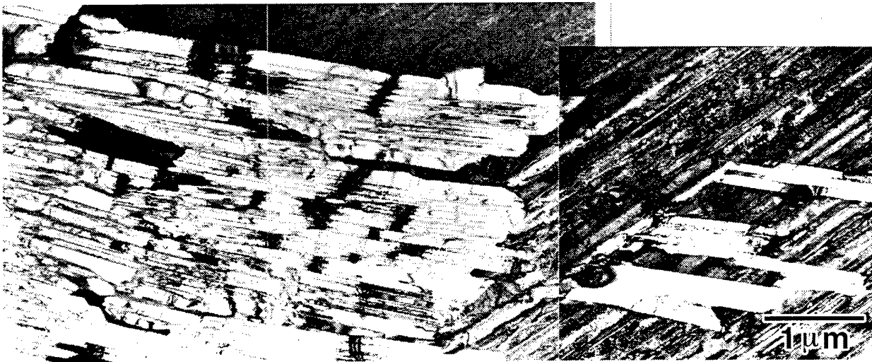
Figure 25. TEM bright-field micrographs of feathery gamma ( \gamma_F ) microconstituent in 45-2-2 alloy (heat treated according to 1320°C/15min. + AC/20sec to 1170°C/WQ). The lamellar \gamma_L front from one grain grows into a neighboring parent alpha grain discontinuously and fans out in the form of the feathery \gamma_F microconstituent.
