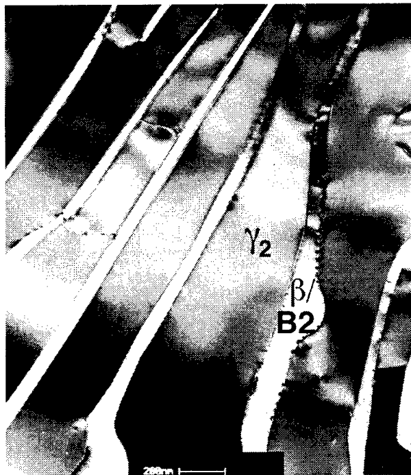
Figure 26. TEM micrographs showing beta decomposition products in the 47-2-2-1 alloy heat treated according to 1370°C/10min. \rightarrow SPQ 1053°C/5sec/WQ. (a) Coarse \gamma precipitates in grain boundary \beta/B2 and (b) cellular \gamma_c + \beta/B2 product.
