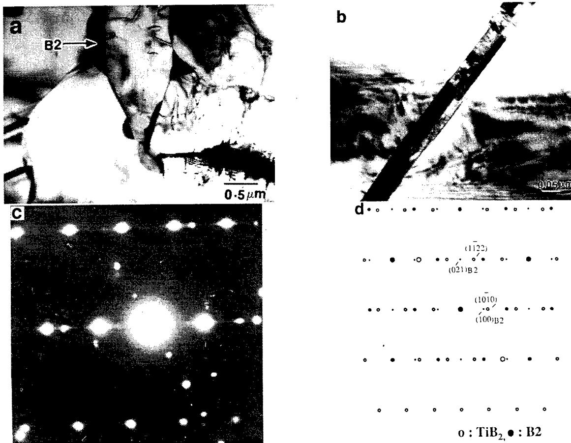
Figure 13. TEM micrographs of 0.2B alloy heat treated at 1400°C/2h/AC. (a) Grain boundary B2 particles; (b) a boride ( TiB_2 ) plate containing thin layers of B2; (c) experimental; (d) simulated [2423]TiB_2 // [012]B_2 SAD pattern from composite boride plate in (b).
