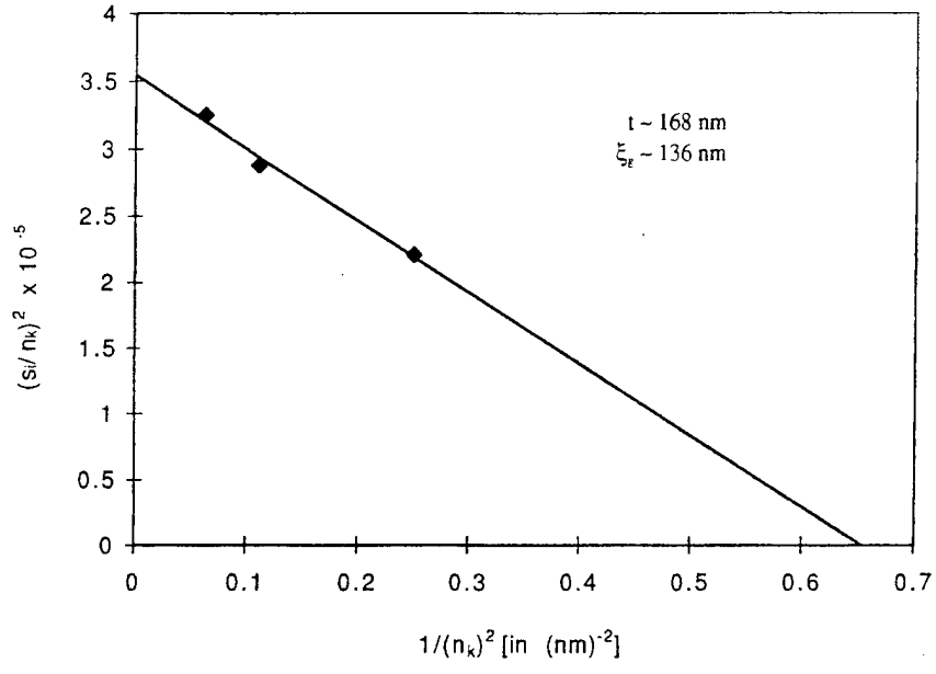
Figure 6. Kossel-Mollenstedt fringes in a ZOLZ CBED pattern from B2 phase in the Nb-37Ti-26Al alloy, quenched from 1200°C after a hold for 200h with (a) (110) strongly excited and (b) a plot of (s_i/n_k)^2 vs. 1/(n_k)^2 ; intercept = 1/r^2 , Slope = 1/(\xi_g)^2 .
