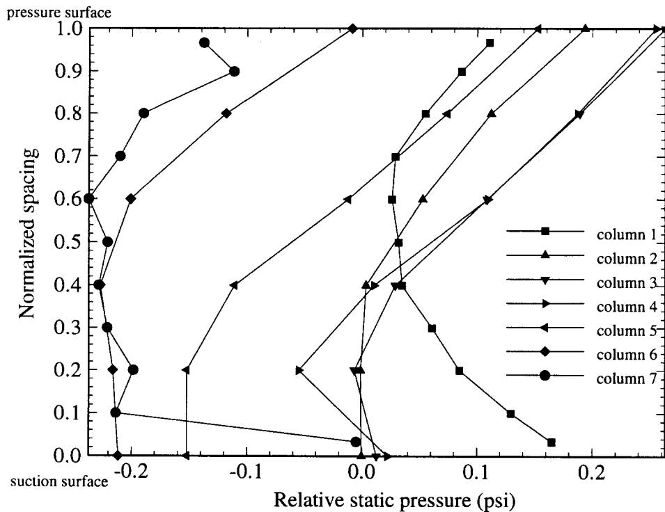
Figure 5.27 Static pressure distribution for each column
