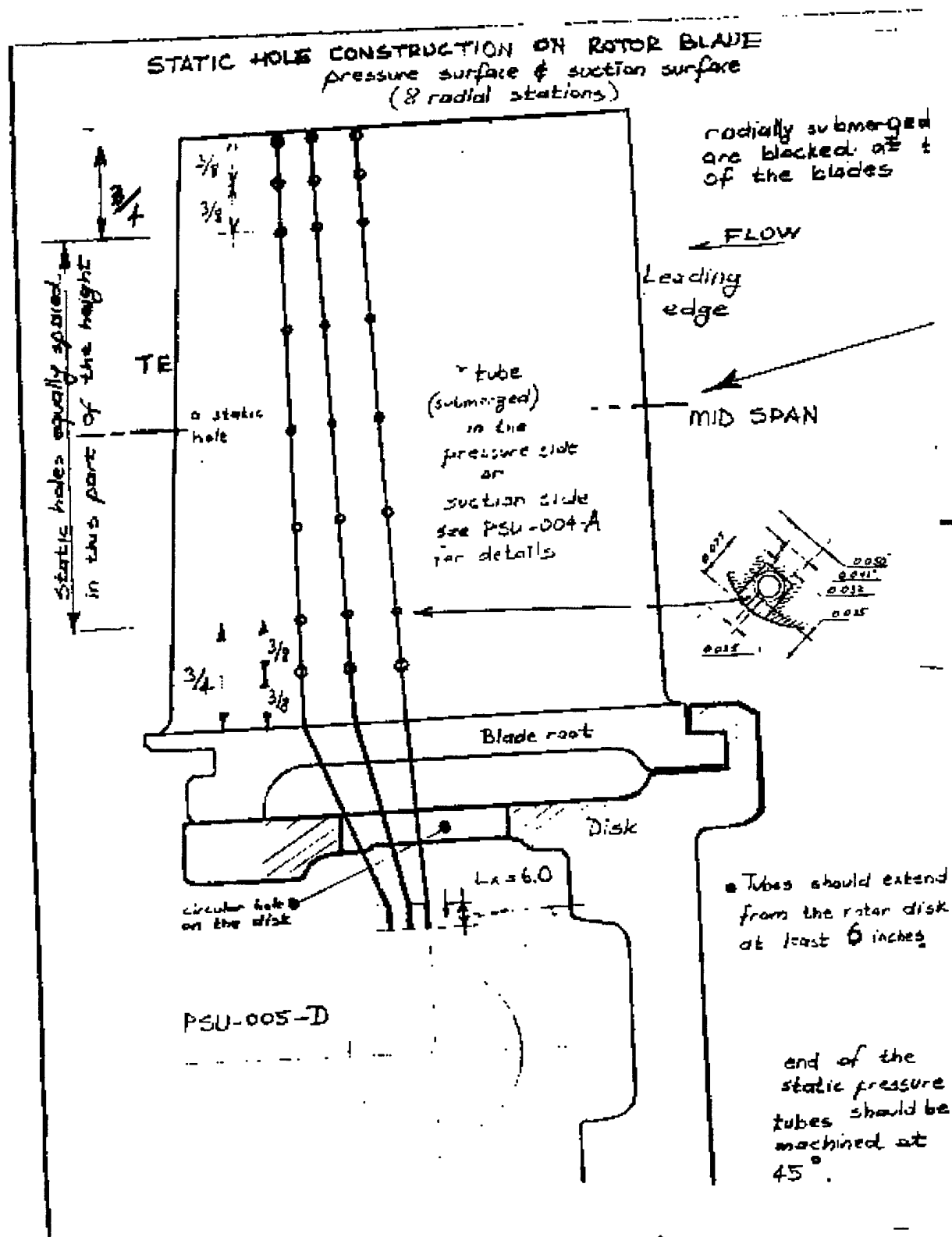
Figure 4.6 static pressure holes location layout 3
